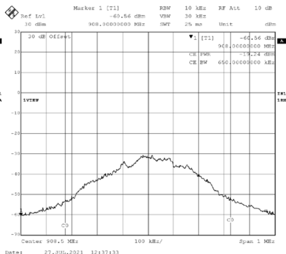
908.5MHz Peak Power (left) and Average Power (right)
