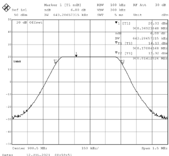
908.5MHz DTS BW (left) and 6dB BW (right)
