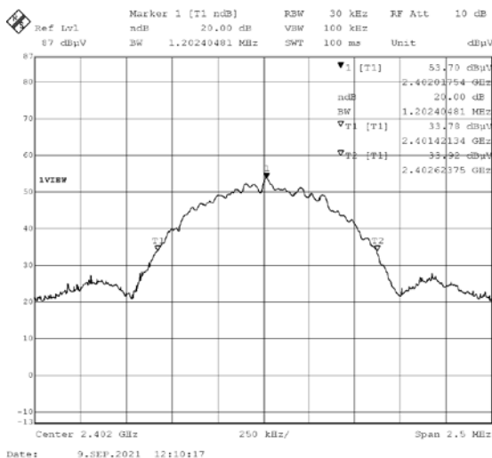
2402MHz 20dB BW (left) and 99% OPB (right)
