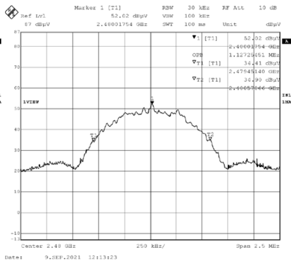
2480MHz 20dB BW (left) and 99% OPB (right)
