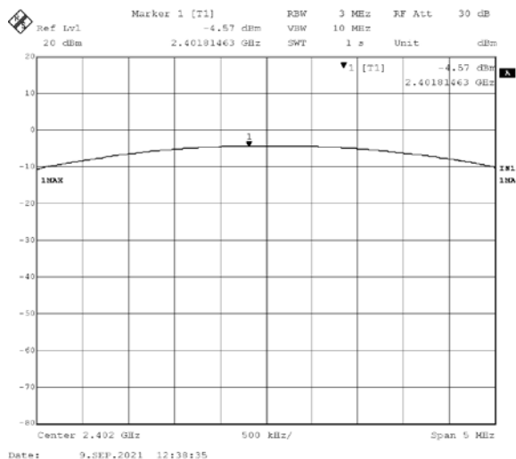
2402MHz Peak Output Power
