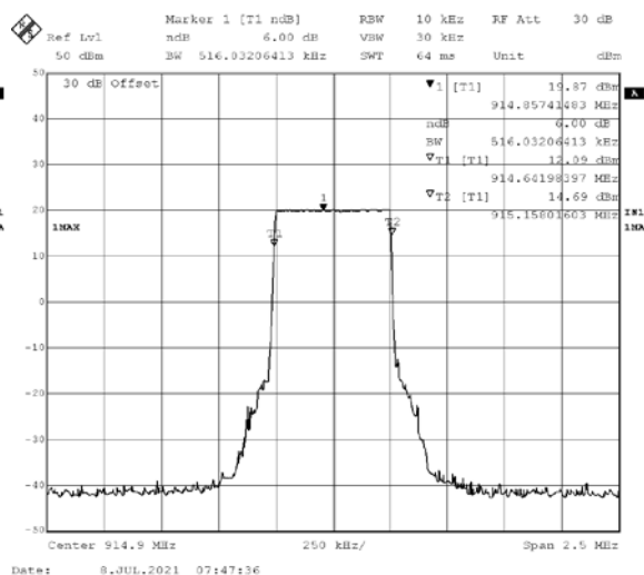
914.9MHz DTS BW (left) and 6dB BW (right)
