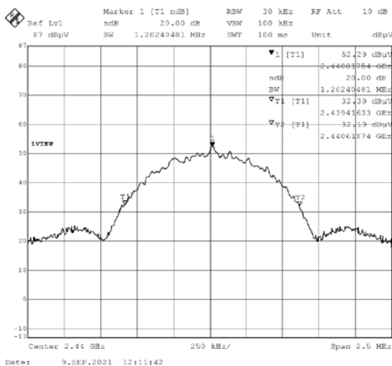
2440MHz 20dB BW (left) and 99% OPB (right)
