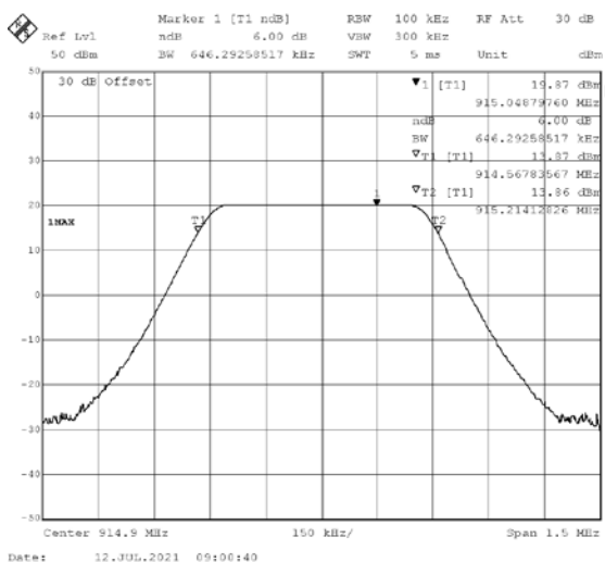
914.9MHz DTS BW (left) and 6dB BW (right)
