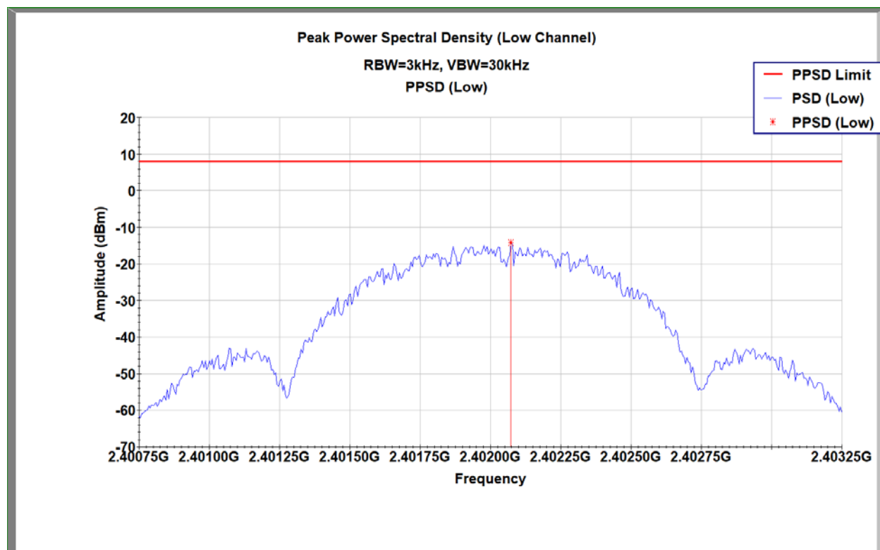
2402MHz Power Spectral Density
