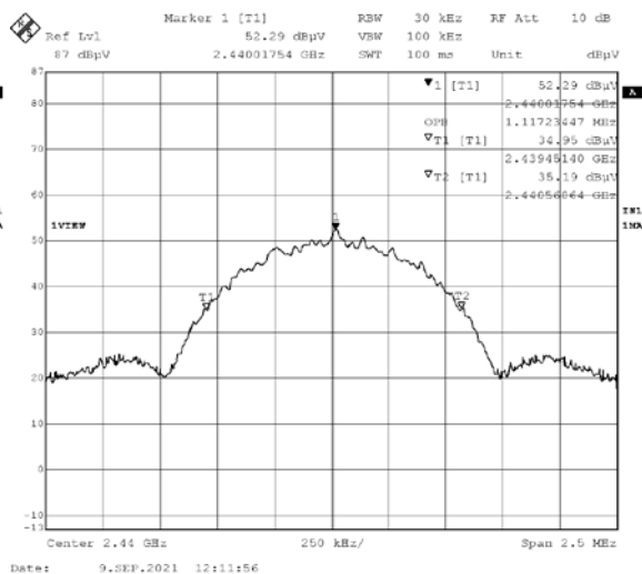
2440MHz 20dB BW (left) and 99% OPB (right)
