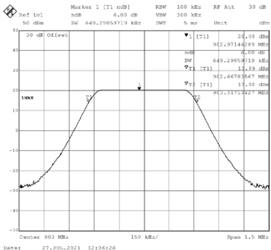
903.0MHz DTS BW (left) and 6dB BW (right)
