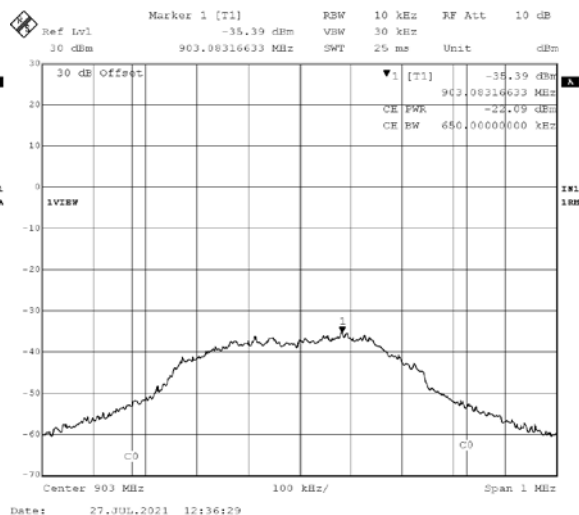
903.0MHz Peak Power (left) and Average Power (right)
