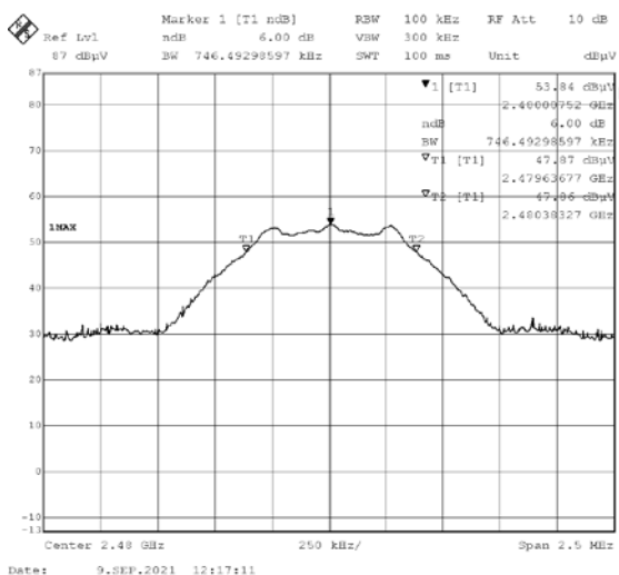
2480MHz DTS BW (left) and 6dB BW (right)
