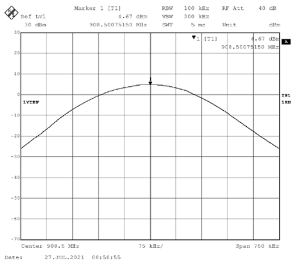
908.5MHz Power Spectral Density
