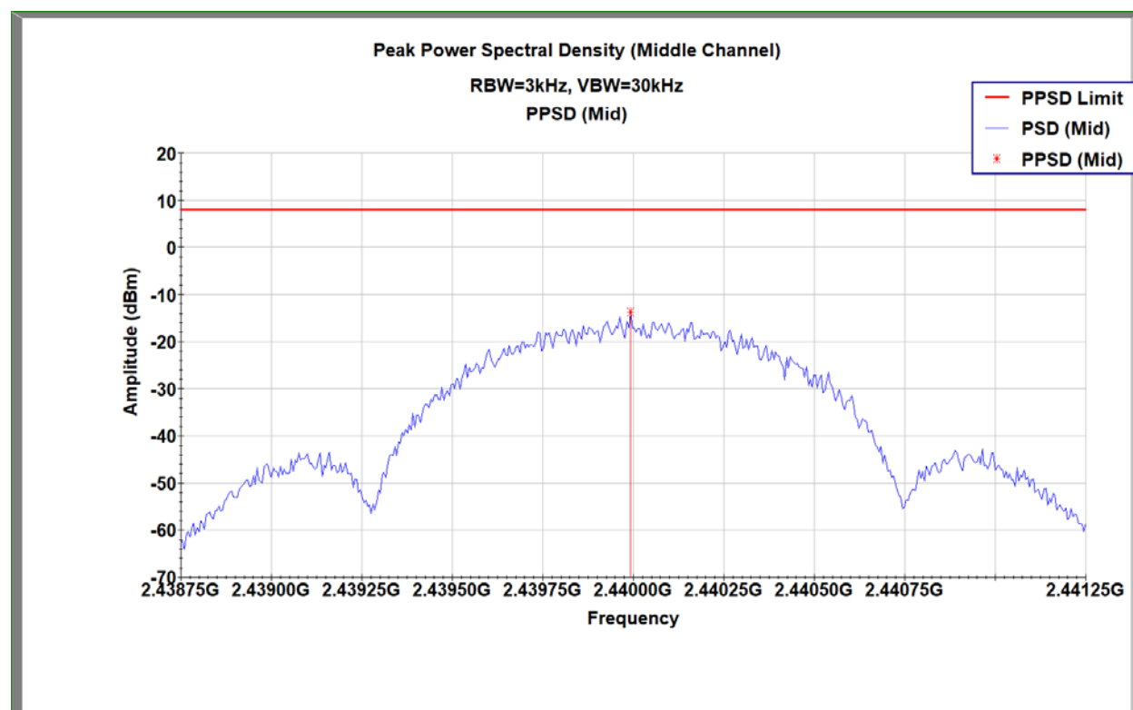
2440MHz Power Spectral Density
