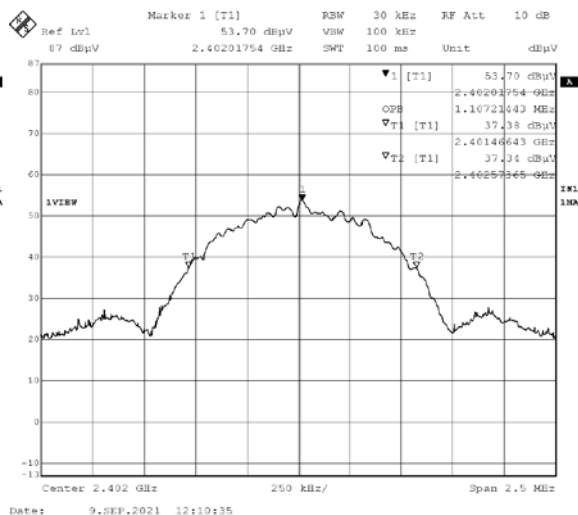
2402MHz 20dB BW (left) and 99% OPB (right)
