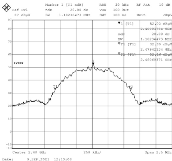
2480MHz 20dB BW (left) and 99% OPB (right)
