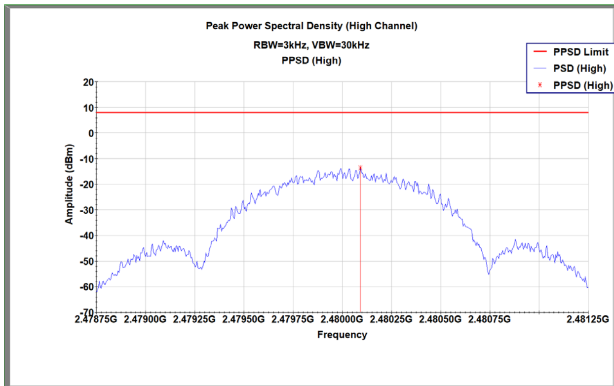
2480MHz Power Spectral Density
