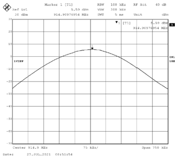
914.9MHz Power Spectral Density
