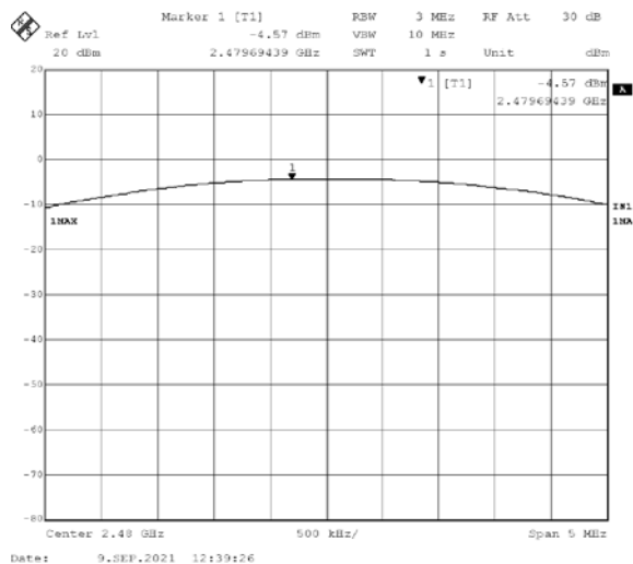
2480MHz Peak Output Power
