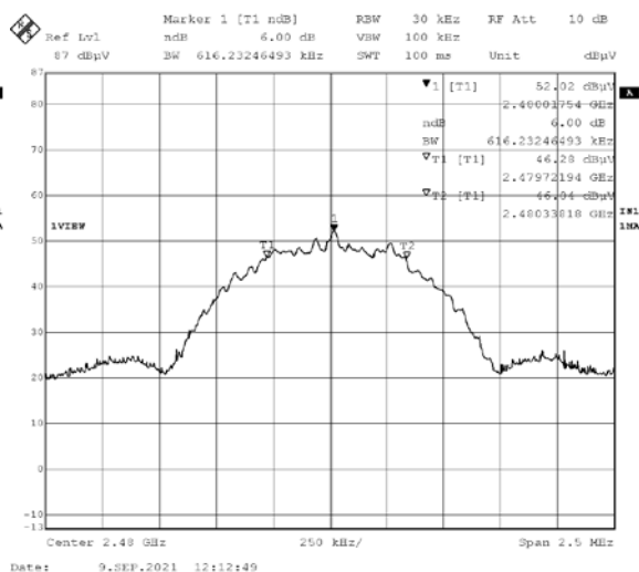
2480MHz DTS BW (left) and 6dB BW (right)
