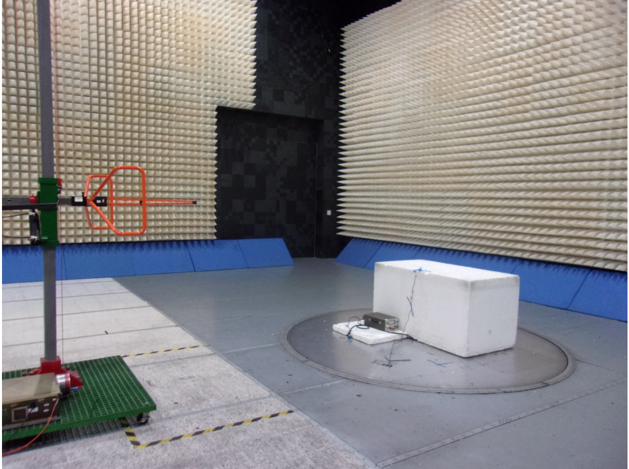
Setup – spurious emissions, 30MHz – 1GHz
