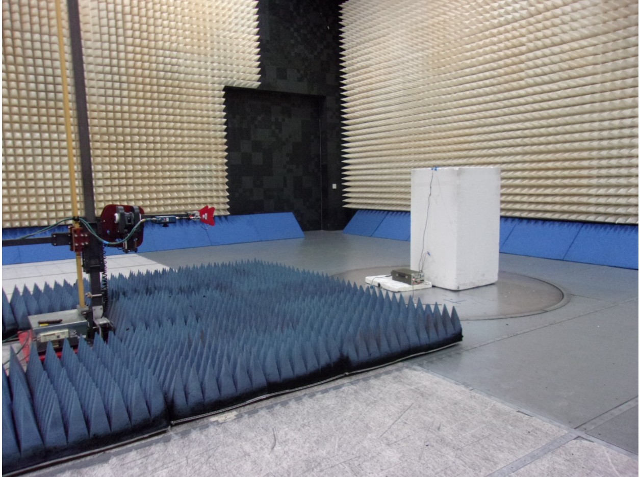
Setup – spurious emissions, 1GHz – 10GHz
