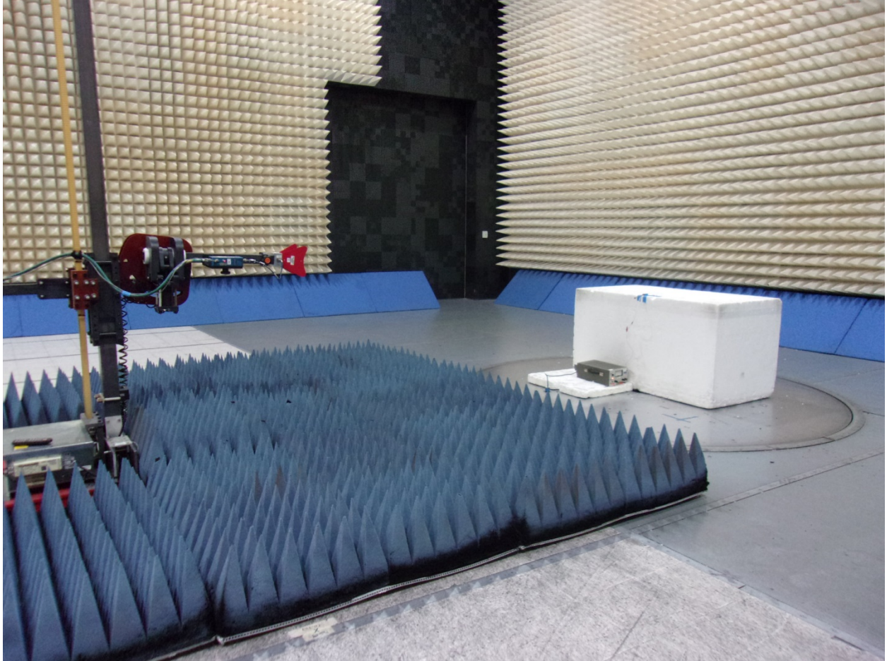
Setup – unintentional emissions, 1GHz – 10GHz
