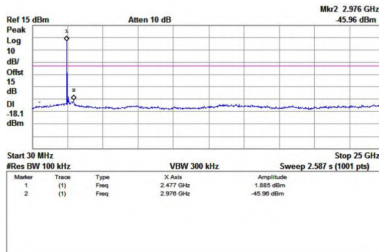
(Plot F.1:Channel = 78, 30MHz to 25GHz @ \pi/4 -DQPSK)
