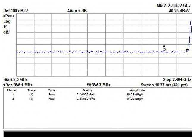
GFSK: Band Edge-Low Channel
