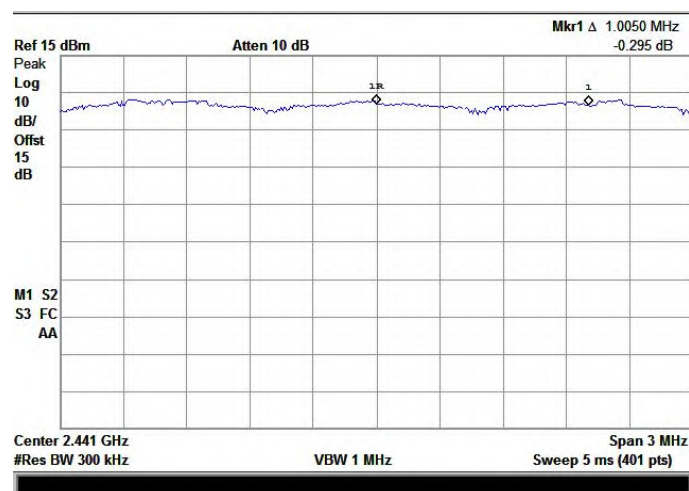
( \pi /4DQPSK) Channel Separation plot
