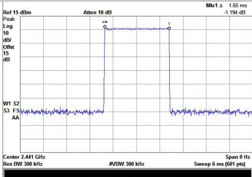
Plot B: DH3
