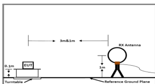
Below 30MHz
