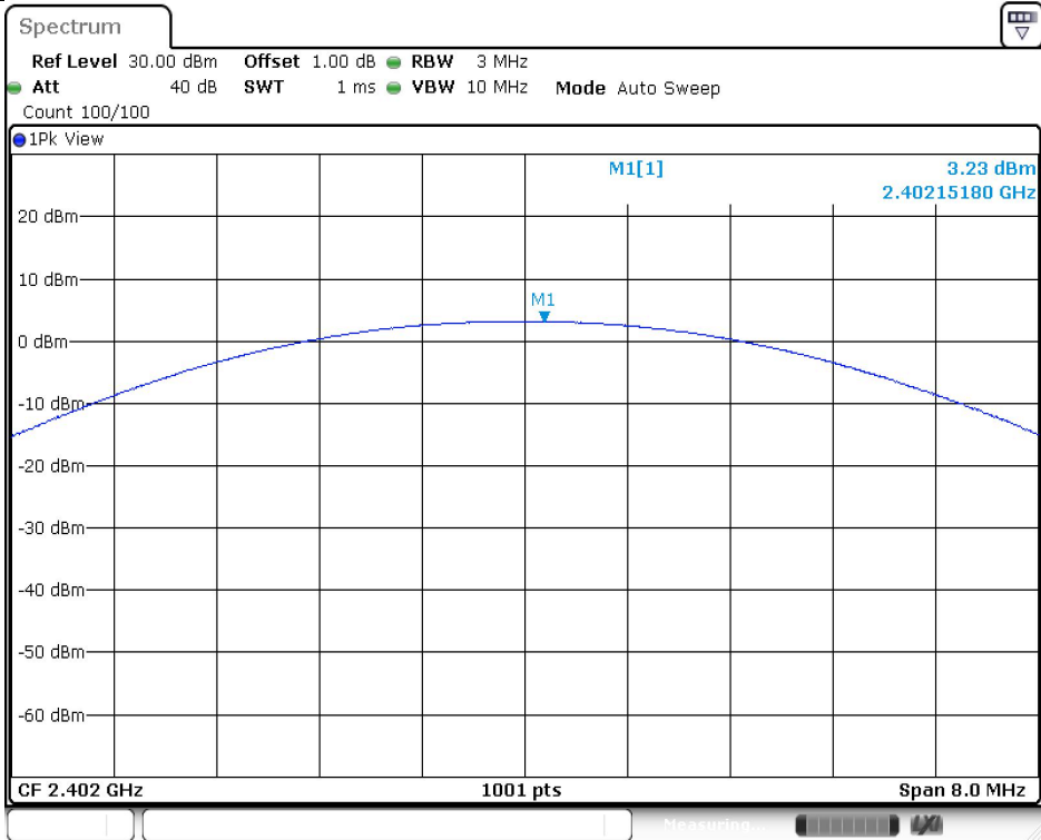
2DH5_Ant1_2402
