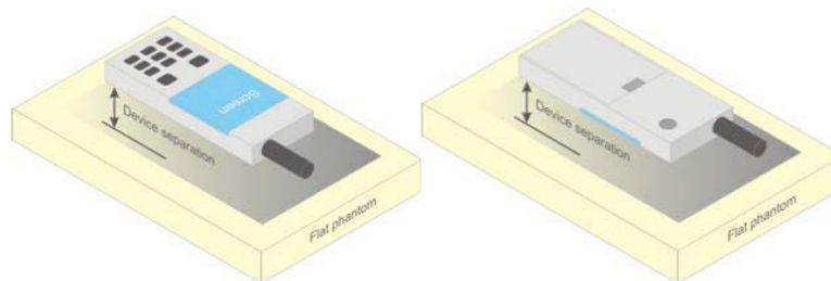
Figure 5 – Test positions for body-worn devices
