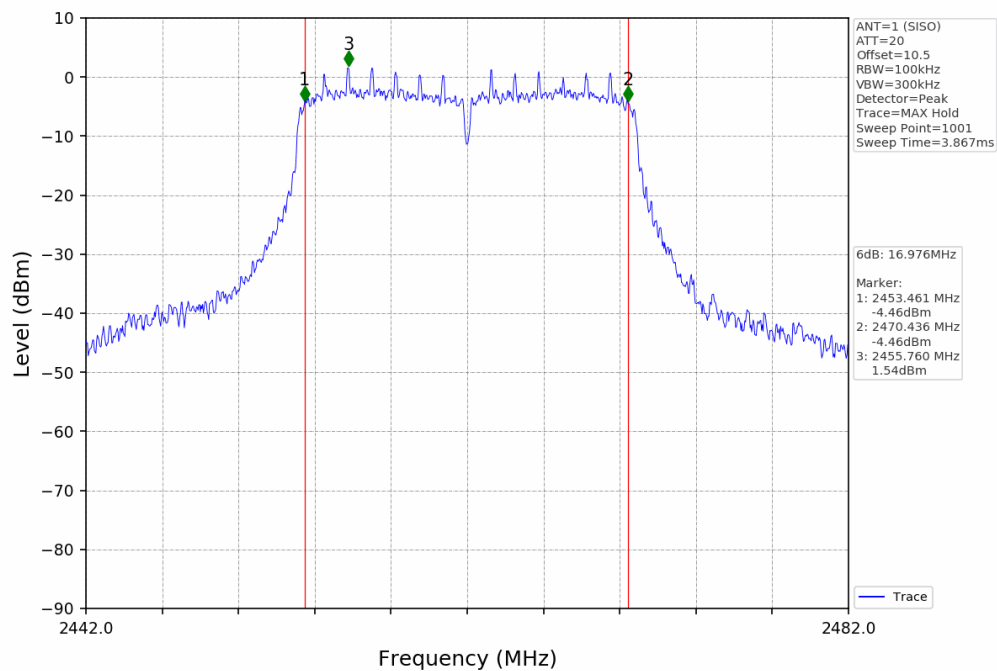
Bandwidth NTNV_802.11n (HT20)_SISO_2462MHz_ANT1
