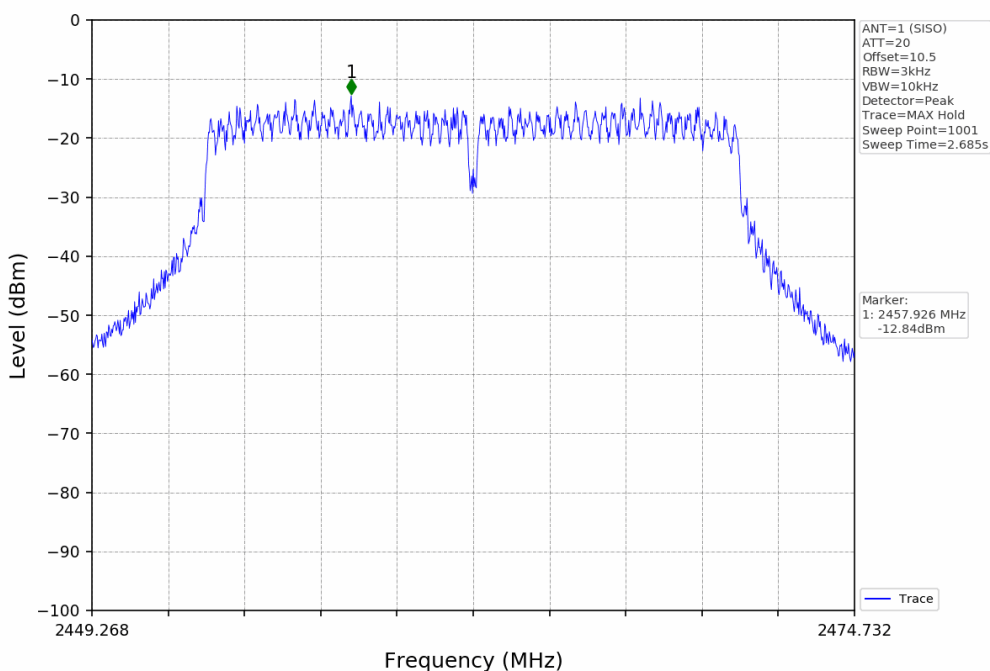
Maximum Power Spectral Density (PSD) NTVN_802.11n(HT20) SISO_2462MHz_ANT1
