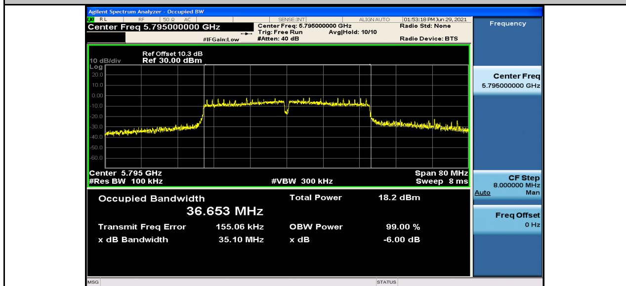
(6dB)Minimum Emission Bandwidth Measurement_11AC20_5745_Ant1
