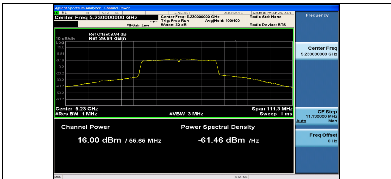
Maximum Conduct Output Power_11AC40_5270_Ant1
