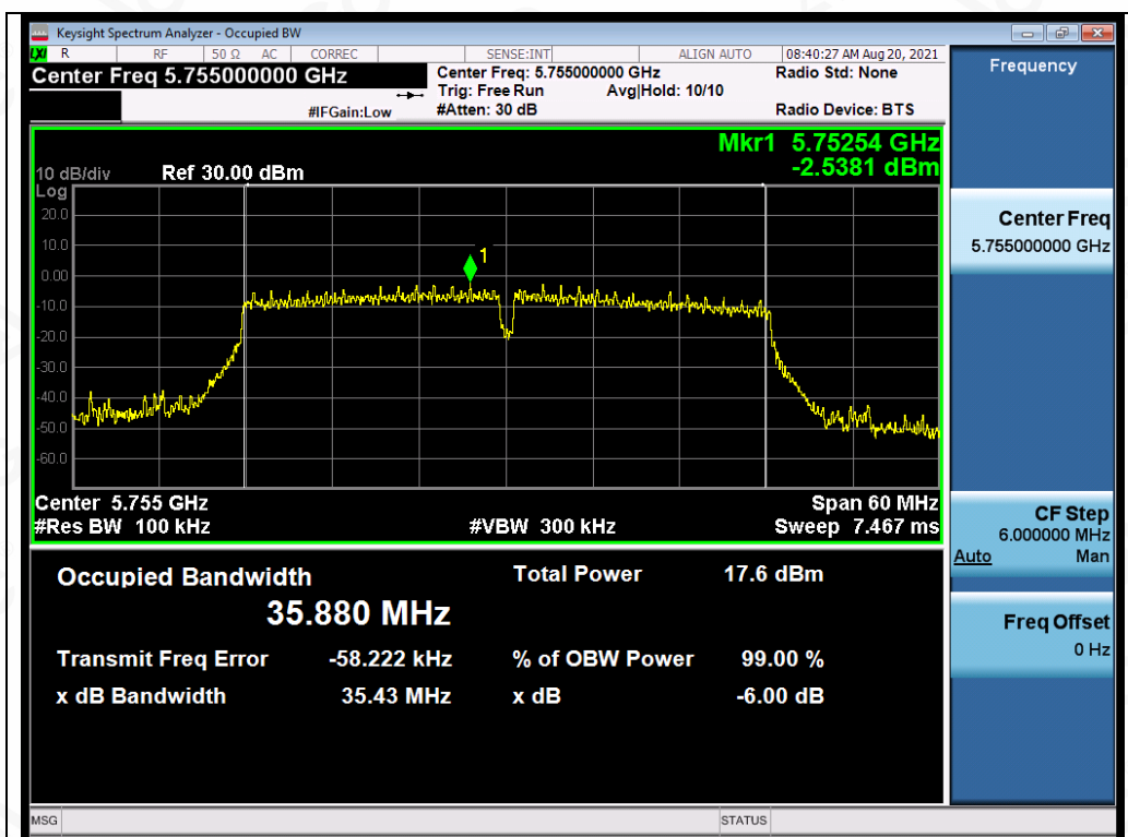
Test_Graph_802.11n40_ANT4_5755_MCS0_DTSBW
