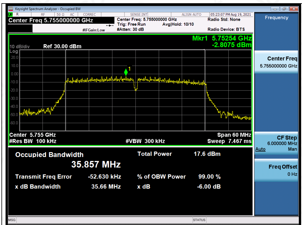
Test_Graph_802.11n40_ANT3_5755_MCS0_DTSBW
