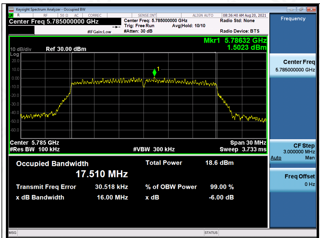
Test_Graph_802.11n20_ANT4_5785_MCS0_DTSBW
