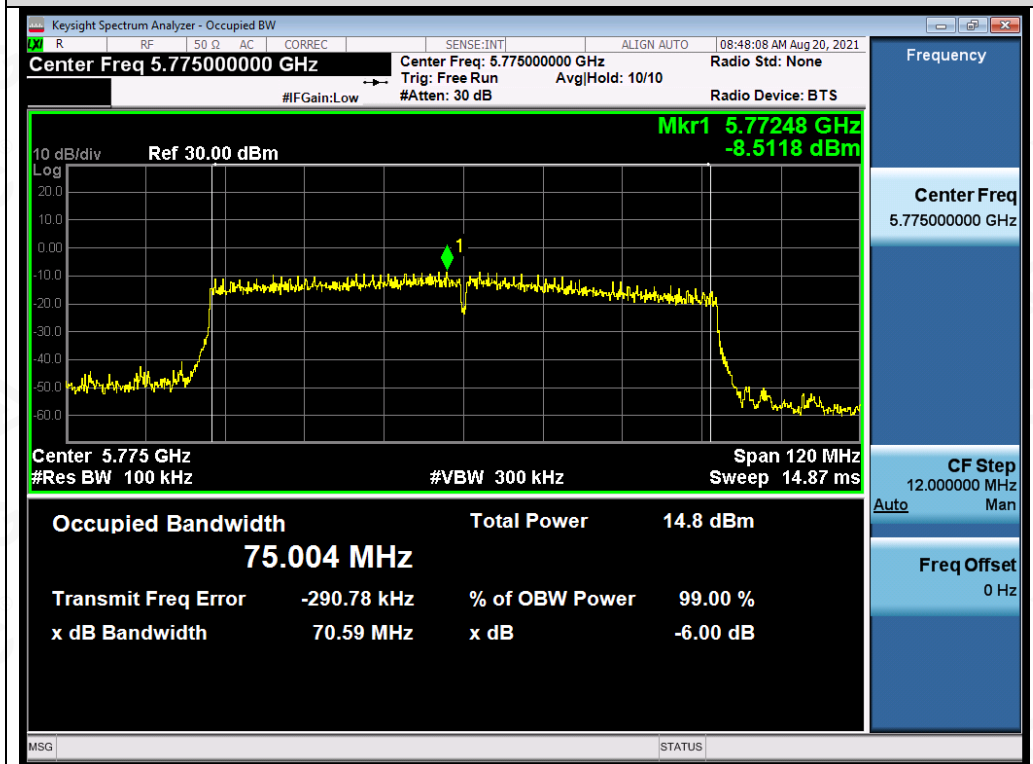
Test_Graph_802.11ac80_ANT4_5775_MCS9_DTSBW
