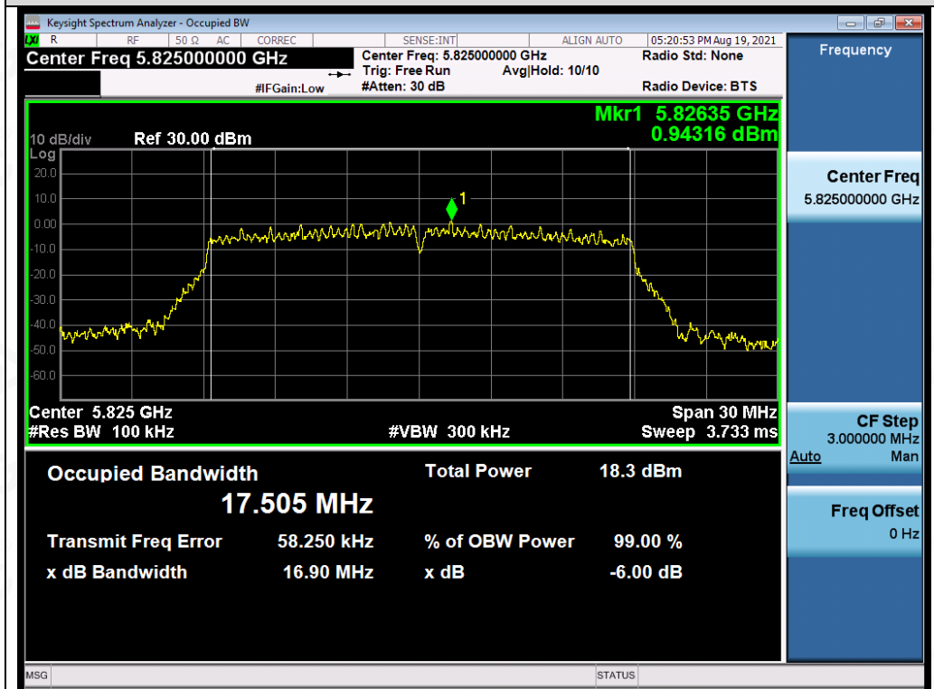
Test_Graph_802.11n20_ANT3_5825_MCS0_DTSBW
