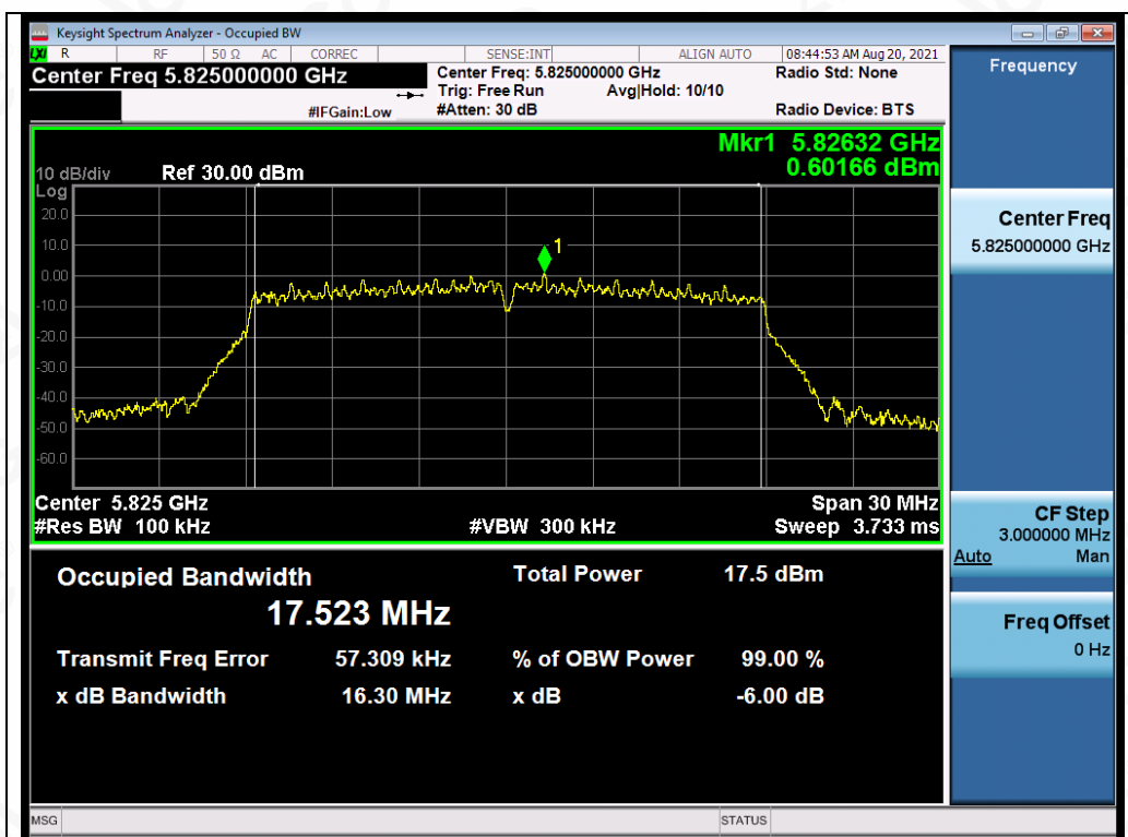
Test_Graph_802.11ac20_ANT4_5825_MCS9_DTSBW
