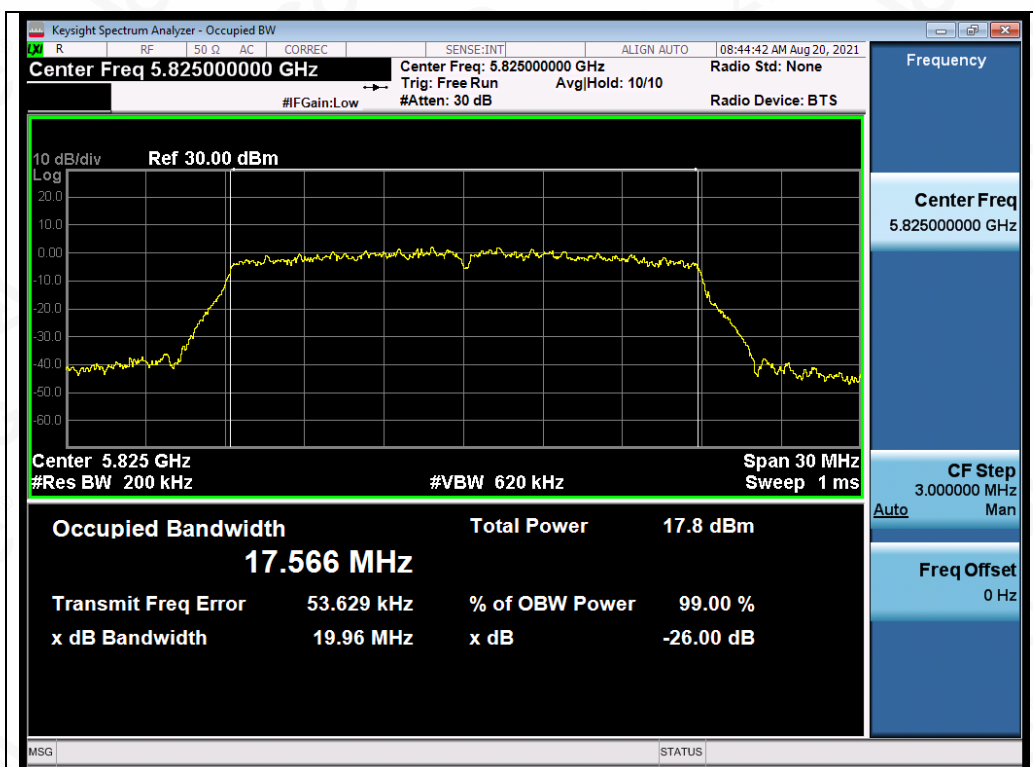
Test_Graph_802.11ac20_ANT4_5825_MCS9_OBW
