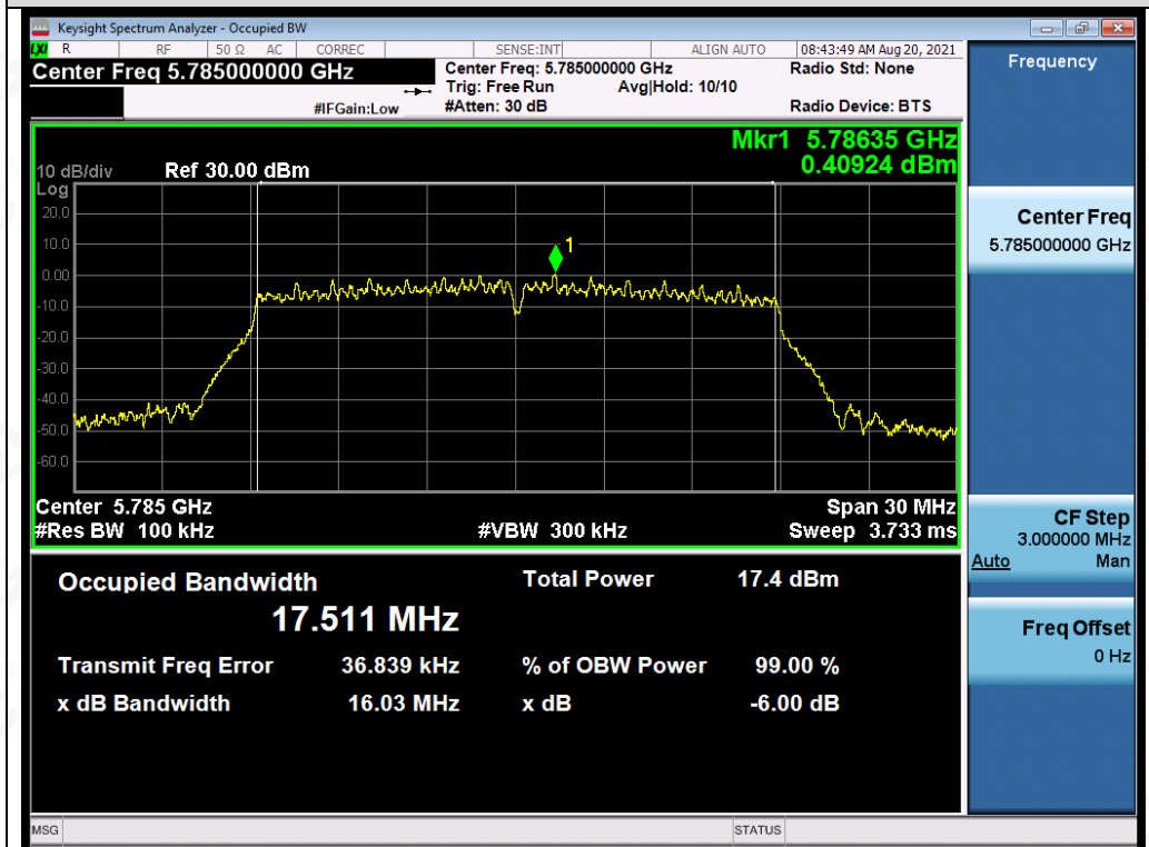
Test_Graph_802.11ac20_ANT4_5785_MCS0_DTSBW
