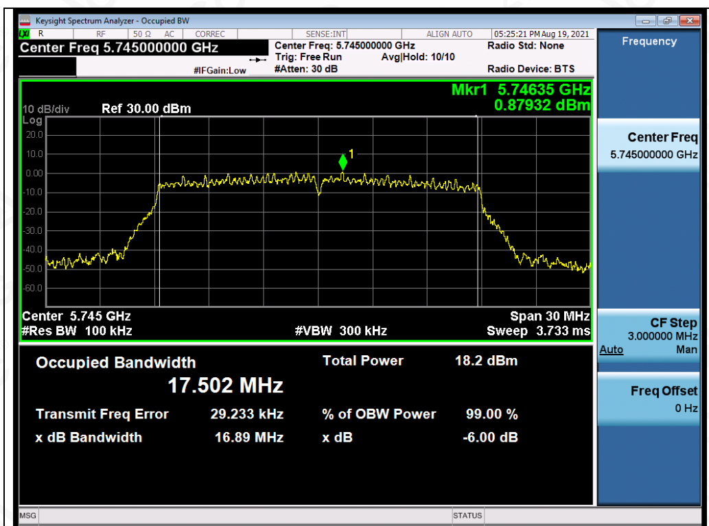
Test_Graph_802.11ac20_ANT3_5745_MCS0_DTSBW
