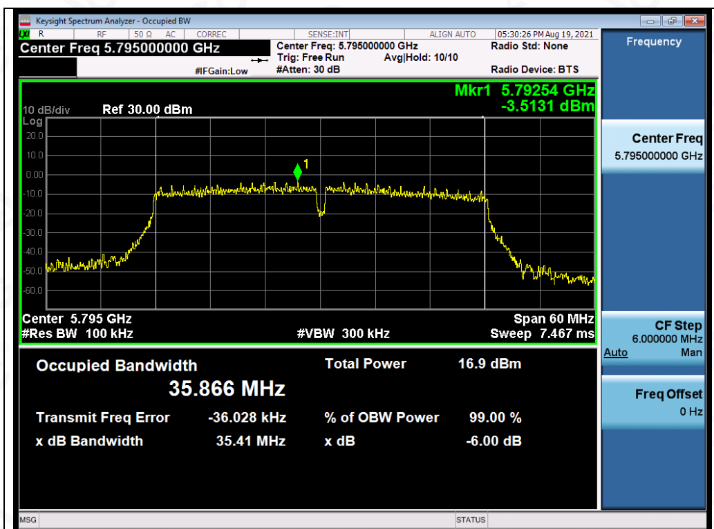
Test_Graph_802.11ac40_ANT3_5795_MCS9_DTSBW
