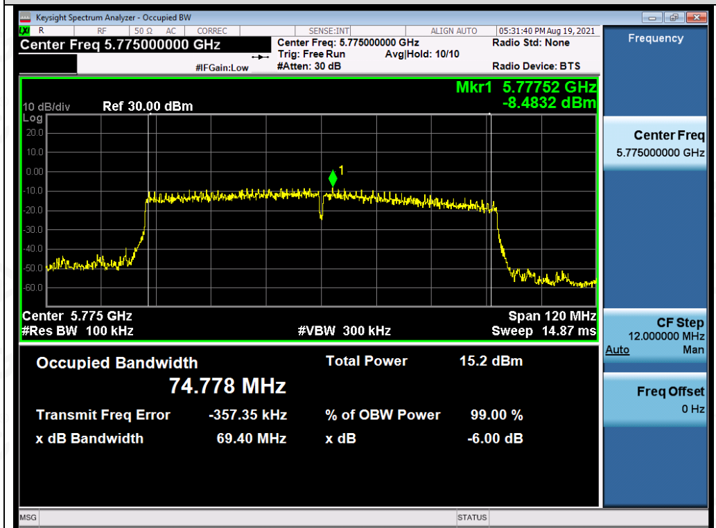
Test_Graph_802.11ac80_ANT3_5775_MCS9_DTSBW
