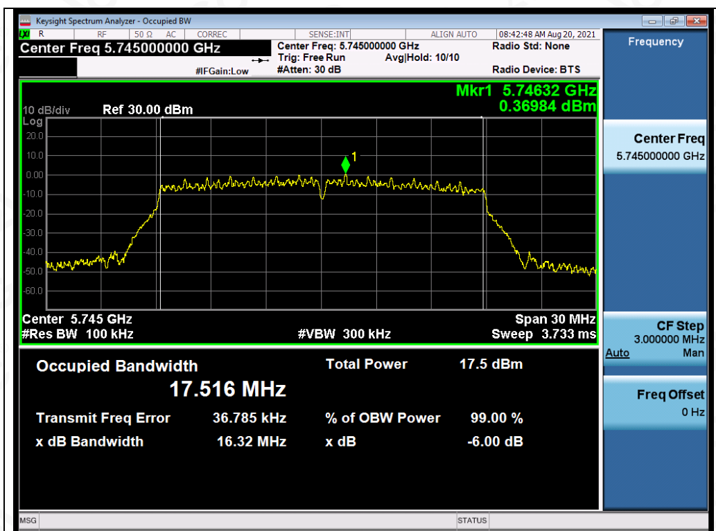
Test_Graph_802.11ac20_ANT4_5745_MCS0_DTSBW
