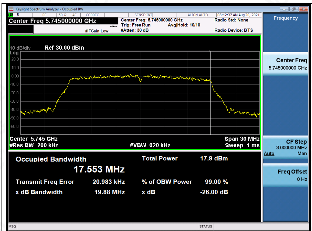
Test_Graph_802.11ac20_ANT4_5745_MCS0_OBW
