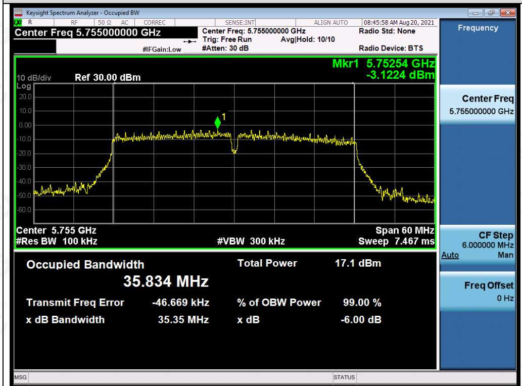
Test_Graph_802.11ac40_ANT4_5755_MCS9_DTSBW
