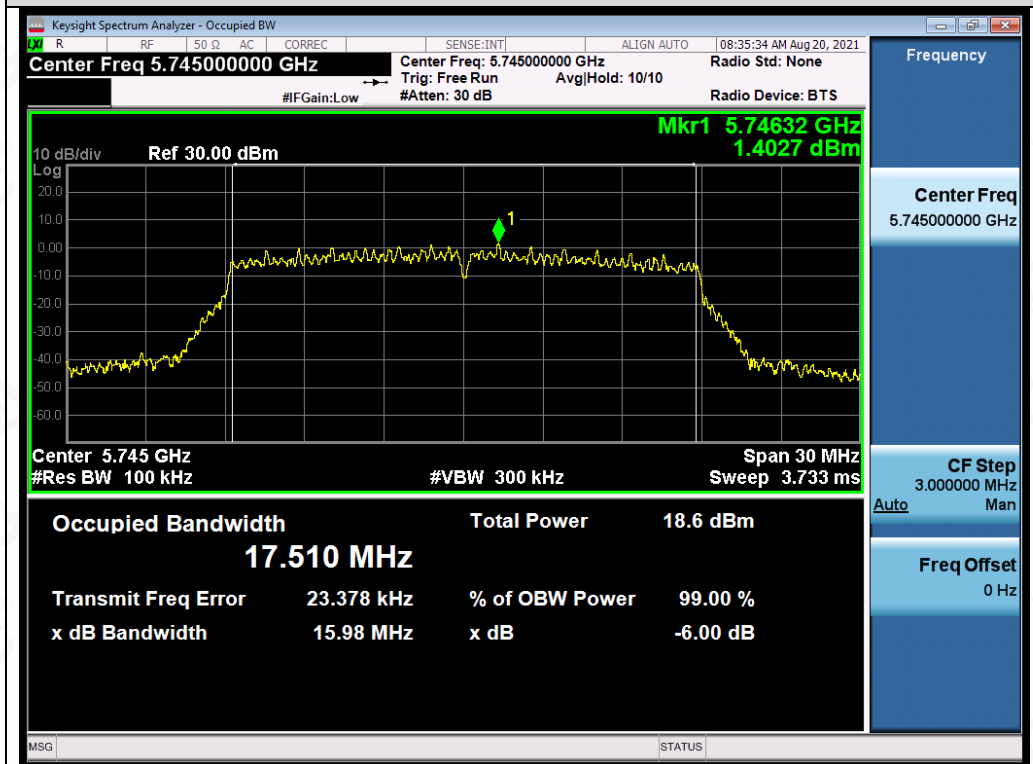
Test_Graph_802.11n20_ANT4_5745_MCS0_DTSBW
