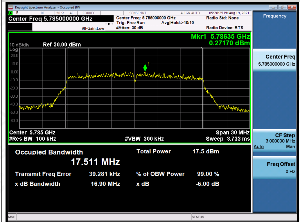
Test_Graph_802.11ac20_ANT3_5785_MCS0_DTSBW
