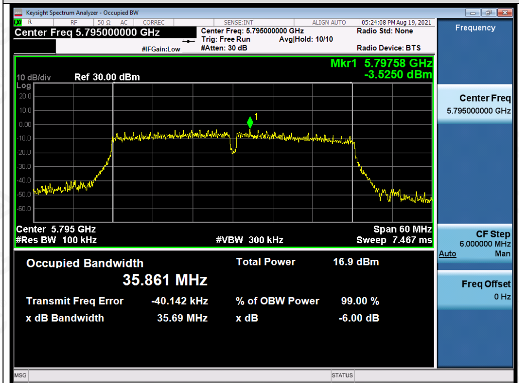
Test_Graph_802.11n40_ANT3_5795_MCS0_DTSBW
