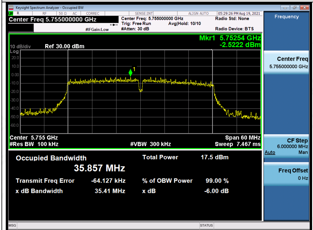
Test_Graph_802.11ac40_ANT3_5755_MCS9_DTSBW
