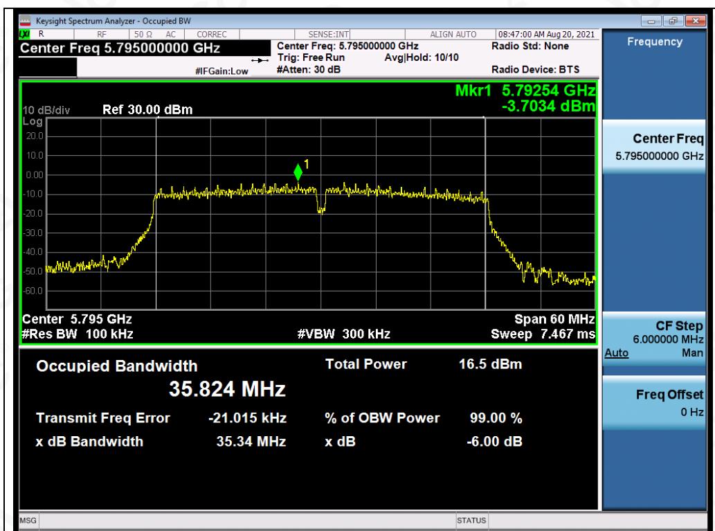
Test_Graph_802.11ac40_ANT4_5795_MCS9_DTSBW
