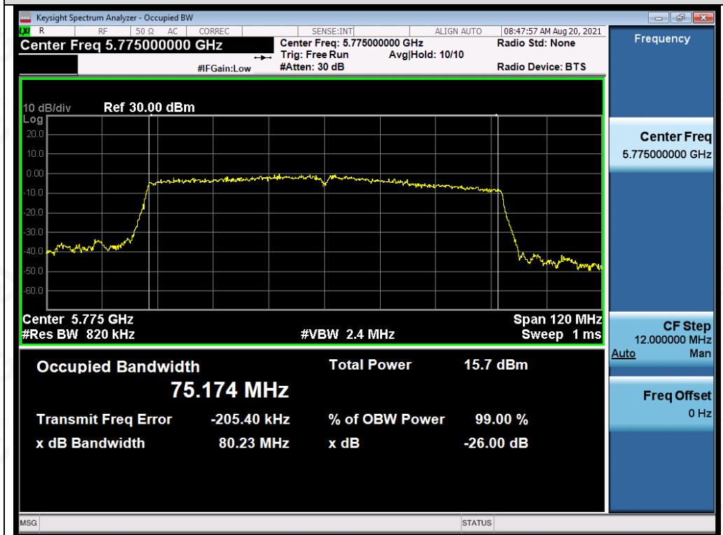
Test_Graph_802.11ac80_ANT4_5775_MCS9_OBW
