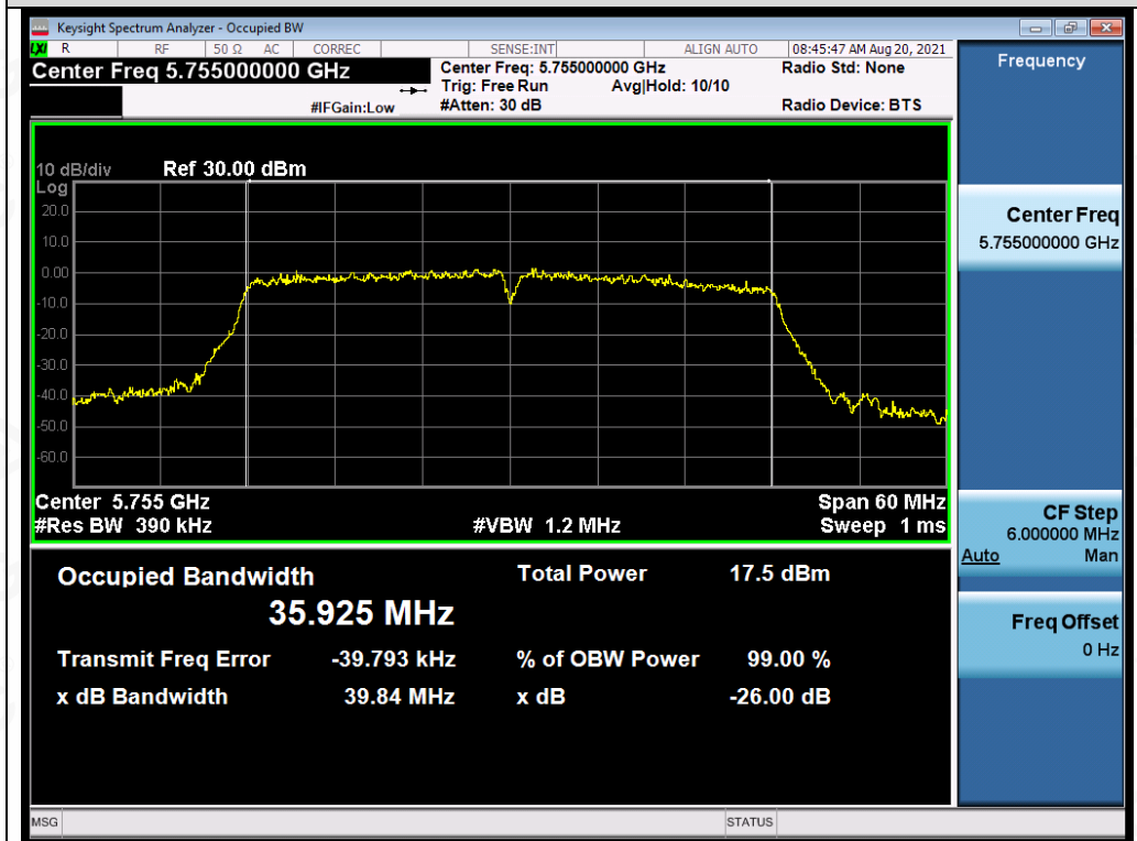
Test_Graph_802.11ac40_ANT4_5755_MCS9_OBW
