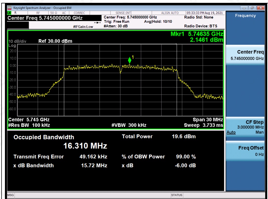
Test_Graph_802.11a_ANT4_5745_6Mbps_DTSBW
