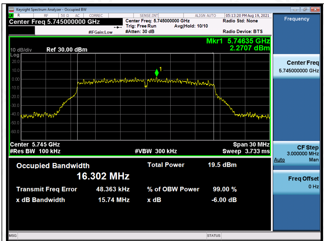
Test_Graph_802.11a_ANT3_5745_6Mbps_DTSBW
