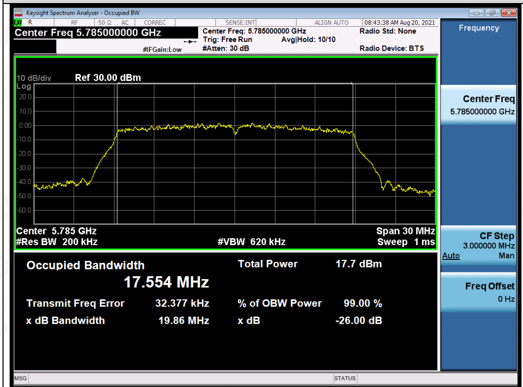
Test_Graph_802.11ac20_ANT4_5785_MCS0_OBW
