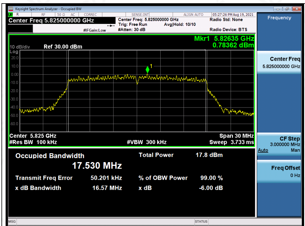
Test_Graph_802.11ac20_ANT3_5825_MCS9_DTSBW
