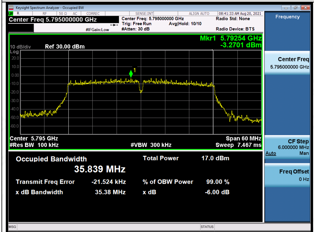
Test_Graph_802.11n40_ANT4_5795_MCS0_DTSBW
