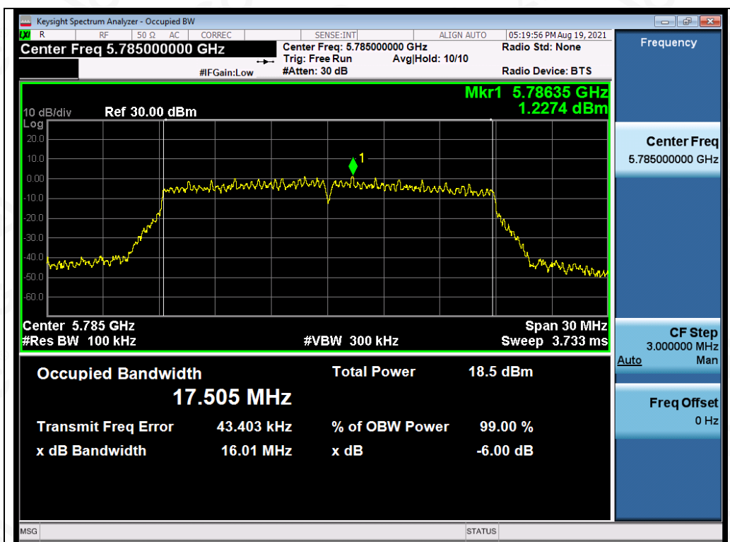
Test_Graph_802.11n20_ANT3_5785_MCS0_DTSBW
