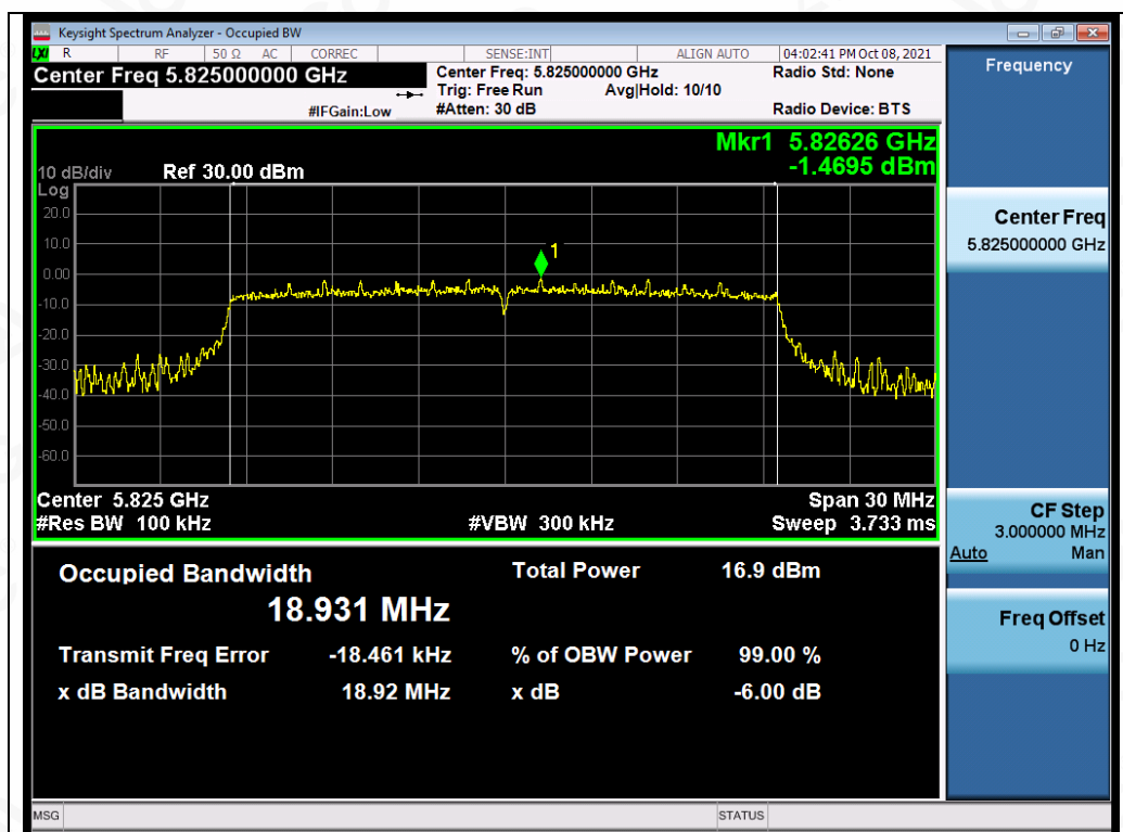
Test_Graph_802.11ax20_ANT2_5825_MCS0_DTSBW
