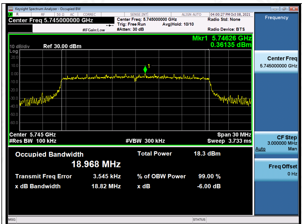
Test_Graph_802.11ax20_ANT2_5745_MCS0_DTSBW
