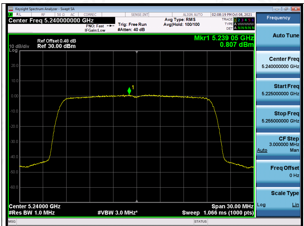
Test_Graph_802.11ax20_ANT1_5240_MCS0_PSD
