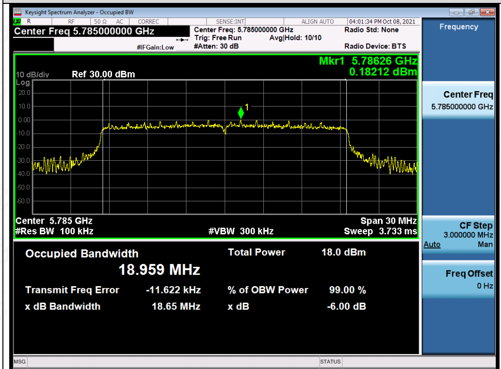
Test_Graph_802.11ax20_ANT2_5785_MCS0_DTSBW
