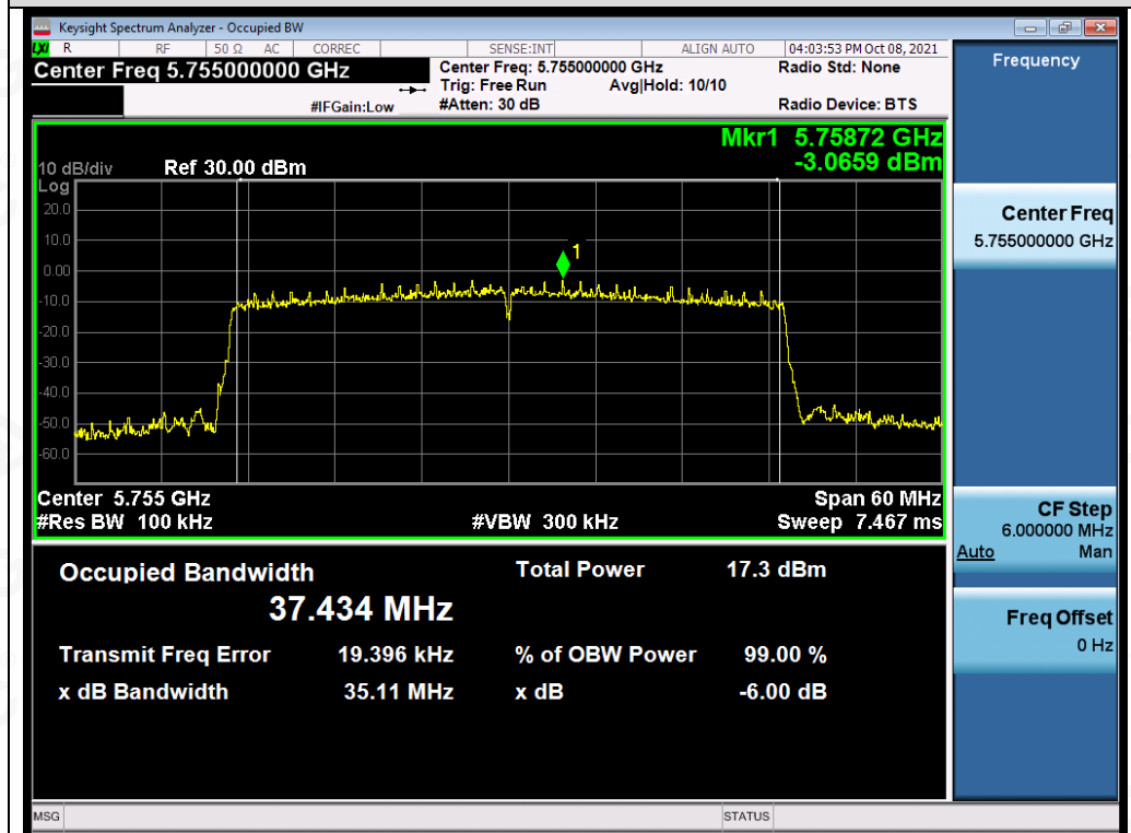
Test_Graph_802.11ax40_ANT2_5755_MCS0_DTSBW
