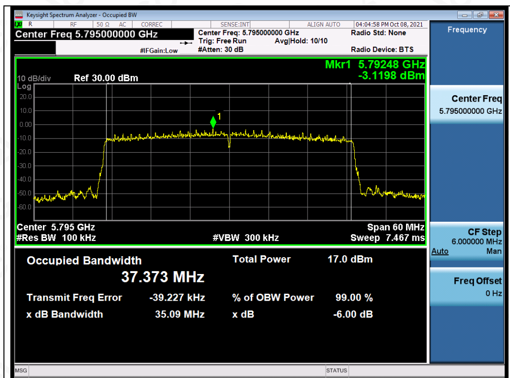
Test_Graph_802.11ax40_ANT2_5795_MCS0_DTSBW
