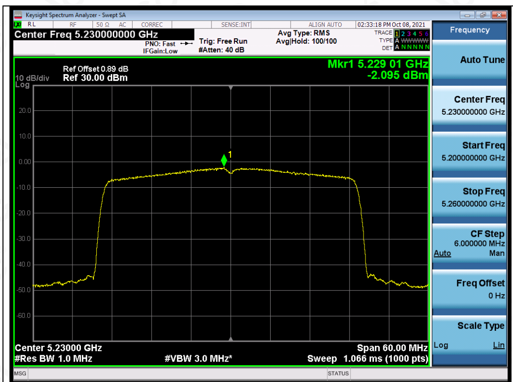
Test_Graph_802.11ax40_ANT2_5230_MCS0_PSD
