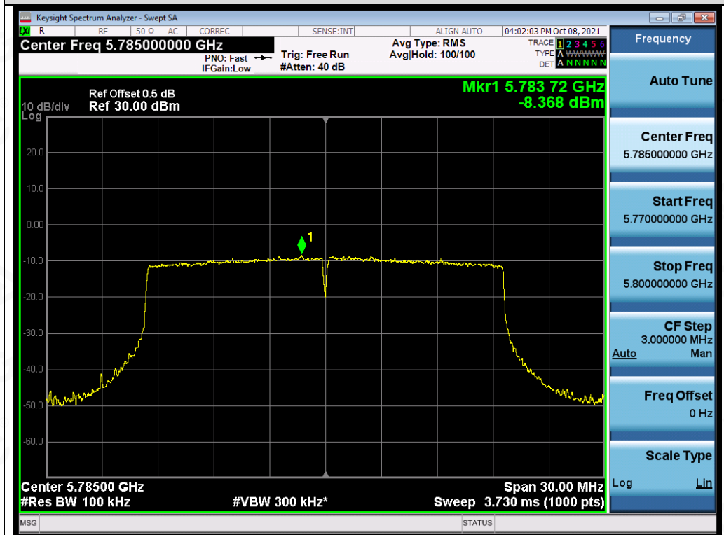
Test_Graph_802.11ax20_ANT2_5785_MCS0_PSD
