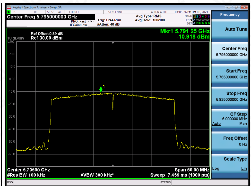
Test_Graph_802.11ax40_ANT2_5795_MCS0_PSD
