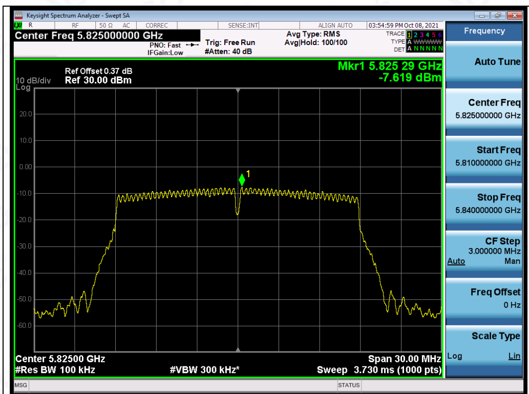
Test_Graph_802.11ac20_ANT2_5825_MCS9_PSD
