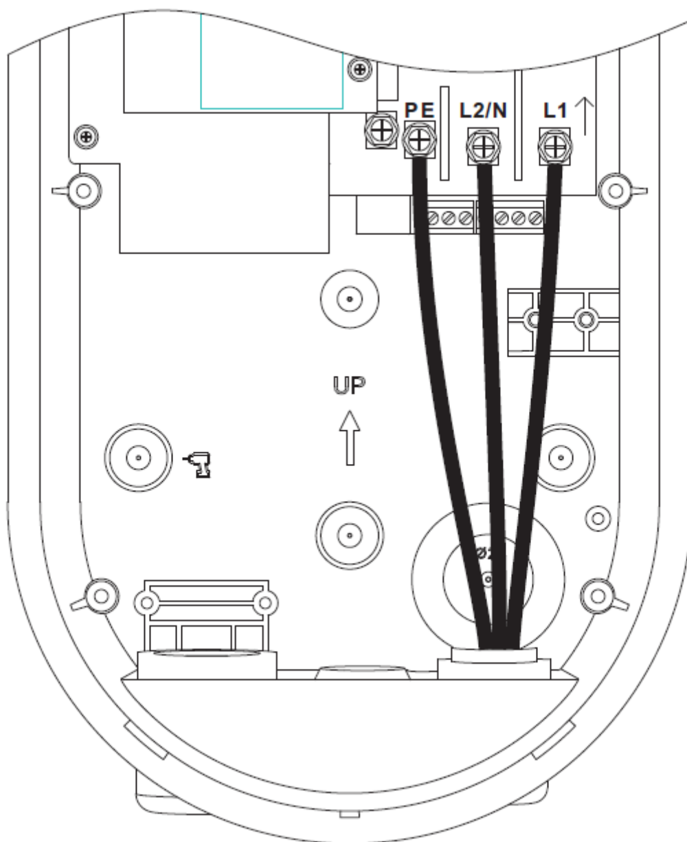
Figure 2-8 Wiring diagram
