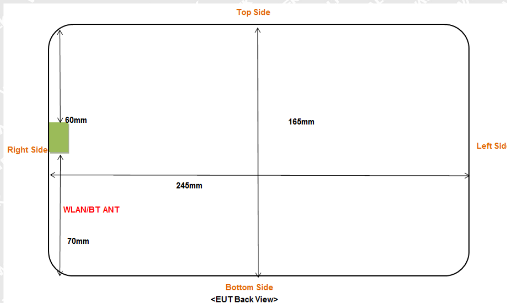
Fig 7.1 Block Diagram for EUT Antenna Position
