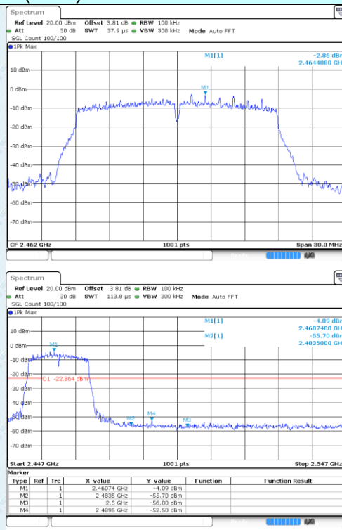
Highest channel
