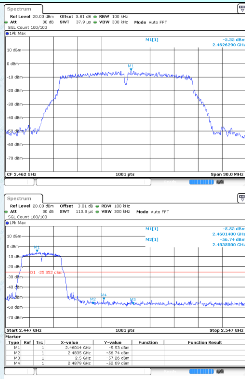
Highest channel
