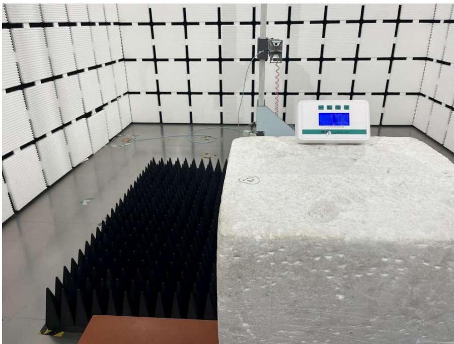
Radiated Emission Test View Above 1GHz
