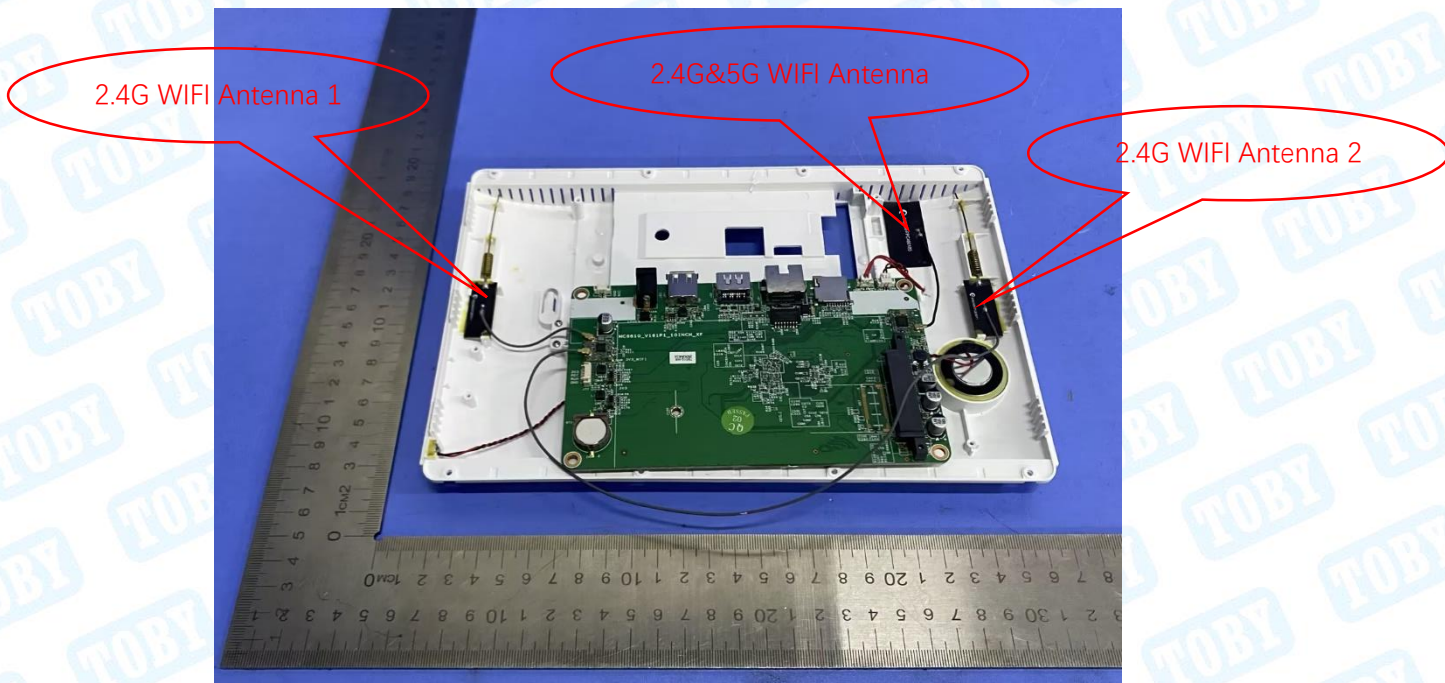
Photo 12 Internal of EUT
