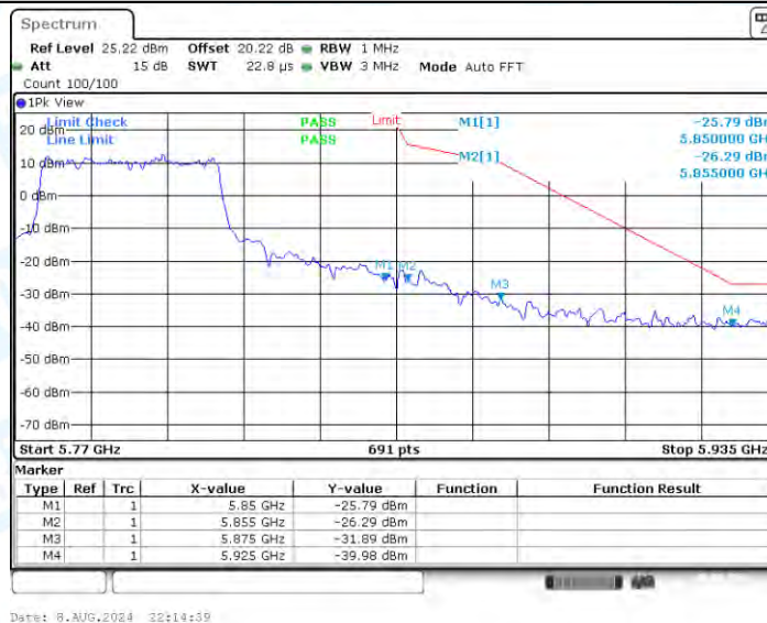
11AX40SISO_Ant1_High_5795_Peak
