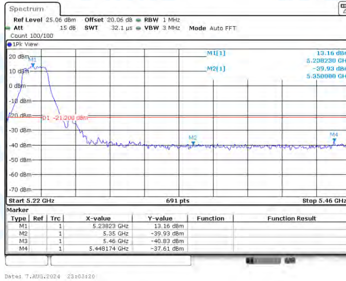
11N20SISO_Ant1_High_5240_Peak
