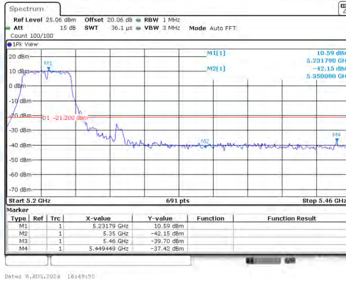
11N40SISO_Ant1_High_5230_Peak
