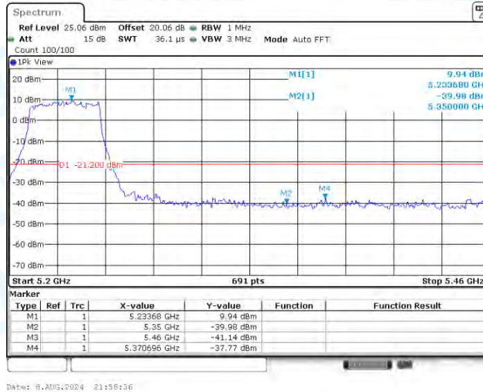
11AX40SISO_Ant1_High_5230_Peak
