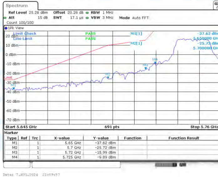
11N20SISO_Ant1_Low_5745_Peak
