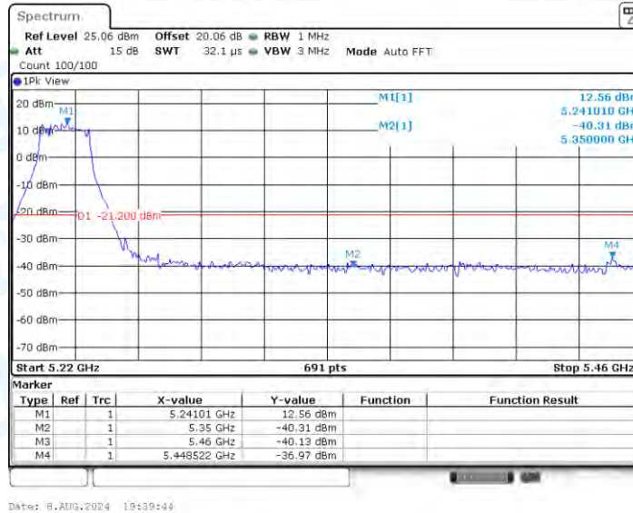
11AX20SISO_Ant1_High_5240_Peak
