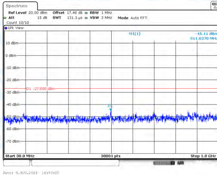
11N40SISO_Ant1_5230_30~1000
