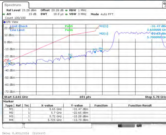
11AX40SISO_Ant1_Low_5755_Peak
