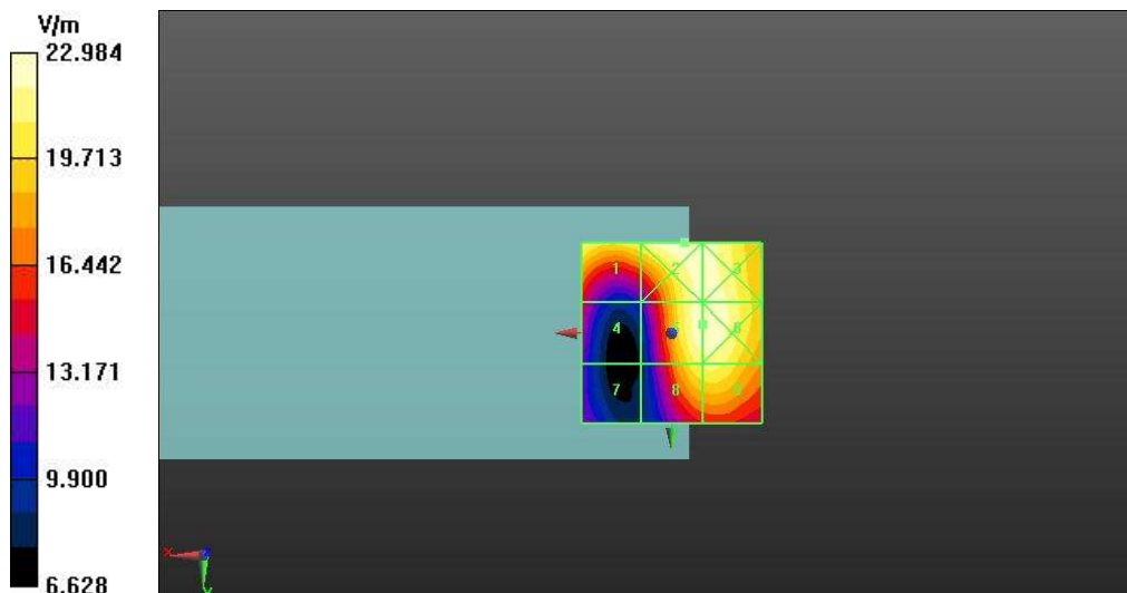
Fig A.9 HAC RF E-Field LTE Band 41
