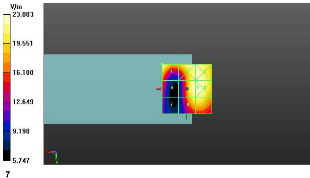
Fig A.8 HAC RF E-Field LTE Band 41
