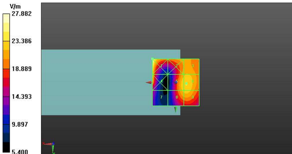
Fig A.7 HAC RF E-Field LTE Band 41
