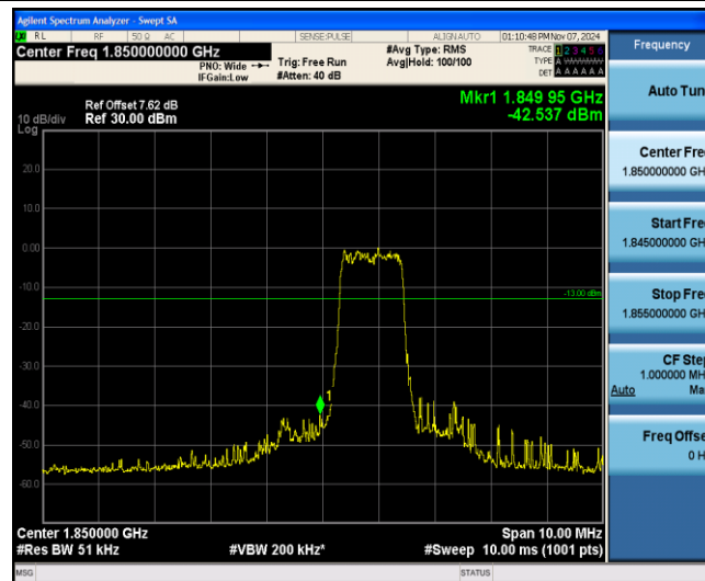
Band25-3MHz-16QAM-26055-6-0-Low--42.54-PASS
