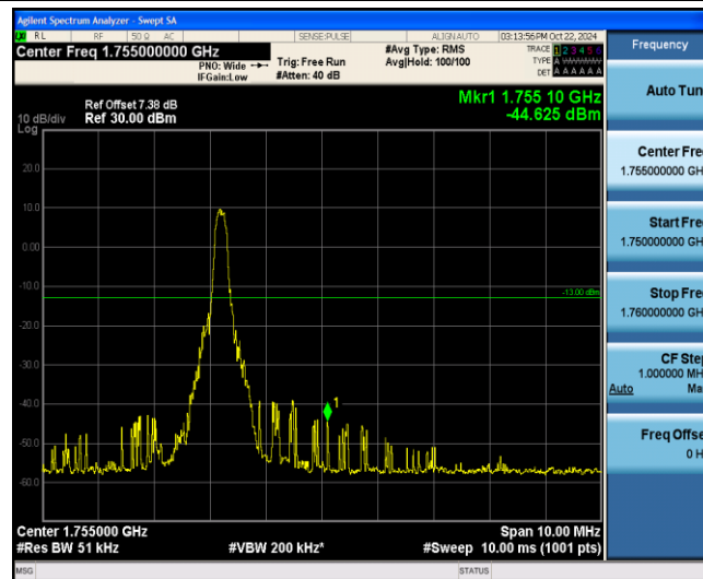
Band4-20MHz-16QAM-20300-1-5-High--44.62-PASS
