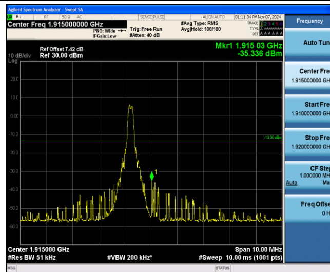
Band25-3MHz-QPSK-26675-1-5-High--35.34-PASS
