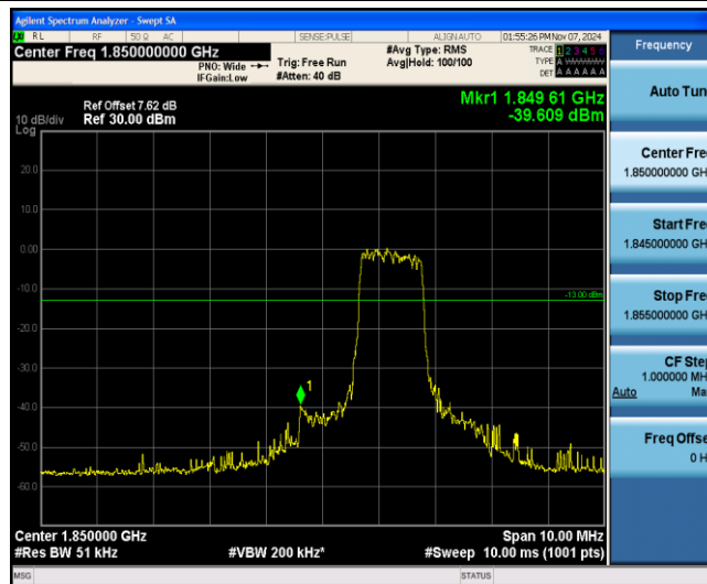
Band25-10MHz-QPSK-26090-6-0-Low--39.61-PASS
