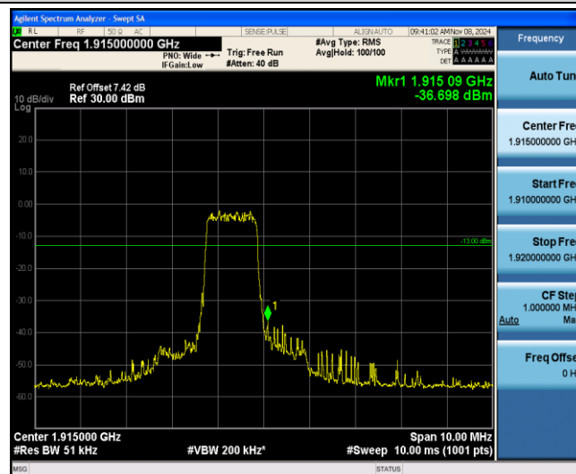
Band25-1.4MHz-QPSK-26683-6-0-High--36.70-PASS
