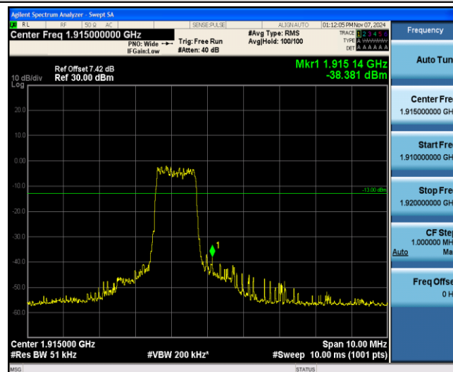
Band25-3MHz-16QAM-26675-6-0-High--38.38-PASS
