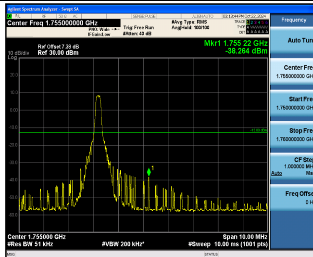
Band4-20MHz-QPSK-20300-1-5-High--38.26-PASS
