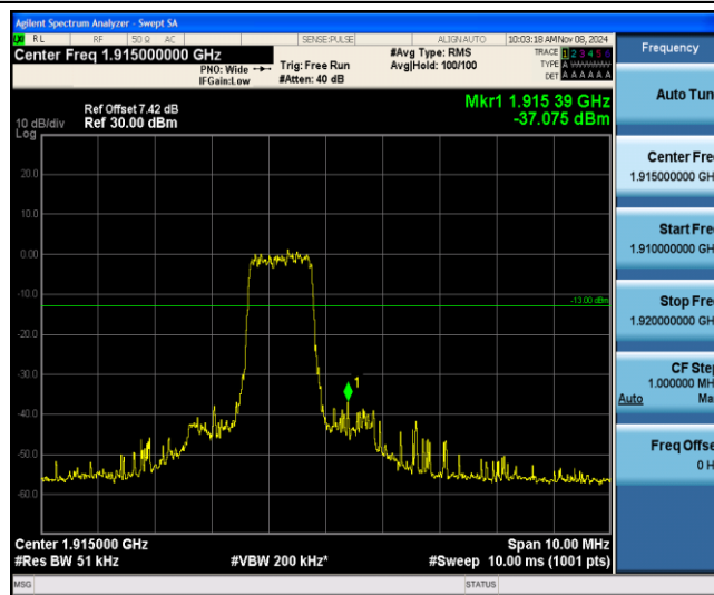
Band25-5MHz-16QAM-26665-6-0-High--37.08-PASS
