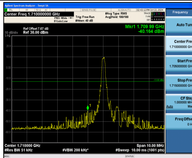
Band4-15MHz-16QAM-20025-1-0-Low--40.16-PASS
