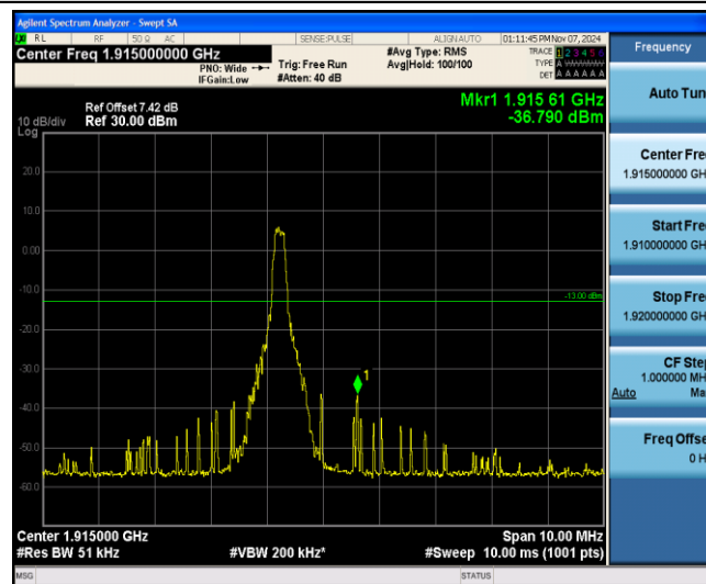
Band25-3MHz-16QAM-26675-1-5-High--36.79-PASS
