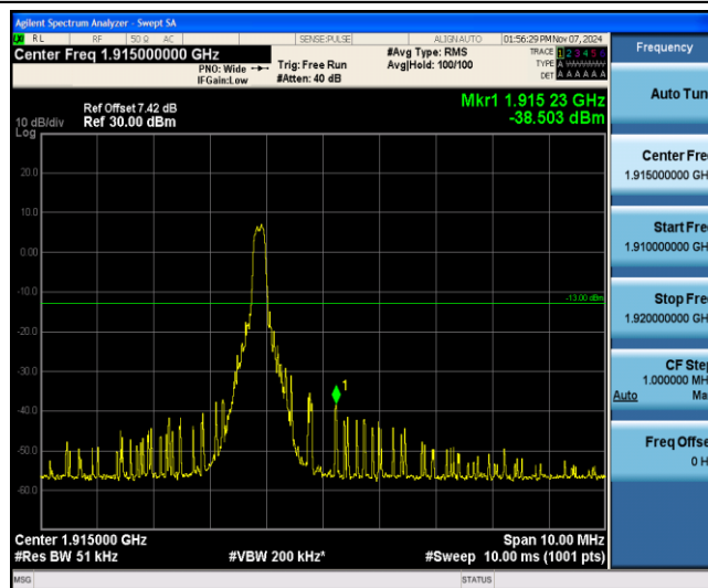
Band25-10MHz-QPSK-26640-1-5-High--38.50-PASS
