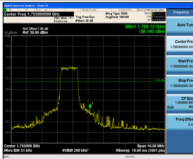
Band4-10MHz-16QAM-20350-6-0-High--38.14-PASS
