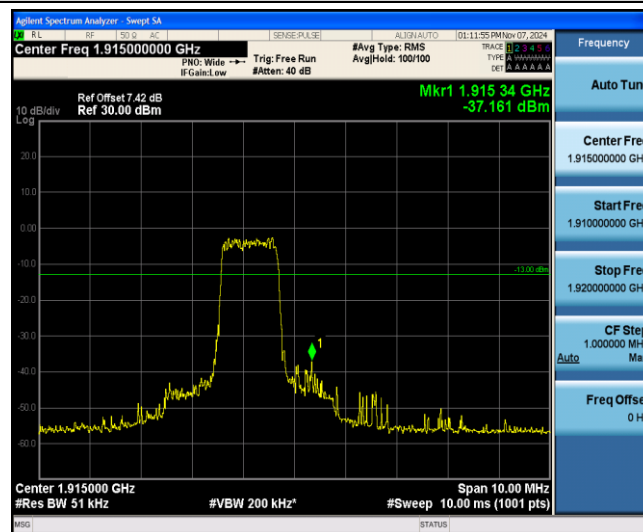
Band25-3MHz-QPSK-26675-6-0-High--37.16-PASS
