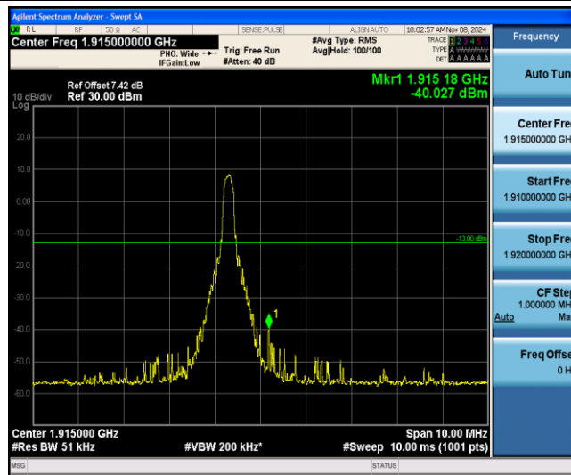
Band25-5MHz-16QAM-26665-1-5-High--40.03-PASS
