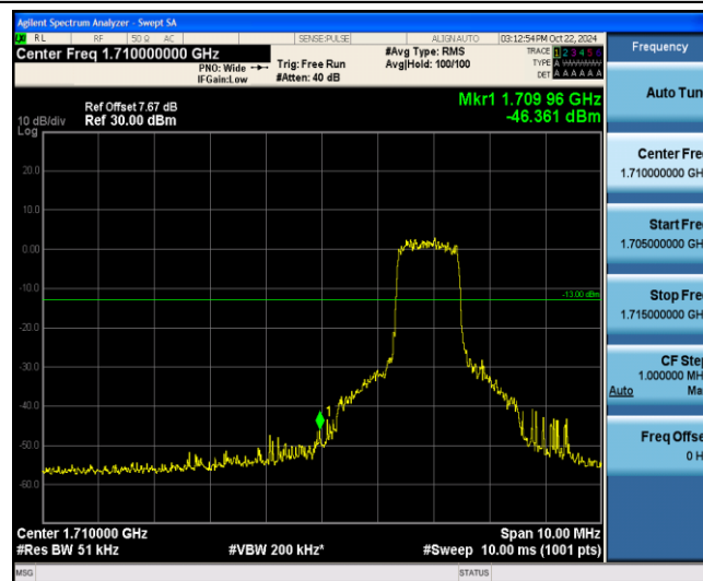
Band4-20MHz-QPSK-20050-6-0-Low--46.36-PASS
