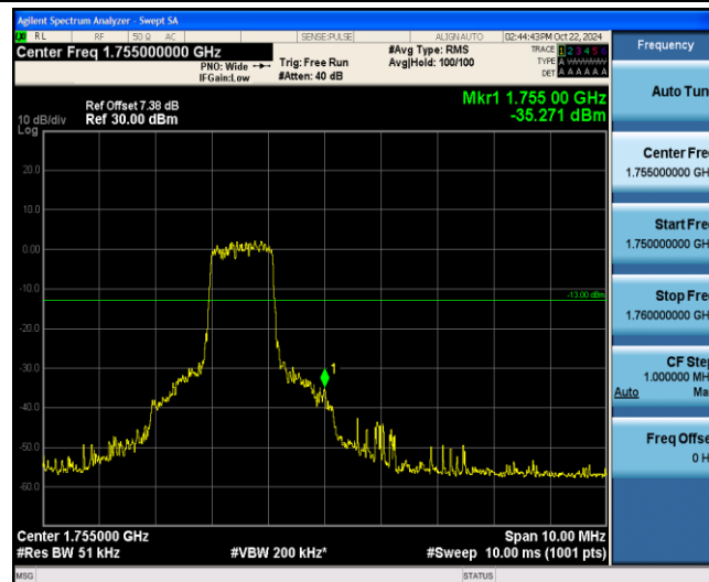
Band4-15MHz-16QAM-20325-6-0-High--35.27-PASS
