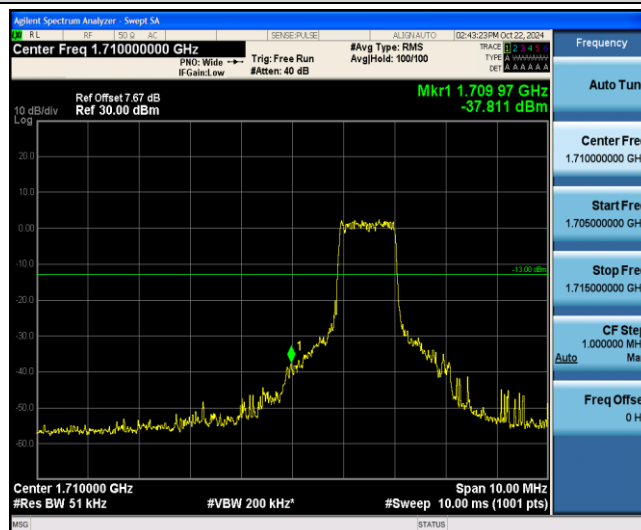
Band4-15MHz-QPSK-20025-6-0-Low--37.81-PASS
