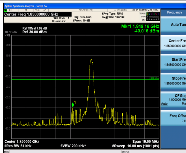
Band25-3MHz-16QAM-26055-1-0-Low--40.02-PASS
