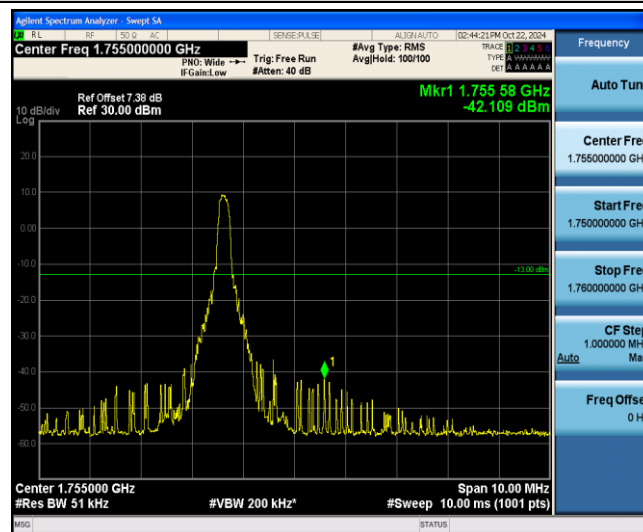
Band4-15MHz-16QAM-20325-1-5-High--42.11-PASS
