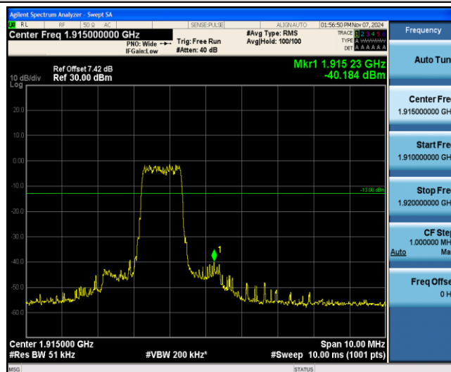
Band25-10MHz-QPSK-26640-6-0-High--40.18-PASS
