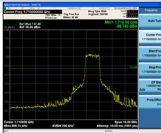
Band4-15MHz-16QAM-20025-6-0-Low--38.14-PASS
