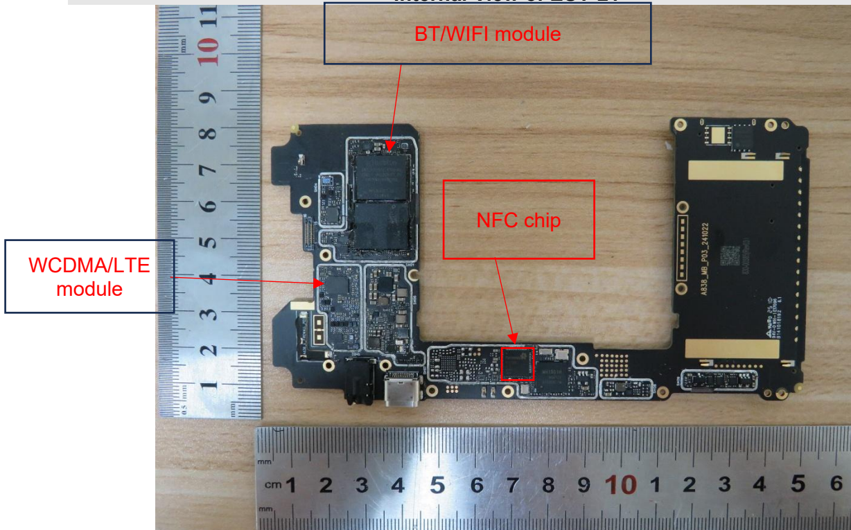
Internal View of EUT-22
