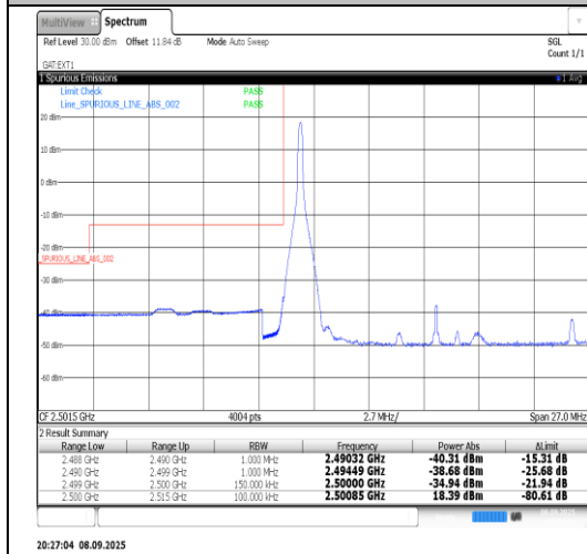
Band41-15MHz-16QAM-39765-75RB#0-PASS
