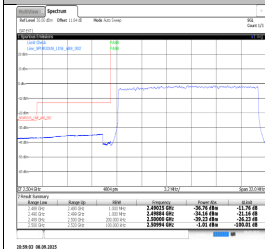
Band41-20MHz-16QAM-39790-100RB#0-PASS
