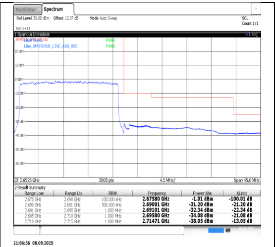
Band41-20MHz-16QAM-39790-1RB#99-PASS
