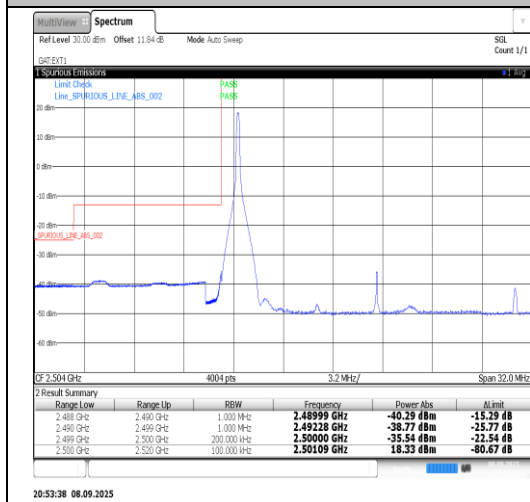
Band41-20MHz-16QAM-39790-100RB#0-PASS
