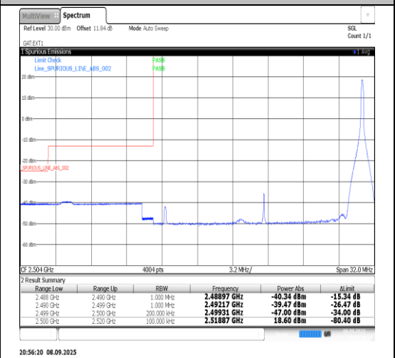
Band41-20MHz-16QAM-39790-1RB#99-PASS
