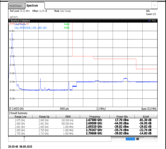
Band41-15MHz-16QAM-41515-75RB#0-PASS
