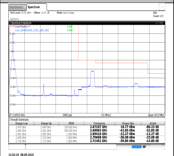
Band41-20MHz-16QAM-41490-100RB#0-PASS
