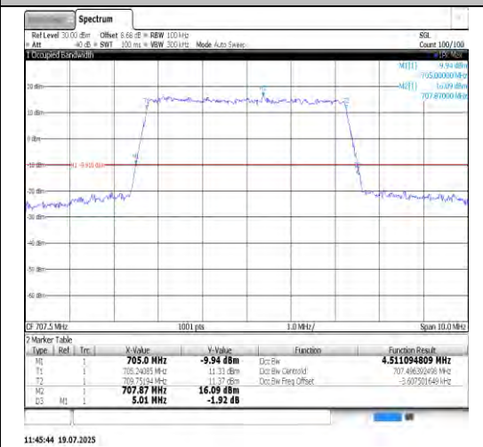
Band12-10MHz-16QAM-23095-50RB#0-PASS
