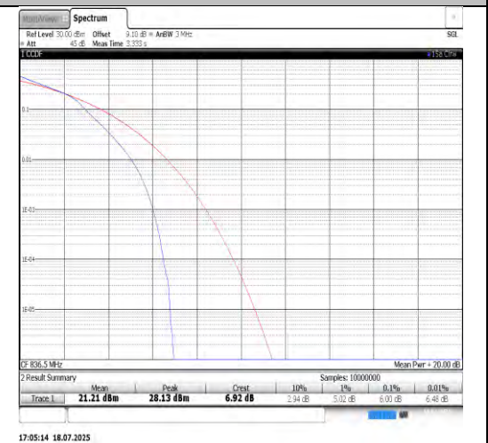
Band5-5MHz-16QAM-20525-25RB#0-PASS
