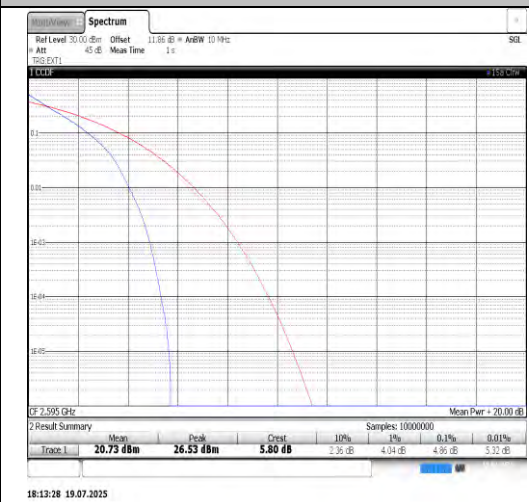
Band38-15MHz-QPSK-38000-75RB#0-PASS
