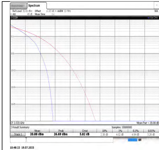
Band7-15MHz-QPSK-21100-75RB#0-PASS
