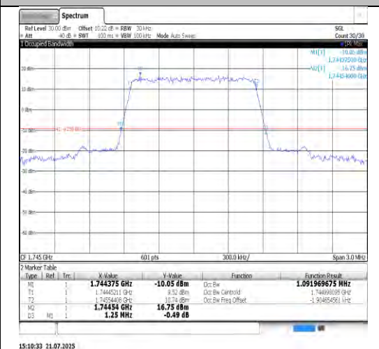
Band66-3MHz-QPSK-132322-15RB#0-PASS
