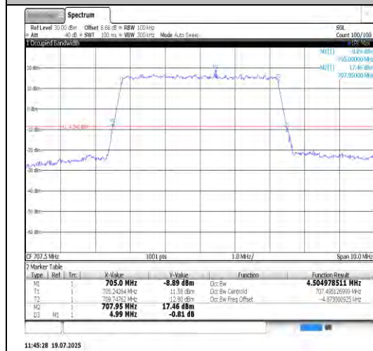
Band12-10MHz-QPSK-23095-50RB#0-PASS
