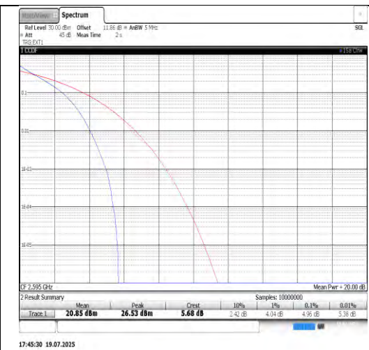
Band38-10MHz-QPSK-38000-50RB#0-PASS
