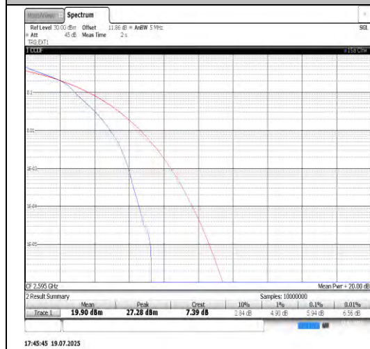
Band38-10MHz-16QAM-38000-50RB#0-PASS
