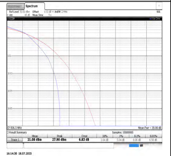
Band5-3MHz-16QAM-20525-15RB#0-PASS
