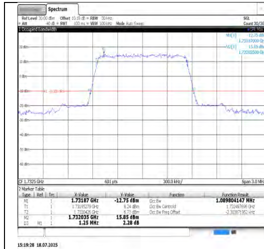
Band4-3MHz-QPSK-20175-15RB#0-PASS
