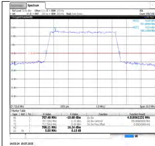
Band17-10MHz-16QAM-23790-50RB#0-PASS
