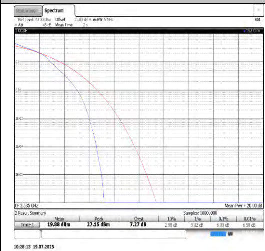
Band7-10MHz-16QAM-21100-50RB#0-PASS
