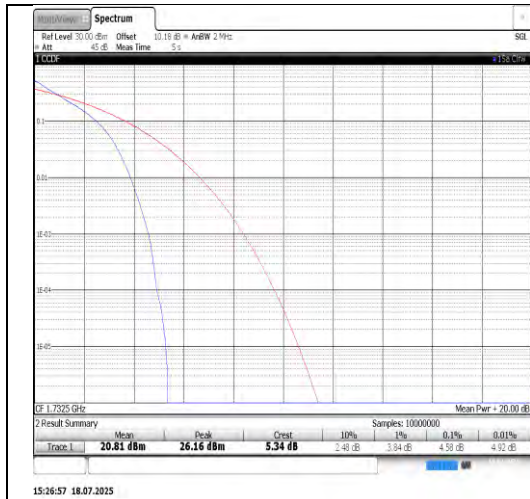
Band4-3MHz-QPSK-20175-15RB#0-PASS
