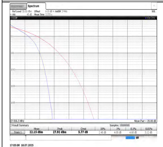
Band5-5MHz-QPSK-20525-25RB#0-PASS
