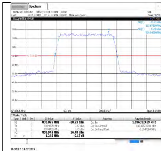
Band26(824-849)-3MHz-16QAM-26915-15RB#0-PASS
