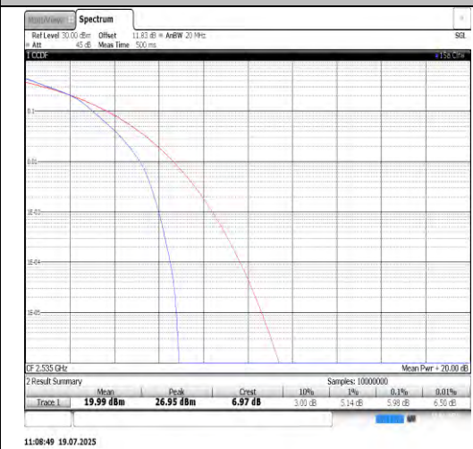
Band7-20MHz-16QAM-21100-100RB#0-PASS
