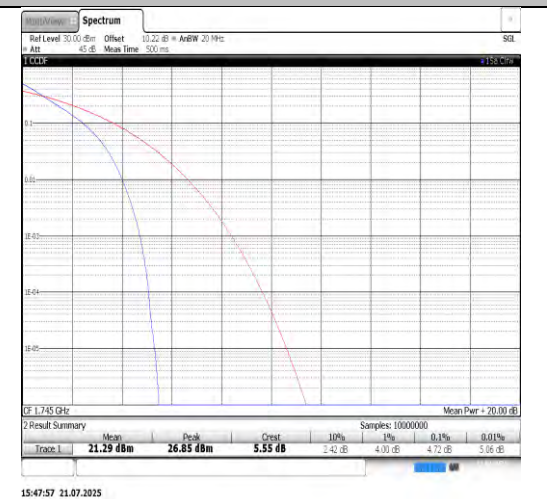
Band66-20MHz-QPSK-132322-100RB#0-PASS
