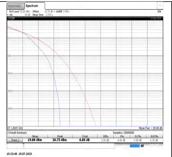
Band25-5MHz-16QAM-26365-25RB#0-PASS
