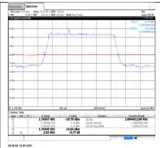
Band66-5MHz-QPSK-132322-25RB#0-PASS
