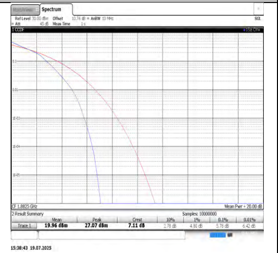
Band25-15MHz-16QAM-26365-75RB#0-PASS
