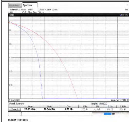
Band7-20MHz-QPSK-21100-100RB#0-PASS
