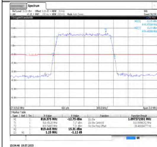
Band26(814-824)-3MHz-16QAM-26740-15RB#0-PASS
