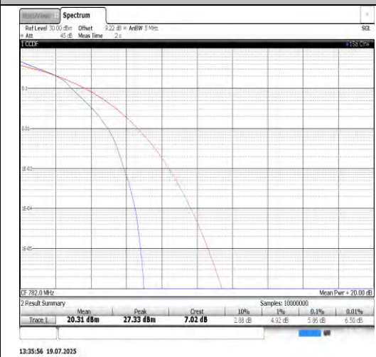
Band13-10MHz-16QAM-23230-50RB#0-PASS
