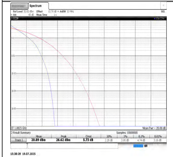
Band25-15MHz-QPSK-26365-75RB#0-PASS
