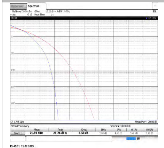
Band66-15MHz-16QAM-132322-75RB#0-PASS
