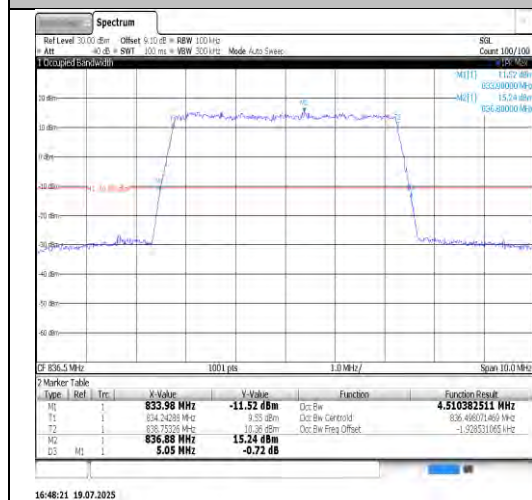
Band26(824-849)-10MHz-16QAM-26915-50RB#0-PASS
