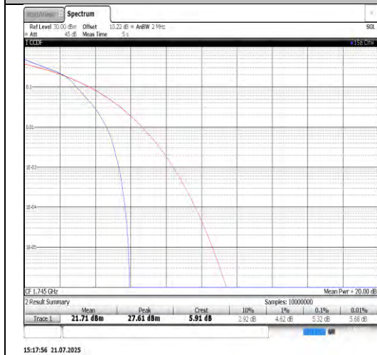
Band66-3MHz-16QAM-132322-15RB#0-PASS
