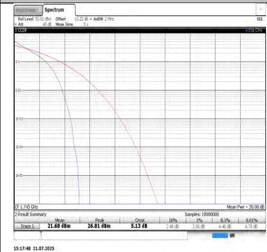
Band66-3MHz-QPSK-132322-15RB#0-PASS
