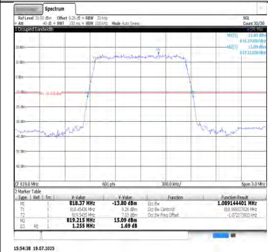
Band26(814-824)-3MHz-QPSK-26740-15RB#0-PASS
