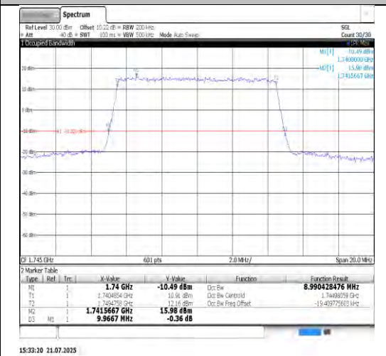
Band66-10MHz-QPSK-132322-50RB#0-PASS
