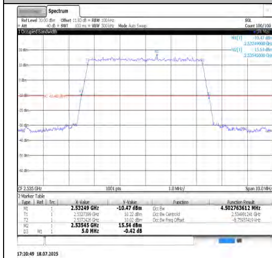
Band7-10MHz-QPSK-21100-50RB#0-PASS
