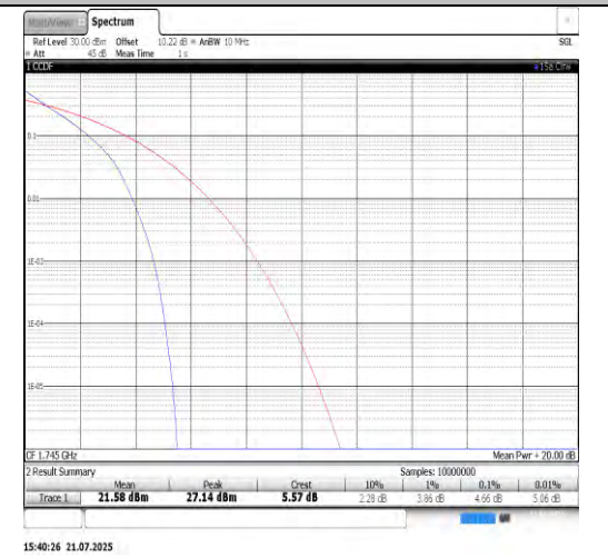
Band66-10MHz-QPSK-132322-50RB#0-PASS
