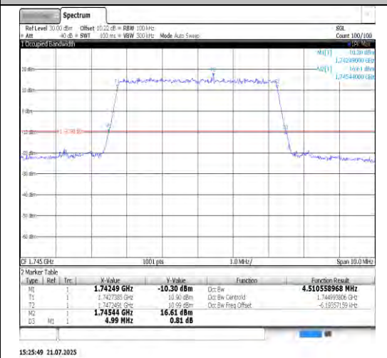
Band66-10MHz-QPSK-132322-50RB#0-PASS
