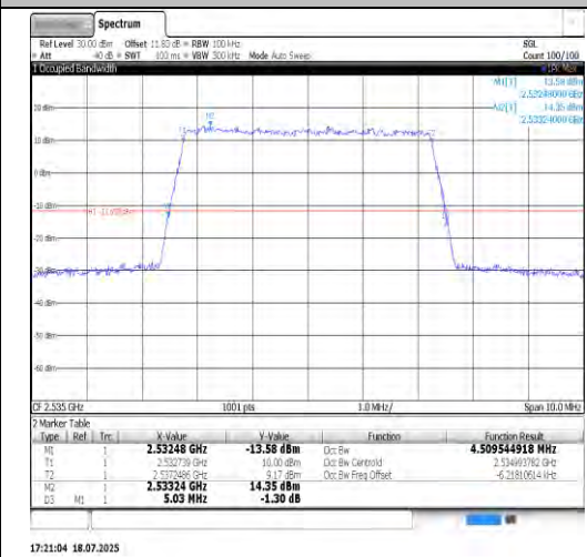
Band7-10MHz-16QAM-21100-50RB#0-PASS
