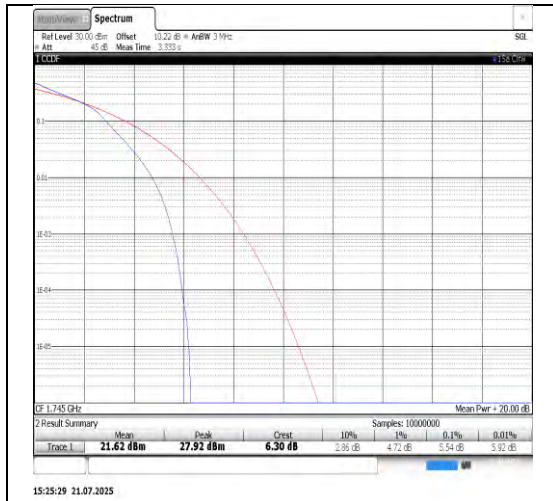
Band66-5MHz-16QAM-132322-25RB#0-PASS
