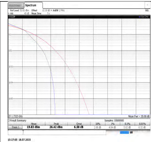
Band4-3MHz-16QAM-20175-15RB#0-PASS
