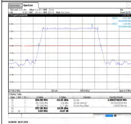
Band5-5MHz-QPSK-20525-25RB#0-PASS
