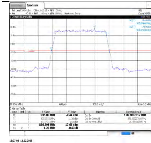
Band5-3MHz-QPSK-20525-15RB#0-PASS
