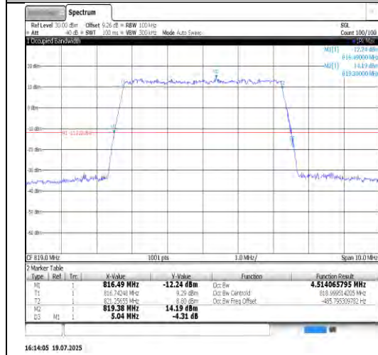
Band26(814-824)-10MHz-16QAM-26740-50RB#0-PASS
