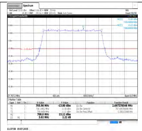
Band12-5MHz-16QAM-23095-25RB#0-PASS
