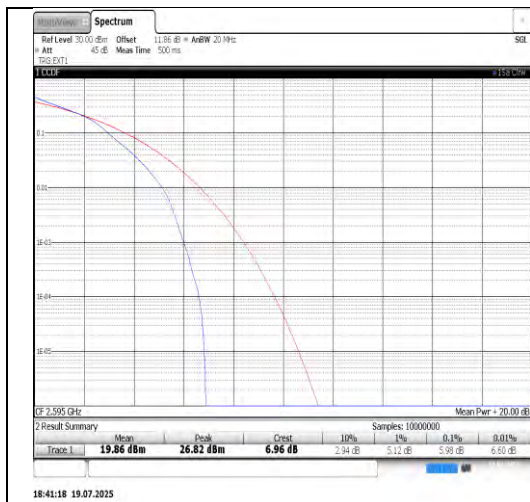
Band38-20MHz-16QAM-38000-100RB#0-PASS
