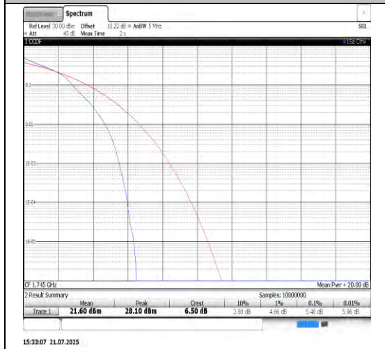
Band66-10MHz-16QAM-132322-50RB#0-PASS
