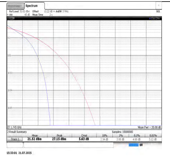
Band66-10MHz-QPSK-132322-50RB#0-PASS
