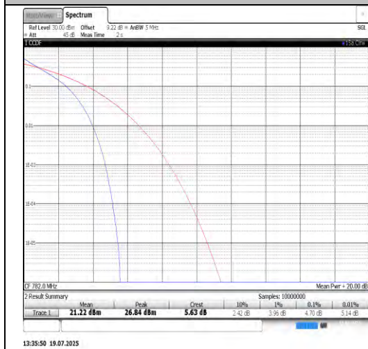
Band13-10MHz-QPSK-23230-50RB#0-PASS
