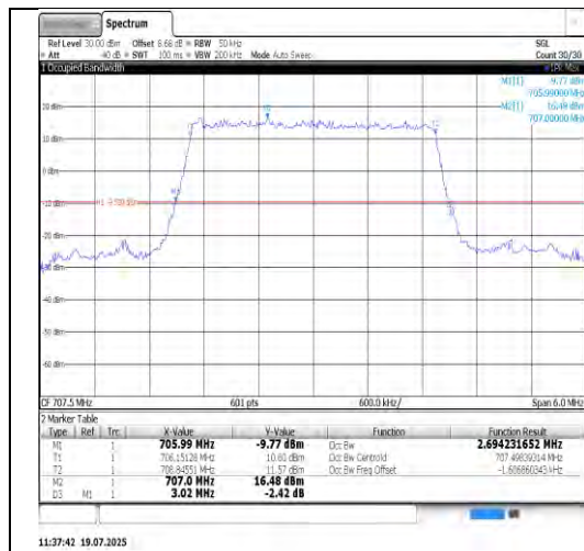
Band12-5MHz-QPSK-23095-25RB#0-PASS
