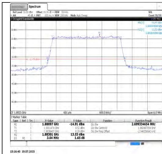
Band25-5MHz-16QAM-26365-25RB#0-PASS
