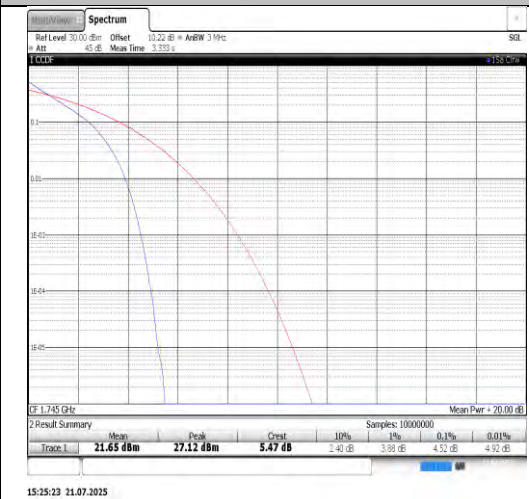
Band66-5MHz-QPSK-132322-25RB#0-PASS
