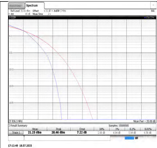
Band5-10MHz-16QAM-20525-50RB#0-PASS
