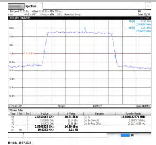
Band38-20MHz-QPSK-38000-100RB#0-PASS
