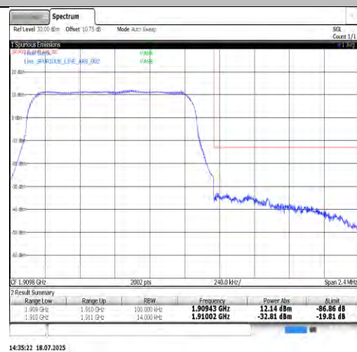
Band2-1.4MHz-16QAM-18607-1RB#5-PASS
