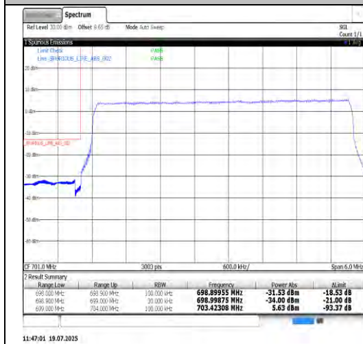
Band12-5MHz-16QAM-23155-1RB#24-PASS
