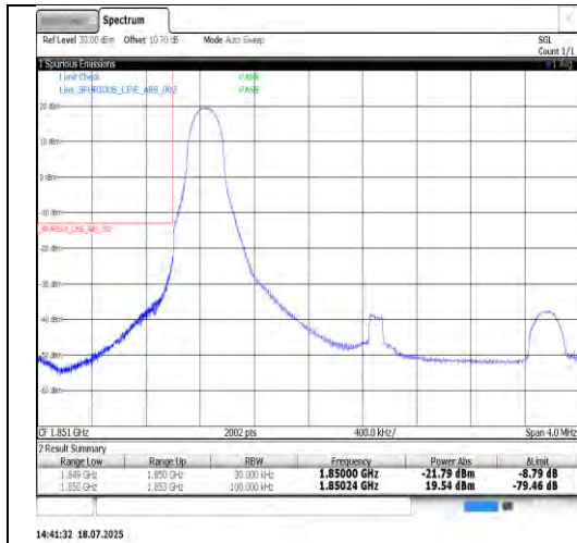
Band2-3MHz-16QAM-18615-15RB#0-PASS
