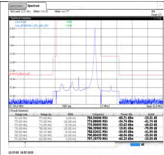
Band13-10MHz-16QAM-23230-1RB#0-PASS
