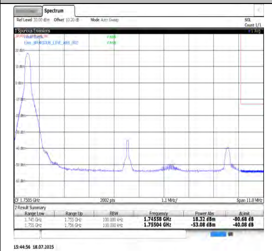
Band4-10MHz-16QAM-20350-50RB#0-PASS
