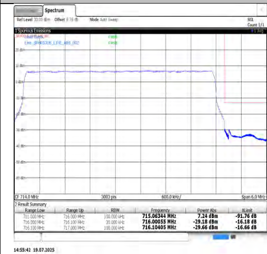
Band17-5MHz-16QAM-23755-1RB#24-PASS
