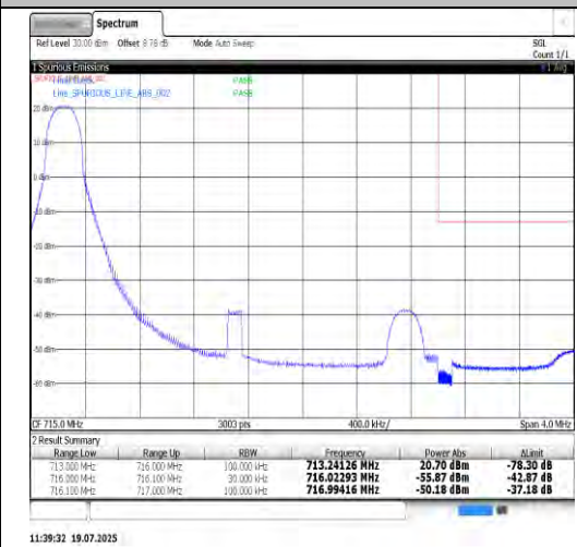
Band12-3MHz-16QAM-23165-15RB#0-PASS
