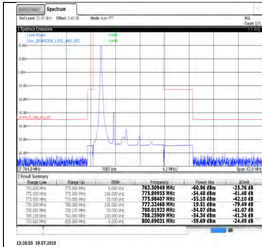
Band13-5MHz-16QAM-23205-25RB#0-PASS
