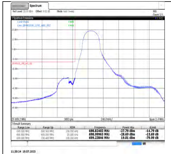
Band12-1.4MHz-QPSK-23017-6RB#0-PASS
