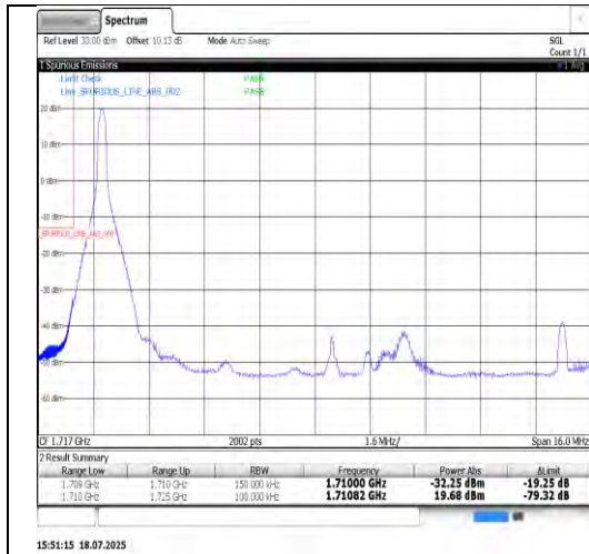
Band4-15MHz-QPSK-20025-75RB#0-PASS
