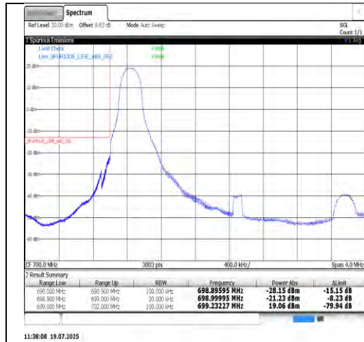
Band12-3MHz-QPSK-23025-15RB#0-PASS
