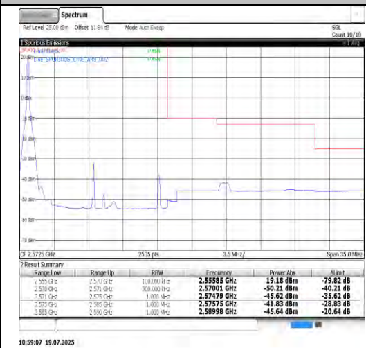
Band7-15MHz-16QAM-21375-75RB#0-PASS
