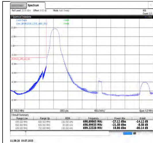
Band12-3MHz-16QAM-23025-15RB#0-PASS
