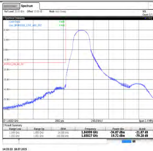
Band2-1.4MHz-QPSK-18607-6RB#0-PASS
