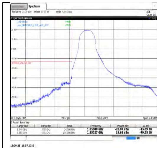
Band25-1.4MHz-QPSK-26047-6RB#0-PASS
