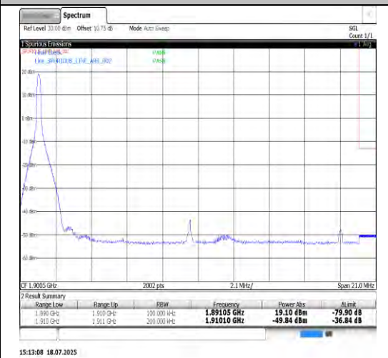
Band2-20MHz-16QAM-19100-100RB#0-PASS
