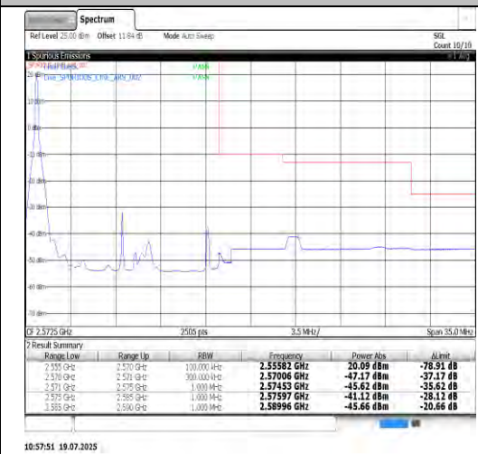
Band7-15MHz-QPSK-21375-75RB#0-PASS
