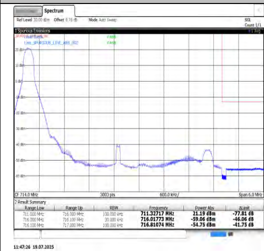
Band12-5MHz-16QAM-23155-25RB#0-PASS
