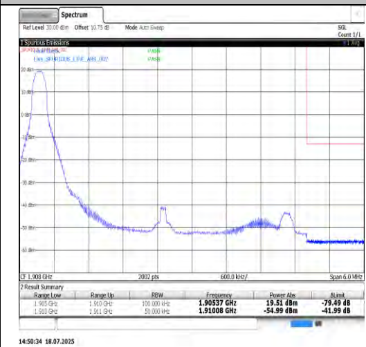
Band2-5MHz-16QAM-19175-25RB#0-PASS
