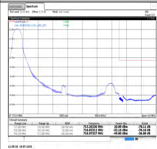
Band12-3MHz-QPSK-23165-15RB#0-PASS
