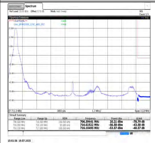
Band17-10MHz-QPSK-23800-50RB#0-PASS
