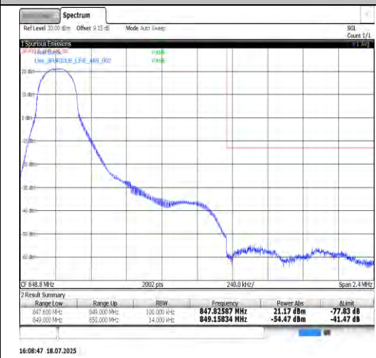
Band5-1.4MHz-QPSK-20643-6RB#0-PASS
