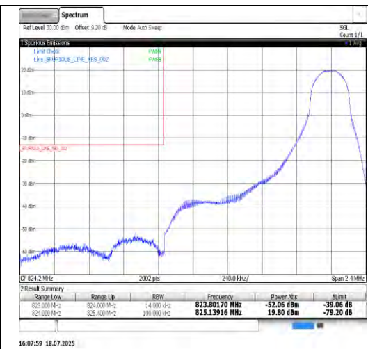
Band5-1.4MHz-QPSK-20643-1RB#0-PASS
