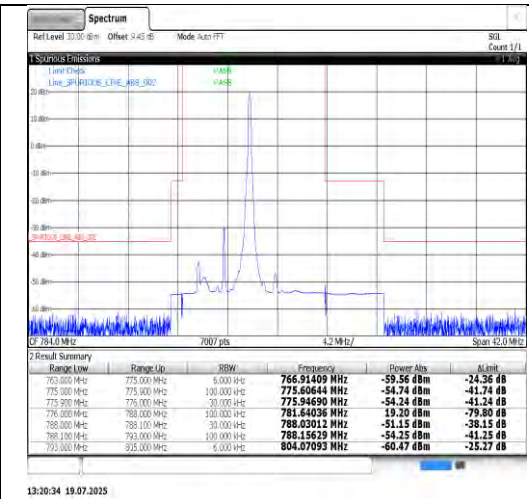
Band13-5MHz-16QAM-23255-1RB#0-PASS
