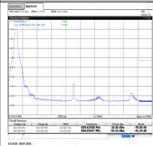
Band5-10MHz-16QAM-20600-50RB#0-PASS
