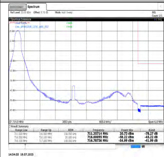
Band17-5MHz-QPSK-23825-25RB#0-PASS
