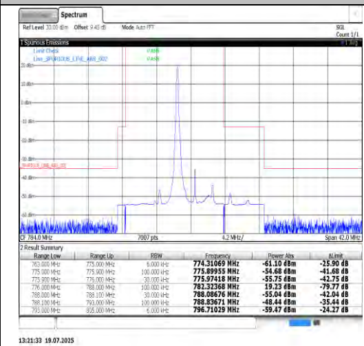
Band13-5MHz-16QAM-23255-25RB#0-PASS
