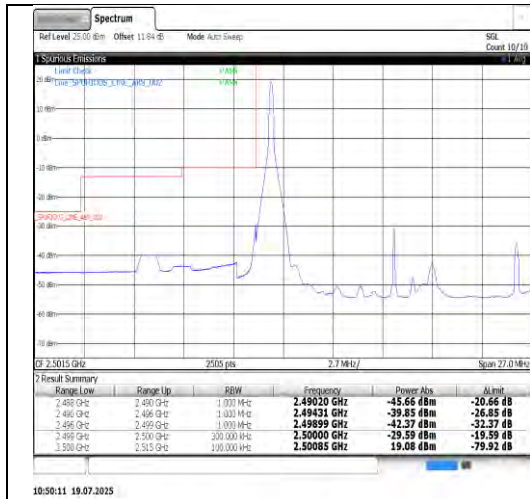
Band7-15MHz-QPSK-20825-75RB#0-PASS
