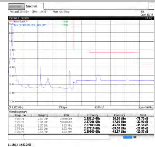
Band7-20MHz-QPSK-21350-100RB#0-PASS
