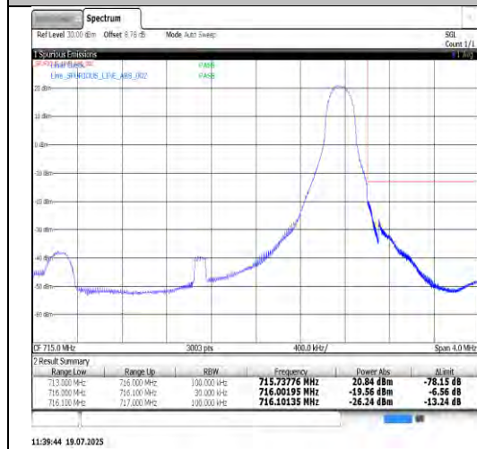
Band12-3MHz-16QAM-23025-1RB#0-PASS
