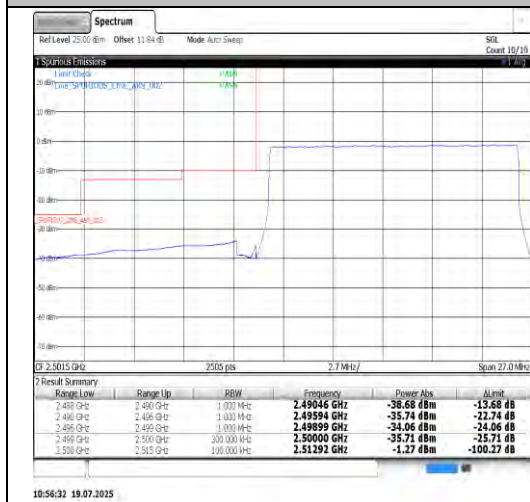
Band7-15MHz-16QAM-21375-1RB#74-PASS
