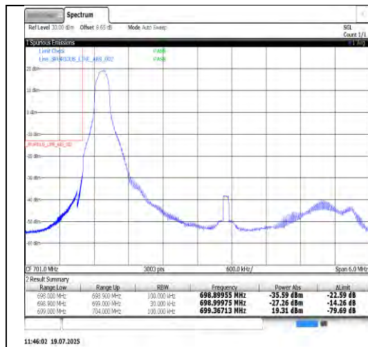
Band12-5MHz-QPSK-23035-25RB#0-PASS
