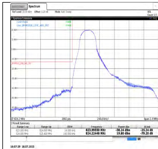
Band5-1.4MHz-QPSK-20407-6RB#0-PASS
