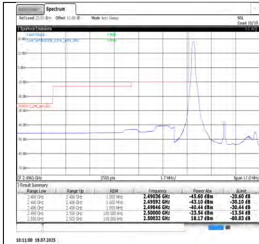
Band7-5MHz-16QAM-20775-25RB#0-PASS
