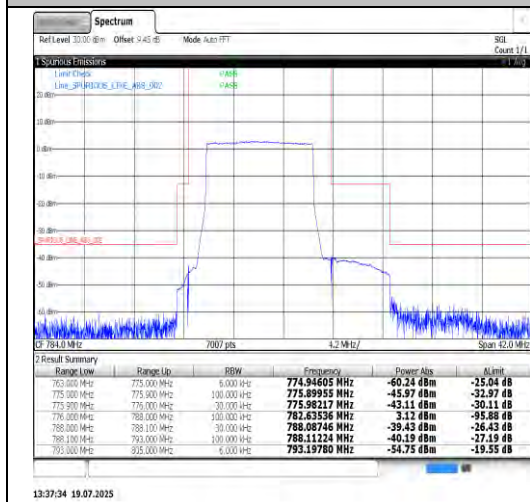
Band13-10MHz-16QAM-23230-1RB#49-PASS
