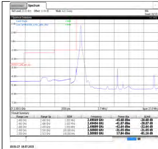
Band7-15MHz-16QAM-20825-75RB#0-PASS
