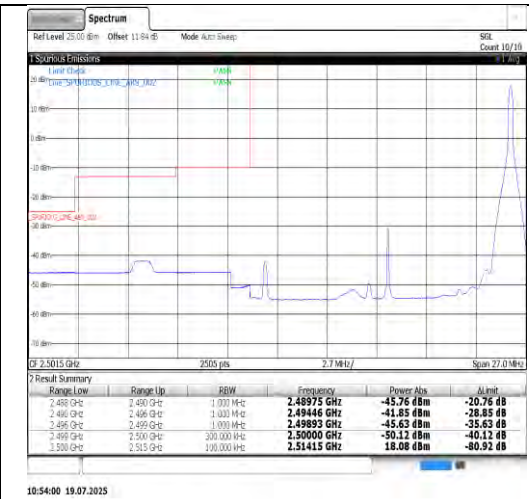
Band7-15MHz-16QAM-21375-1RB#0-PASS
