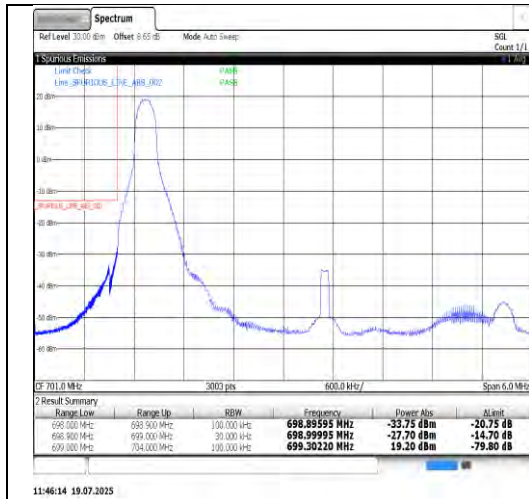
Band12-5MHz-16QAM-23035-25RB#0-PASS
