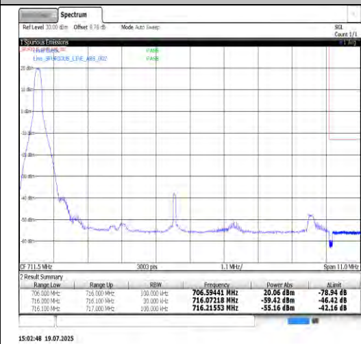
Band17-10MHz-16QAM-23800-50RB#0-PASS
