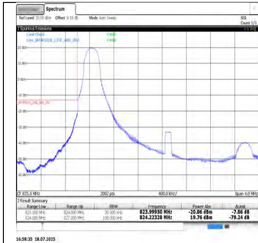
Band5-3MHz-QPSK-20415-15RB#0-PASS
