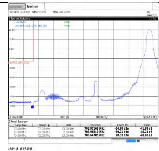
Band17-5MHz-16QAM-23825-1RB#0-PASS
