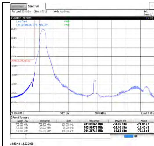
Band17-5MHz-QPSK-23755-25RB#0-PASS
