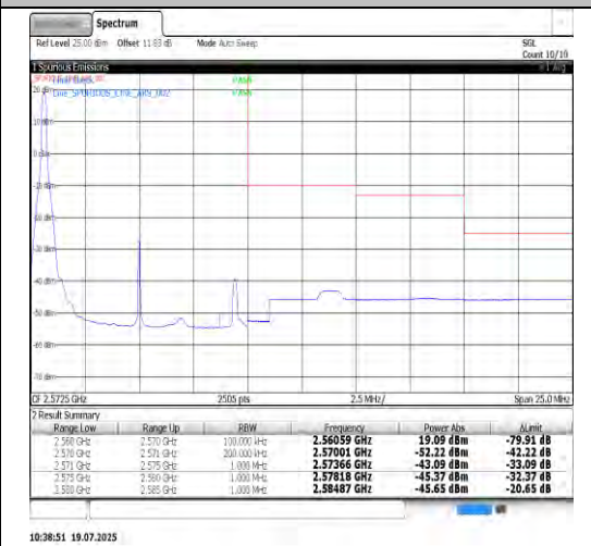
Band7-10MHz-16QAM-21400-50RB#0-PASS
