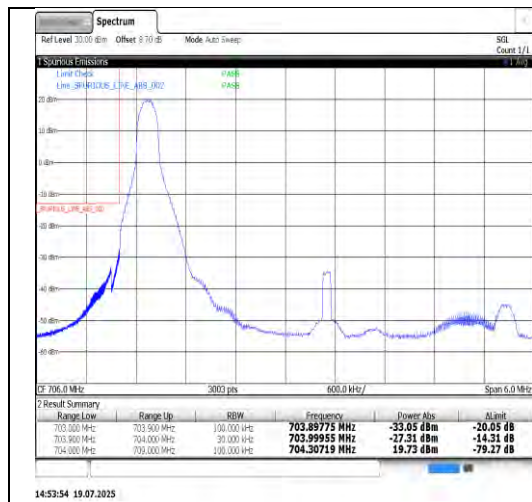
Band17-5MHz-16QAM-23755-25RB#0-PASS
