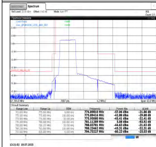
Band13-5MHz-16QAM-23255-1RB#24-PASS
