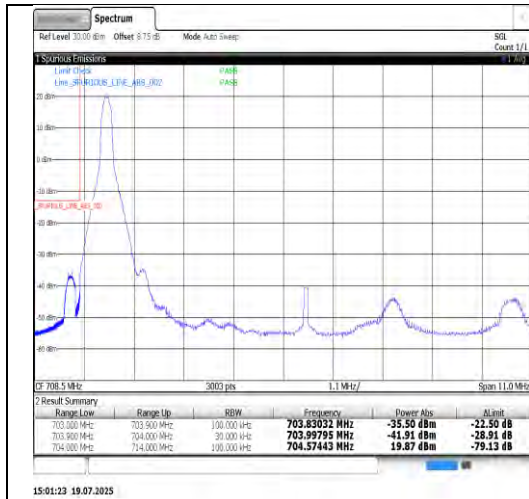
Band17-10MHz-QPSK-23780-50RB#0-PASS
