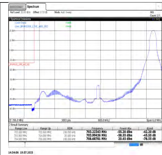
Band17-5MHz-QPSK-23825-1RB#0-PASS
