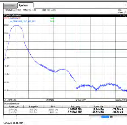
Band2-1.4MHz-QPSK-19193-6RB#0-PASS
