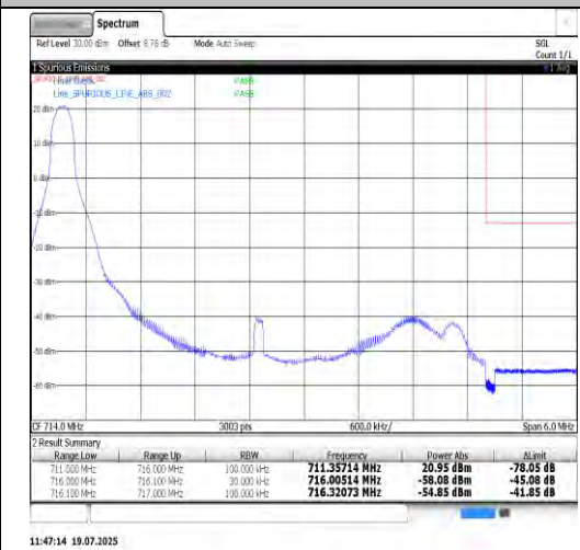
Band12-5MHz-QPSK-23155-25RB#0-PASS
