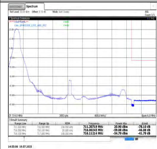
Band17-5MHz-16QAM-23825-25RB#0-PASS
