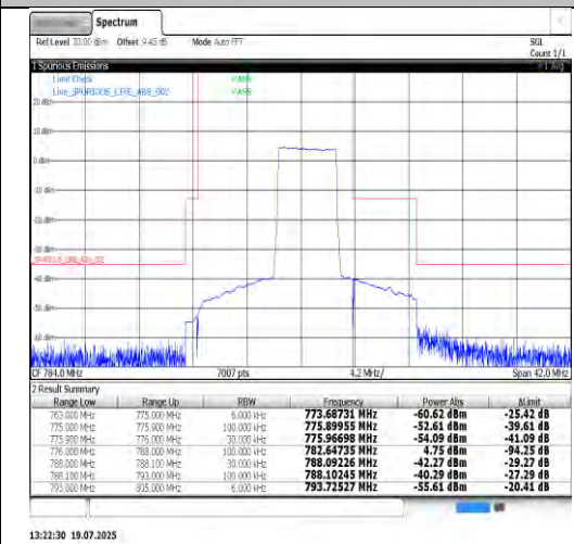
Band13-10MHz-QPSK-23230-1RB#49-PASS
