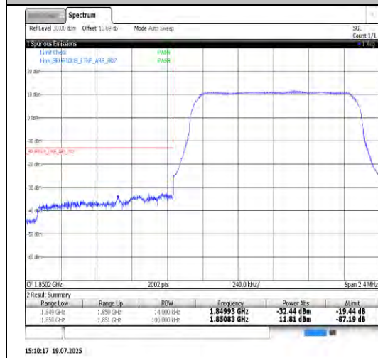
Band25-1.4MHz-QPSK-26683-1RB#5-PASS
