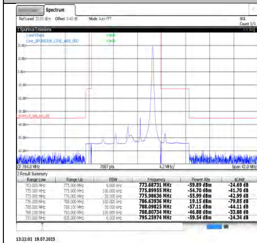
Band13-10MHz-QPSK-23230-1RB#0-PASS
