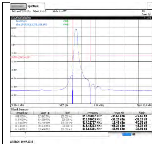
Band26(814-824)-1.4MHz-QPSK-26697-6RB#0-PASS
