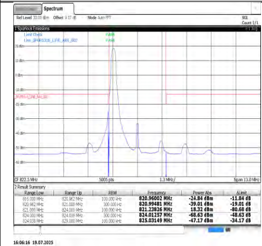
Band26(814-824)-3MHz-16QAM-26775-15RB#0-PASS
