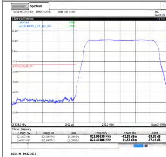
Band26(824-849)-1.4MHz-QPSK-27033-1RB#5-PASS
