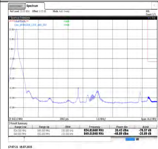
Band26(824-849)-15MHz-QPSK-26965-75RB#0-PASS
