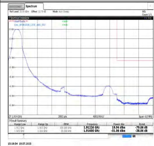
Band25-3MHz-QPSK-26675-15RB#0-PASS
