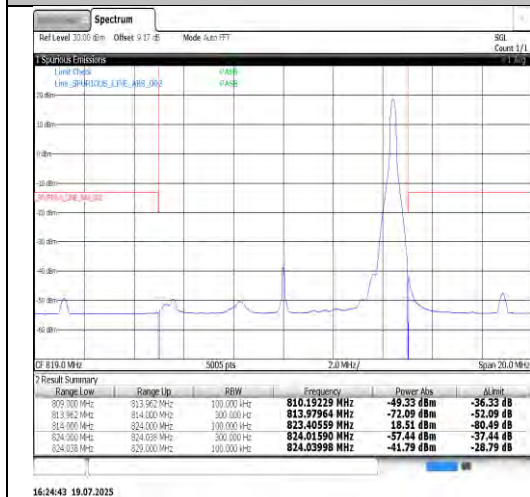
Band26(824-849)-1.4MHz-QPSK-26797-1RB#0-PASS
