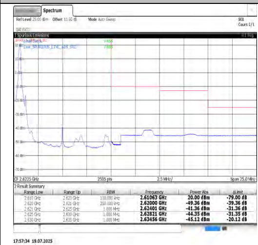
Band38-10MHz-QPSK-38200-50RB#0-PASS
