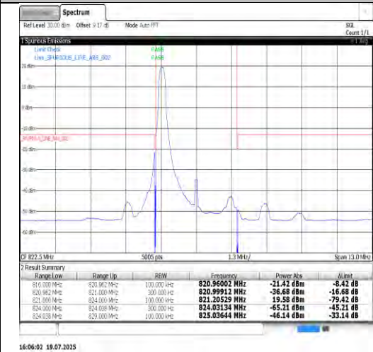
Band26(814-824)-3MHz-QPSK-26775-15RB#0-PASS
