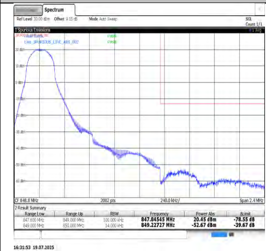
Band26(824-849)-1.4MHz-16QAM-27033-6RB#0-PASS
