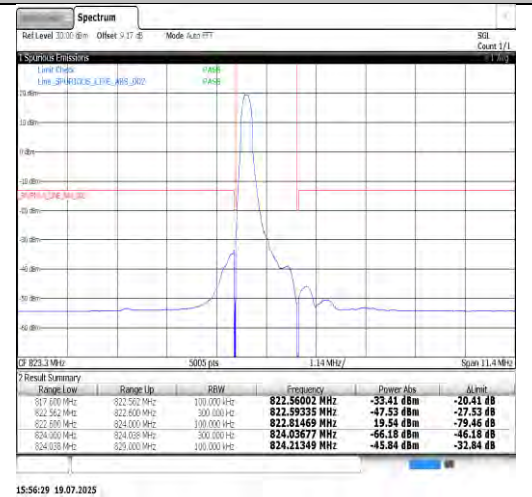
Band26(814-824)-1.4MHz-QPSK-26783-6RB#0-PASS
