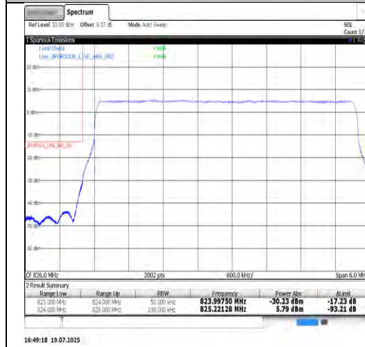
Band26(824-849)-5MHz-QPSK-27015-1RB#24-PASS
