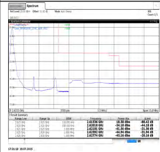
Band38-5MHz-16QAM-38225-25RB#0-PASS
