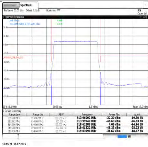
Band26(814-824)-5MHz-QPSK-26765-1RB#24-PASS
