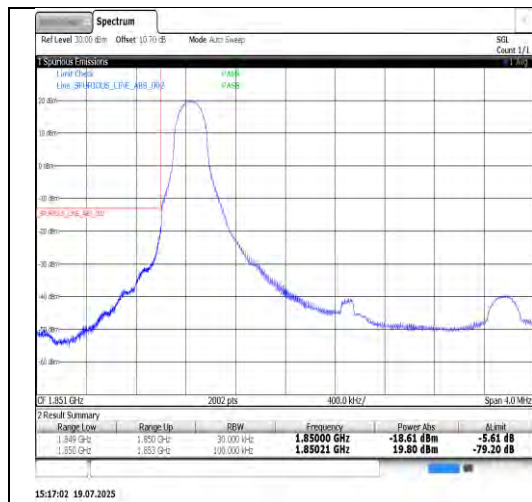
Band25-3MHz-QPSK-26055-15RB#0-PASS
