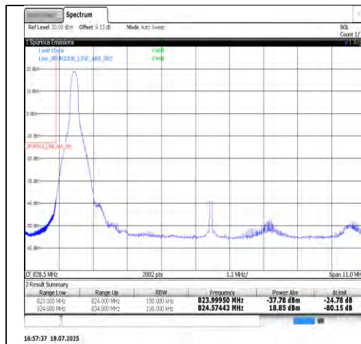
Band26(824-849)-10MHz-16QAM-26840-50RB#0-PASS
