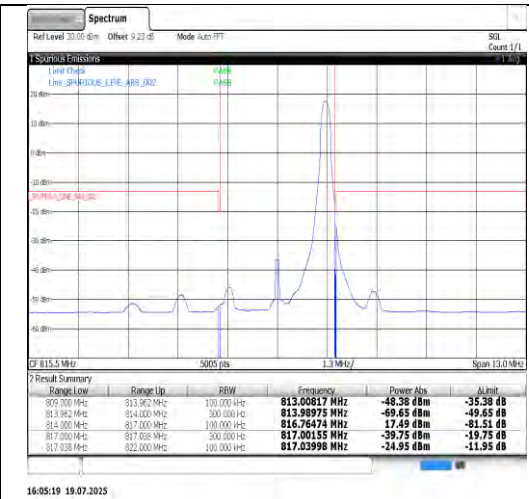
Band26(814-824)-3MHz-16QAM-26775-1RB#0-PASS
