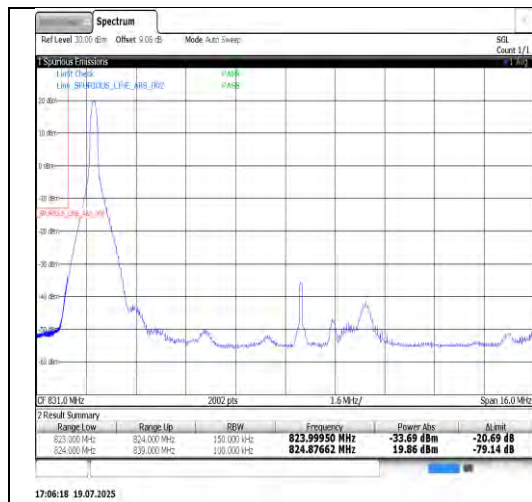
Band26(824-849)-15MHz-QPSK-26865-75RB#0-PASS
