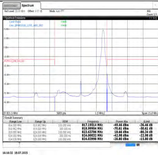
Band26(814-824)-10MHz-QPSK-26740-1RB#0-PASS
