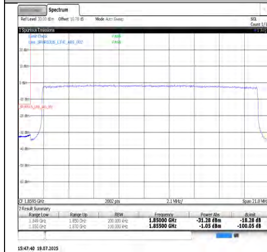
Band25-20MHz-16QAM-26140-100RB#0-PASS
