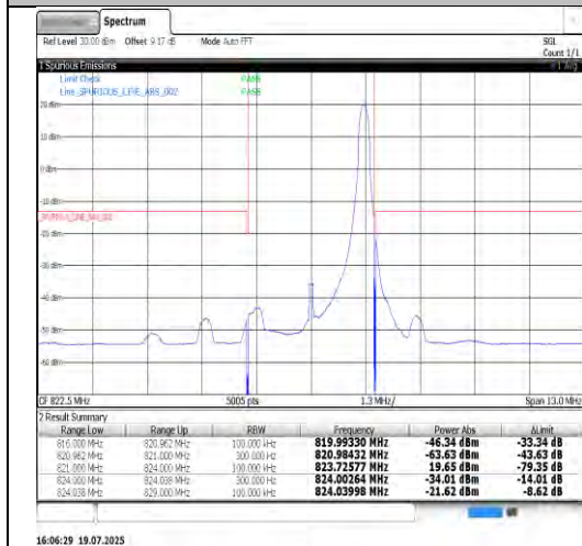
Band26(814-824)-3MHz-16QAM-26705-1RB#0-PASS
