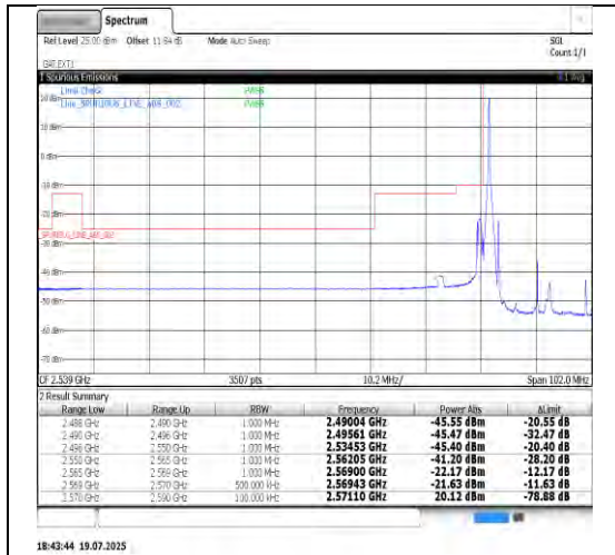
Band38-20MHz-QPSK-37850-100RB#0-PASS
