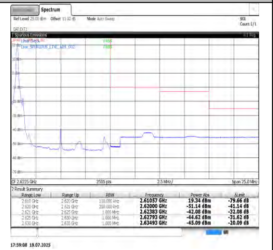
Band38-10MHz-16QAM-38200-50RB#0-PASS
