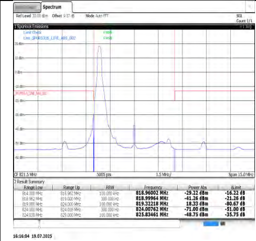
Band26(814-824)-5MHz-16QAM-26765-25RB#0-PASS
