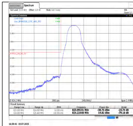
Band26(824-849)-1.4MHz-QPSK-26797-6RB#0-PASS
