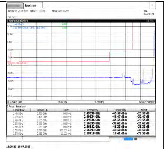
Band38-15MHz-16QAM-38175-1RB#0-PASS
