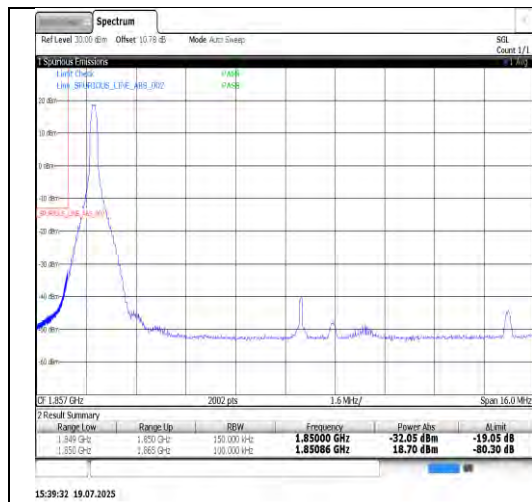
Band25-15MHz-16QAM-26115-75RB#0-PASS
