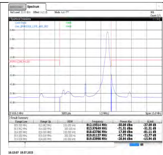
Band26(814-824)-5MHz-16QAM-26765-1RB#0-PASS
