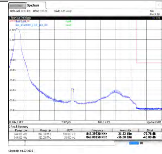
Band26(824-849)-5MHz-QPSK-27015-25RB#0-PASS
