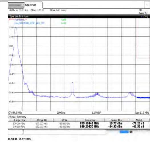
Band26(824-849)-10MHz-16QAM-26990-50RB#0-PASS
