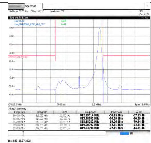
Band26(814-824)-5MHz-QPSK-26765-1RB#0-PASS
