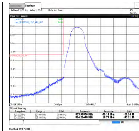
Band26(824-849)-1.4MHz-16QAM-26797-6RB#0-PASS
