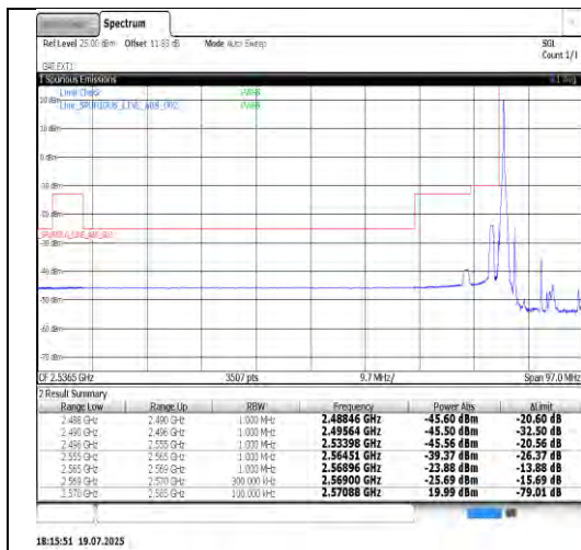
Band38-15MHz-QPSK-37825-75RB#0-PASS
