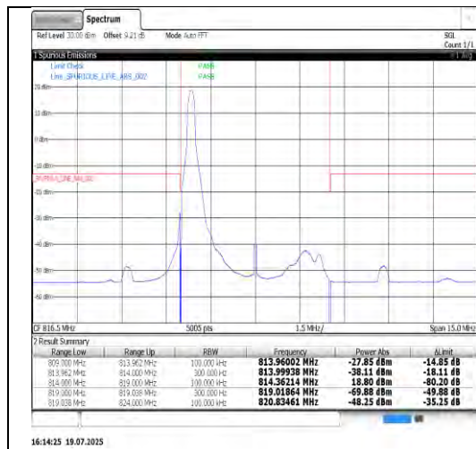
Band26(814-824)-5MHz-QPSK-26715-25RB#0-PASS
