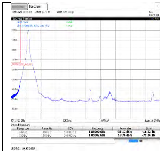
Band25-15MHz-QPSK-26115-75RB#0-PASS
