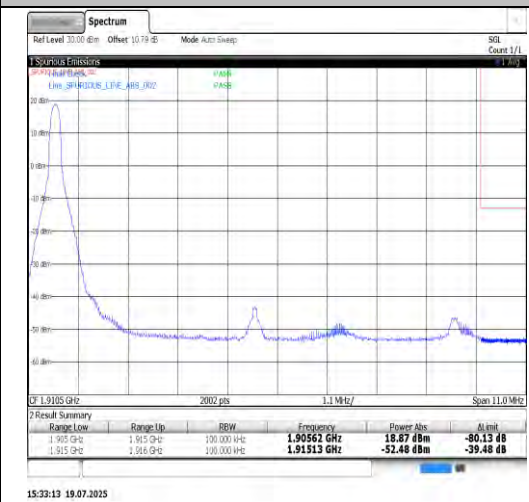
Band25-10MHz-16QAM-26640-50RB#0-PASS
