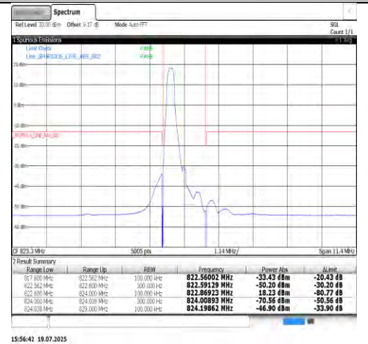
Band26(814-824)-1.4MHz-16QAM-26783-6RB#0-PASS
