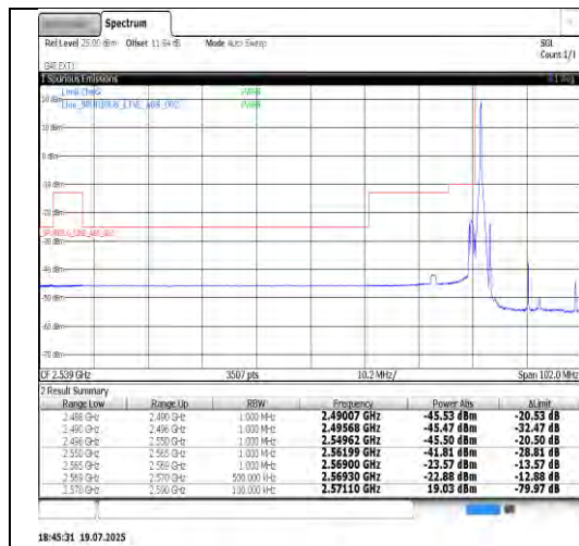
Band38-20MHz-16QAM-37850-100RB#0-PASS
