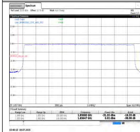
Band25-15MHz-16QAM-26615-1RB#74-PASS
