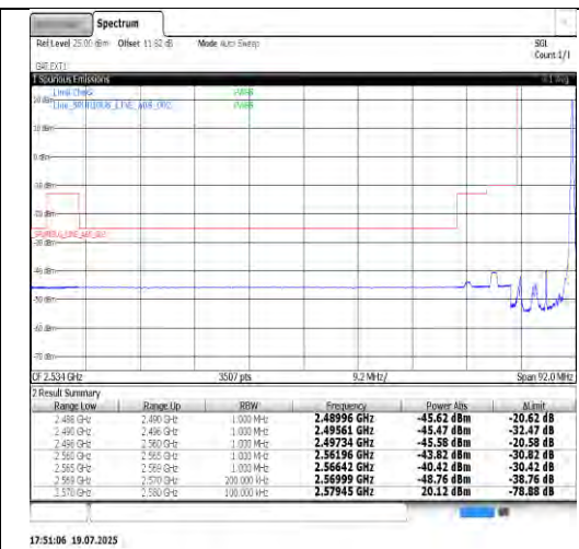
Band38-10MHz-QPSK-38200-1RB#0-PASS
