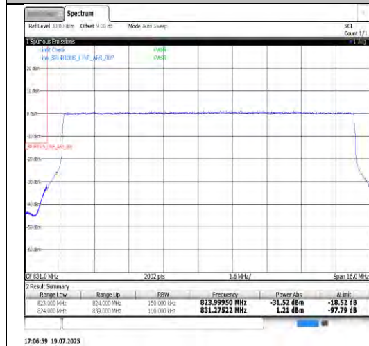
Band26(824-849)-15MHz-QPSK-26965-1RB#74-PASS
