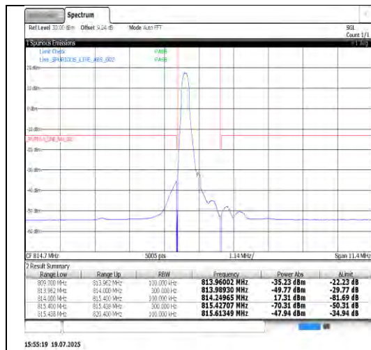
Band26(814-824)-1.4MHz-16QAM-26697-6RB#0-PASS
