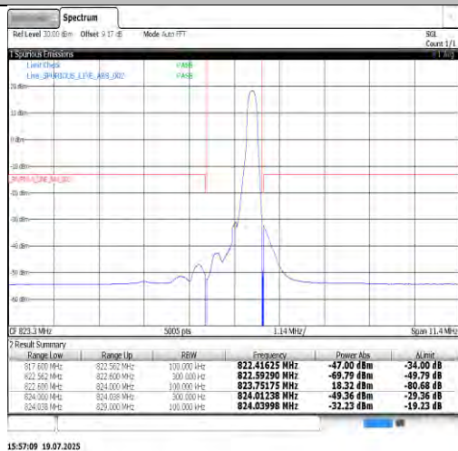
Band26(814-824)-3MHz-QPSK-26705-1RB#0-PASS
