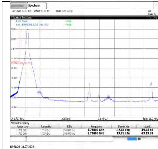
Band66-15MHz-16QAM-132047-75RB#0-PASS
