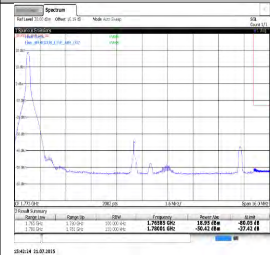
Band66-15MHz-16QAM-132597-75RB#0-PASS
