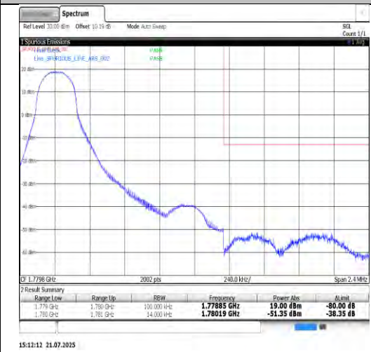
Band66-1.4MHz-16QAM-132665-6RB#0-PASS
