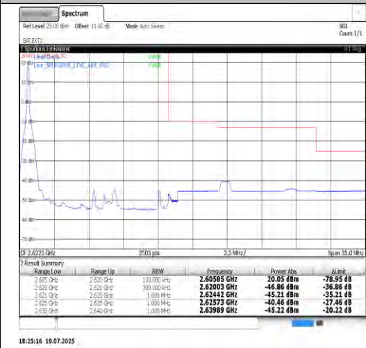
Band38-15MHz-QPSK-38175-75RB#0-PASS
