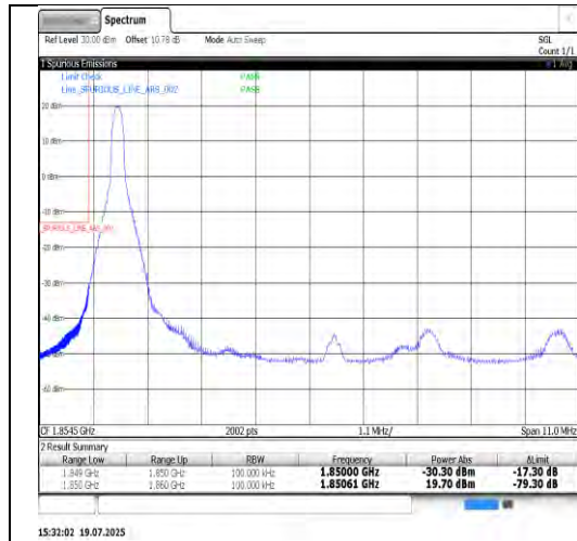
Band25-10MHz-QPSK-26090-50RB#0-PASS
