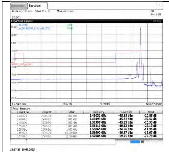
Band38-15MHz-16QAM-37825-75RB#0-PASS
