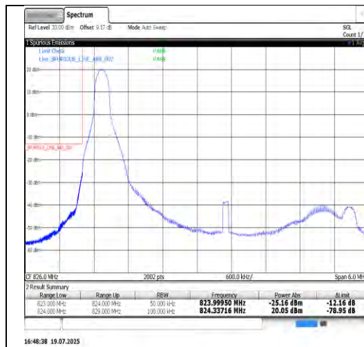
Band26(824-849)-5MHz-QPSK-26815-25RB#0-PASS
