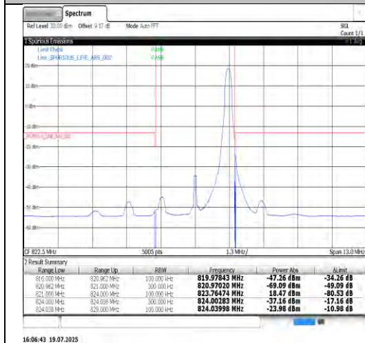
Band26(814-824)-5MHz-QPSK-26715-1RB#0-PASS
