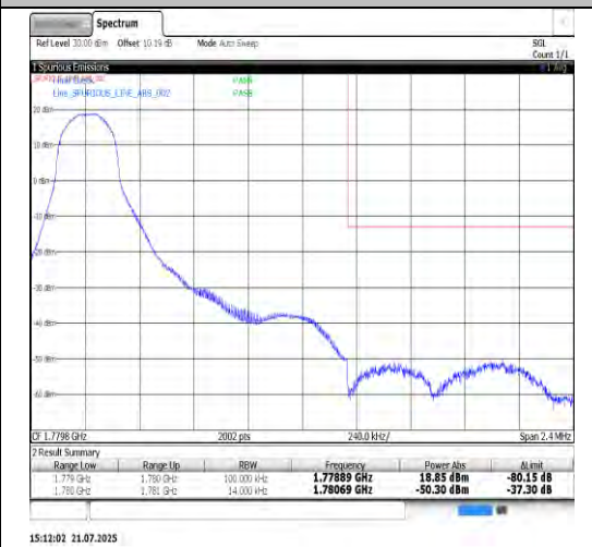
Band66-1.4MHz-QPSK-132665-6RB#0-PASS
