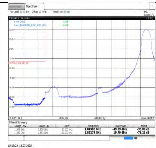
Band25-3MHz-QPSK-26675-1RB#0-PASS
