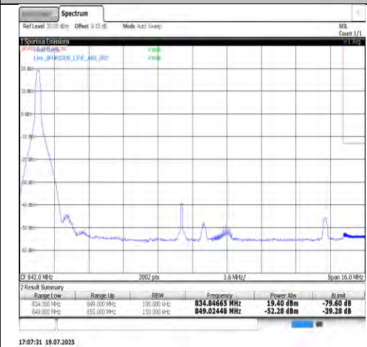
Band26(824-849)-15MHz-16QAM-26965-75RB#0-PASS
