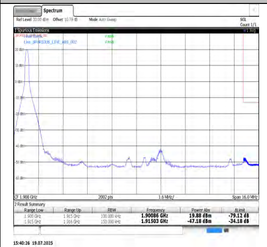
Band25-15MHz-QPSK-26615-75RB#0-PASS
