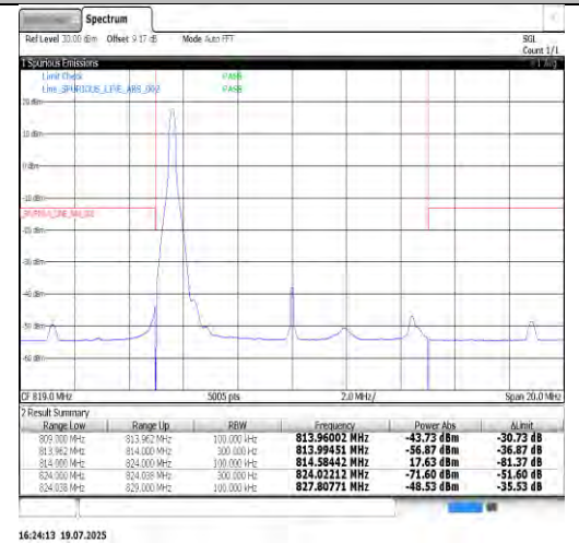
Band26(814-824)-10MHz-16QAM-26740-50RB#0-PASS
