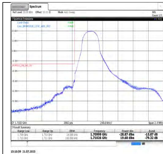
Band66-1.4MHz-QPSK-131979-6RB#0-PASS
