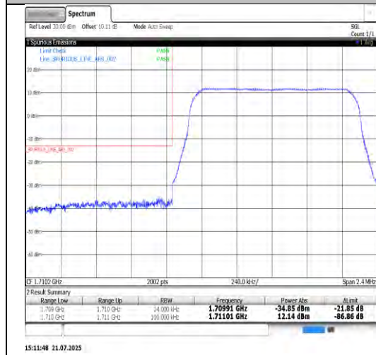
Band66-1.4MHz-16QAM-132665-1RB#5-PASS
