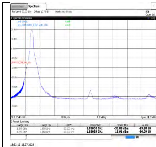
Band25-10MHz-16QAM-26090-50RB#0-PASS
