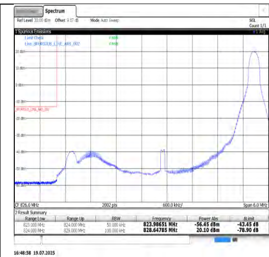
Band26(824-849)-5MHz-QPSK-27015-1RB#0-PASS
