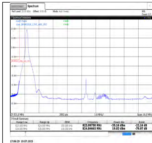
Band26(824-849)-15MHz-16QAM-26865-75RB#0-PASS
