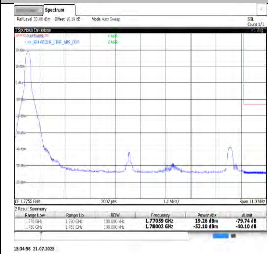
Band66-10MHz-16QAM-132622-50RB#0-PASS
