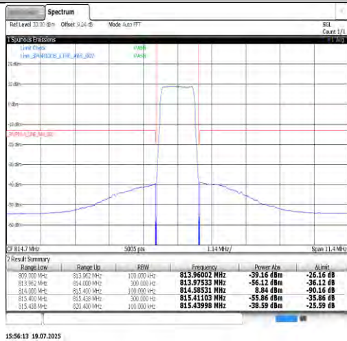
Band26(814-824)-1.4MHz-16QAM-26783-1RB#5-PASS
