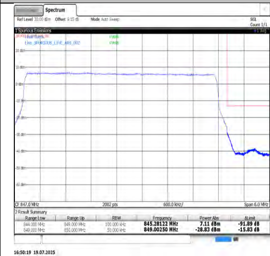
Band26(824-849)-5MHz-16QAM-26815-1RB#24-PASS
