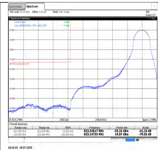
Band26(824-849)-1.4MHz-QPSK-27033-1RB#0-PASS
