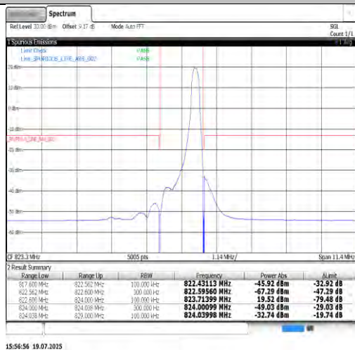
Band26(814-824)-1.4MHz-16QAM-26697-1RB#0-PASS
