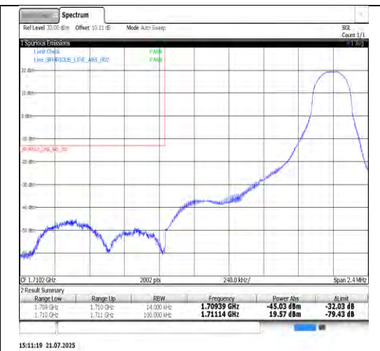
Band66-1.4MHz-QPSK-132665-1RB#0-PASS
