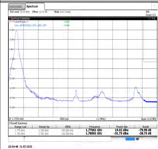
Band66-10MHz-QPSK-132622-50RB#0-PASS
