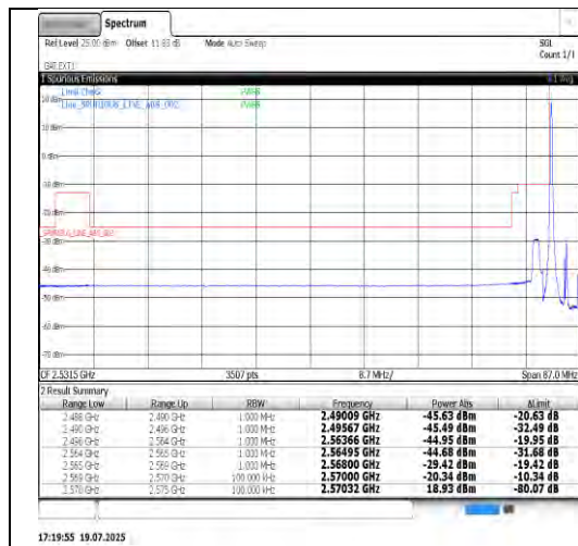
Band38-5MHz-16QAM-37775-25RB#0-PASS
