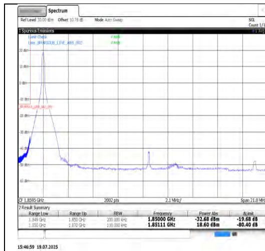
Band25-20MHz-16QAM-26140-100RB#0-PASS
