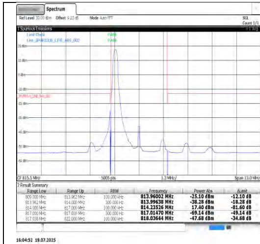
Band26(814-824)-3MHz-16QAM-26705-15RB#0-PASS
