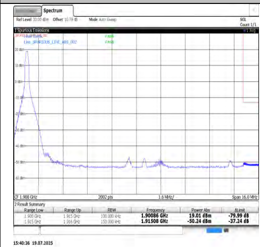
Band25-15MHz-16QAM-26615-75RB#0-PASS
