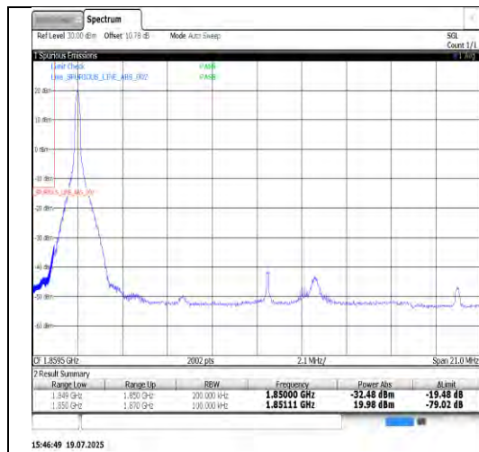
Band25-20MHz-QPSK-26140-100RB#0-PASS
