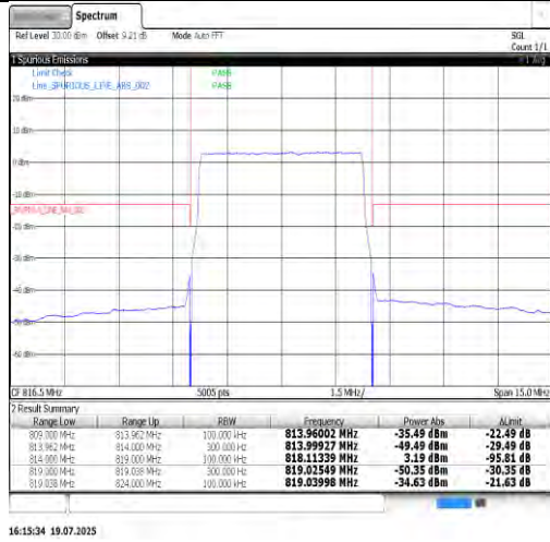
Band26(814-824)-5MHz-16QAM-26765-1RB#24-PASS
