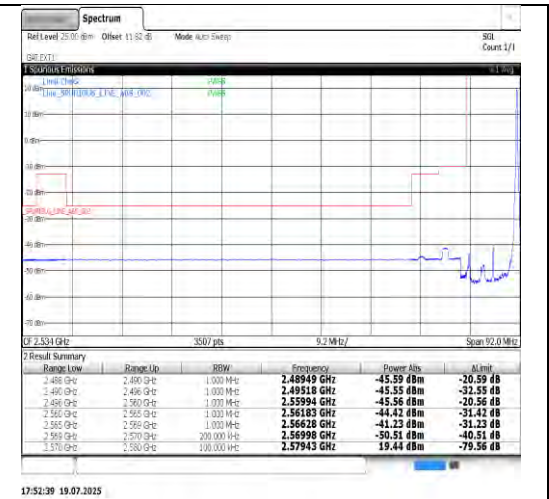
Band38-10MHz-16QAM-38200-1RB#0-PASS
