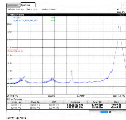
Band26(824-849)-10MHz-16QAM-26990-1RB#0-PASS
