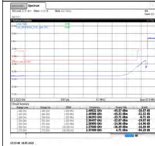
Band38-5MHz-16QAM-38225-1RB#24-PASS
