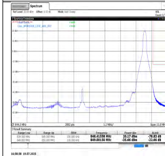
Band26(824-849)-15MHz-QPSK-26865-1RB#0-PASS
