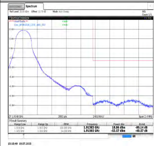
Band25-1.4MHz-16QAM-26683-6RB#0-PASS
