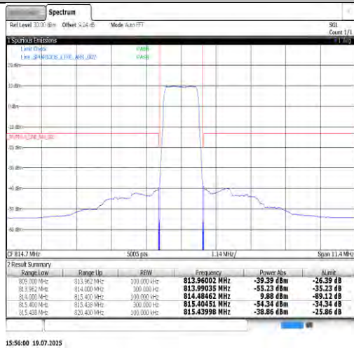
Band26(814-824)-1.4MHz-QPSK-26783-1RB#5-PASS
