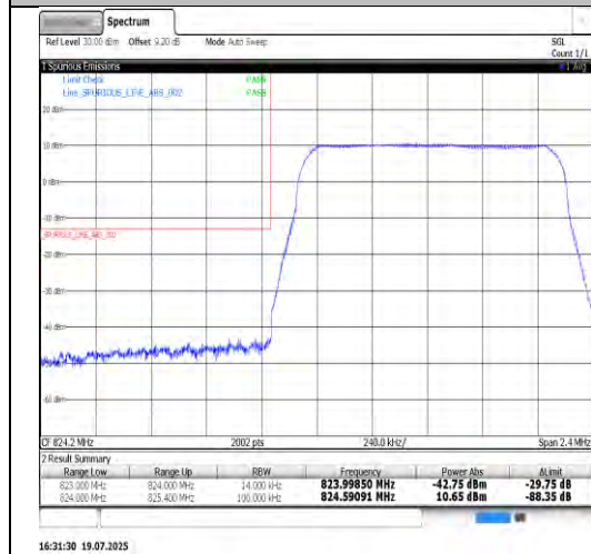
Band26(824-849)-1.4MHz-16QAM-27033-1RB#5-PASS
