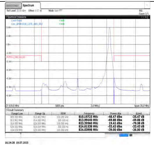
Band26(814-824)-10MHz-16QAM-26740-1RB#0-PASS
