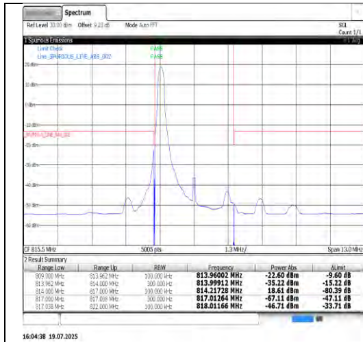
Band26(814-824)-3MHz-QPSK-26705-15RB#0-PASS
