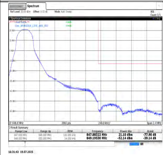
Band26(824-849)-1.4MHz-QPSK-27033-6RB#0-PASS
