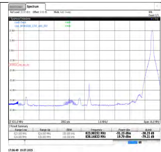
Band26(824-849)-15MHz-16QAM-26965-1RB#0-PASS
