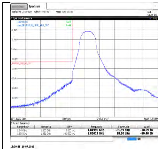
Band25-1.4MHz-16QAM-26047-6RB#0-PASS
