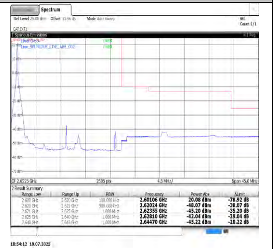
Band38-20MHz-QPSK-38150-100RB#0-PASS
