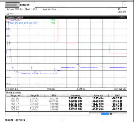
Band38-15MHz-16QAM-38175-75RB#0-PASS
