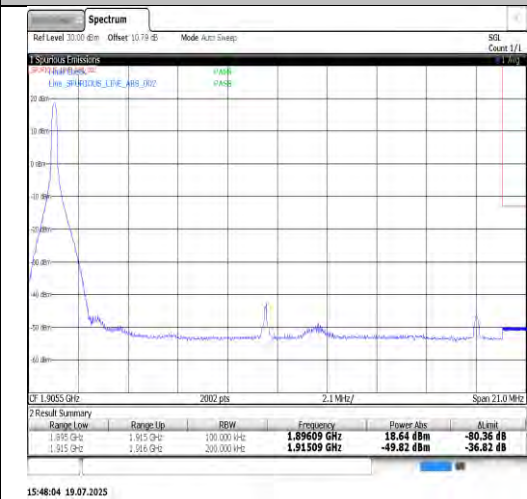
Band25-20MHz-16QAM-26590-100RB#0-PASS
