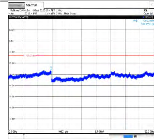
Band4-3MHz-QPSK-19965-1RB#0- 3000~20000-PASS
