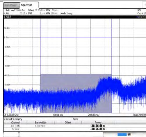
Band4-3MHz-QPSK-19965-1RB#0- 1000~3000-PASS
