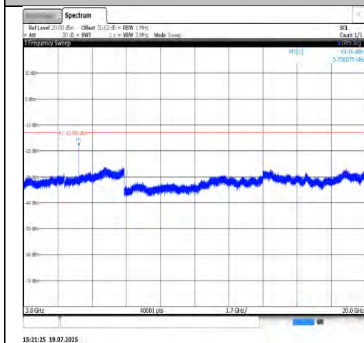
Band25-3MHz-16QAM-26055-1RB#0-1000~3000-PASS
