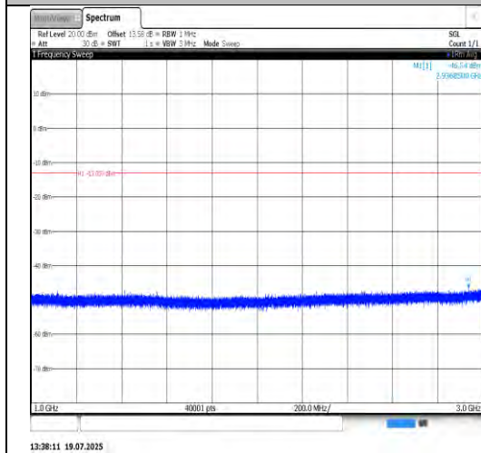
Band13-10MHz-QPSK-23230-1RB#49- 30~1000-PASS
