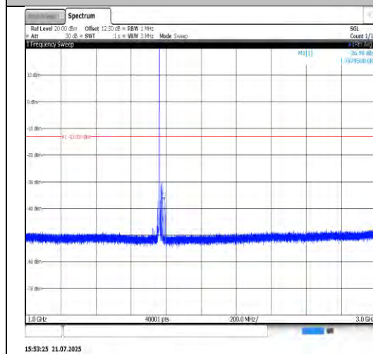
Band66-20MHz-16QAM-132572-1RB#0- 1000~3000-PASS
