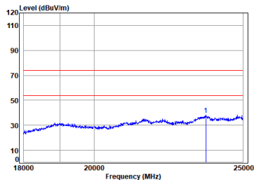
BT_DH5_TX_CH_00_Horizontal
