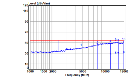
BT_DH5_TX_CH_00_Horizontal
