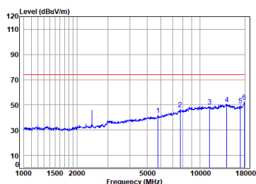
BLE_2M_TX_CH_19_Vertical-Peak
