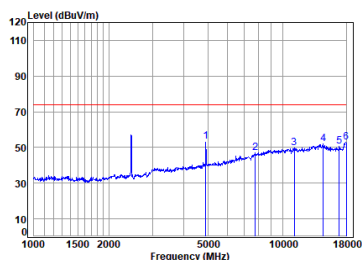
11b_TX_CH_11_Horizontal-Peak
