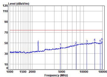
11n_20M_TX_CH_01_Horizontal-Peak
