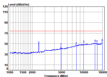
11g_TX_CH_11_Horizontal-Peak
