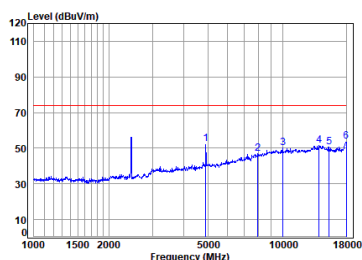
11b_TX_CH_11_Vertical-Peak
