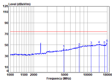
11g_TX_CH_11_Vertical-Peak
