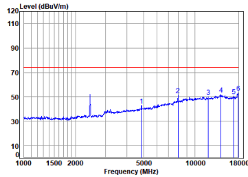
11g_TX_CH_06_Vertical-Peak
