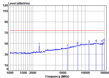
11n_20M_TX_CH_06_Vertical-Peak
