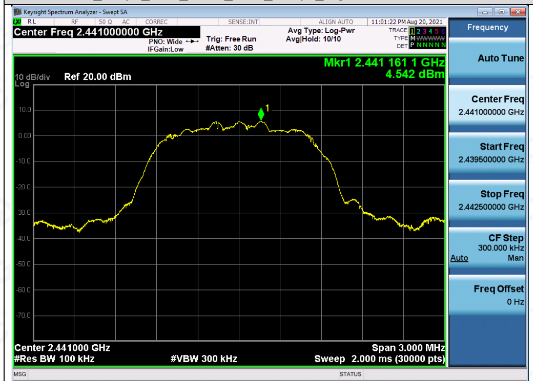
Test_Graph_EDR_ANT1_2441_3Mbps_Reference Level
