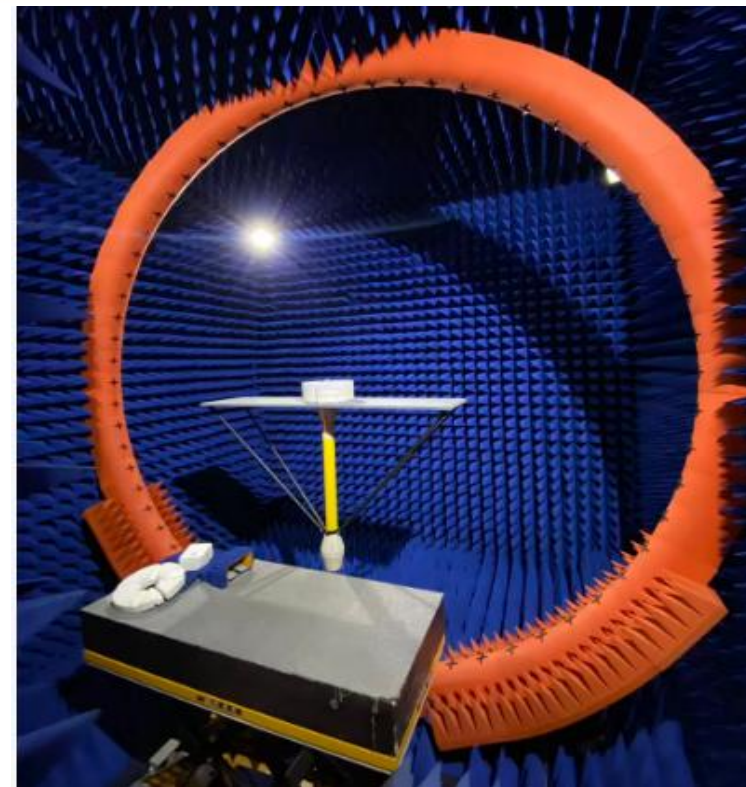
Testing 3D microwave darkroom(6m*6m*6m)
