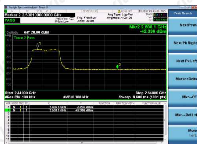
Right bandedge
