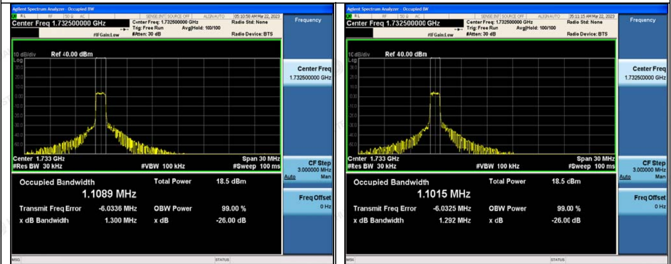
Low Channel
