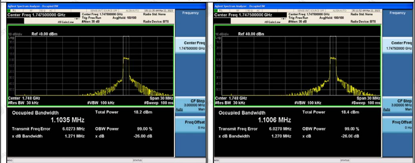
Middle Channel
