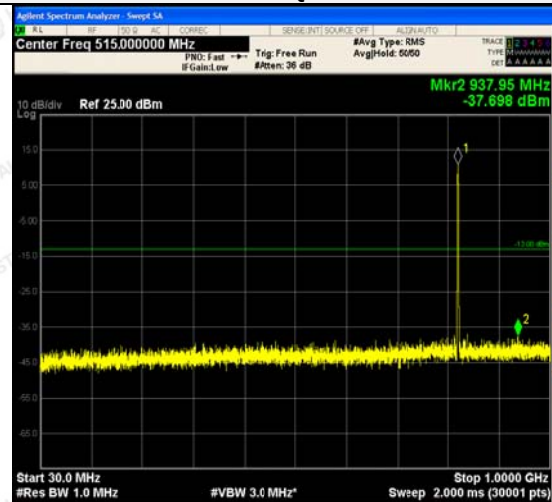
30MHz~1GHz
