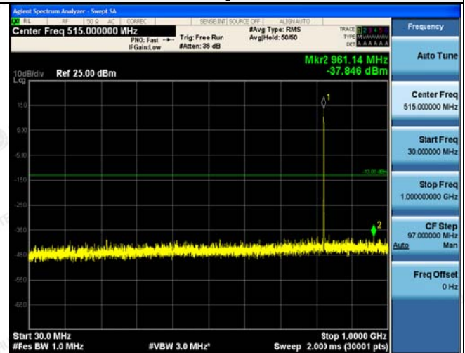
30MHz~1GHz
