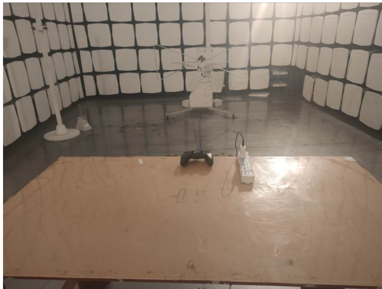
Test Setup Photo for Radiated Emissions (Below 1GHz)
