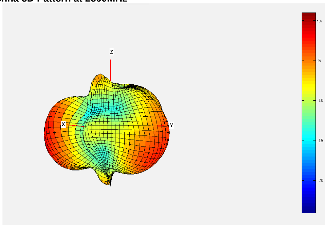
Antenna 3D Pattern at 2500MHz
