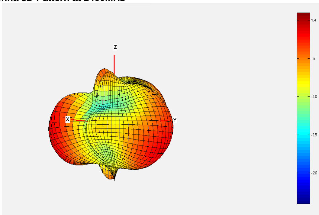
Antenna 3D Pattern at 2460MHz
