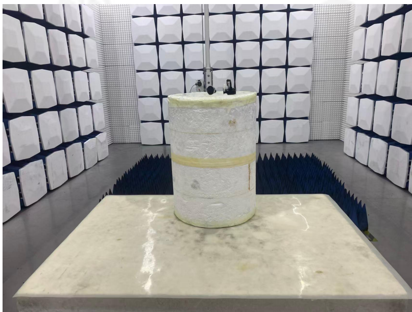
Radiated Emission (18GHz-25GHz)
