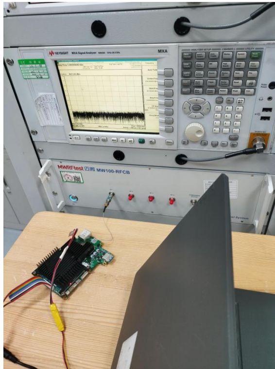
Photograph 3: Set-up photo for RF Conducted Test
