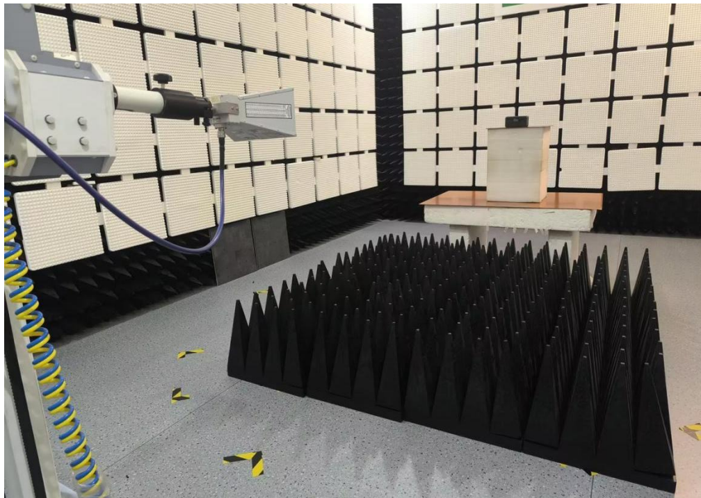
Photograph 2: Set-up photo for Radiated Spurious Emission, above 1GHz
