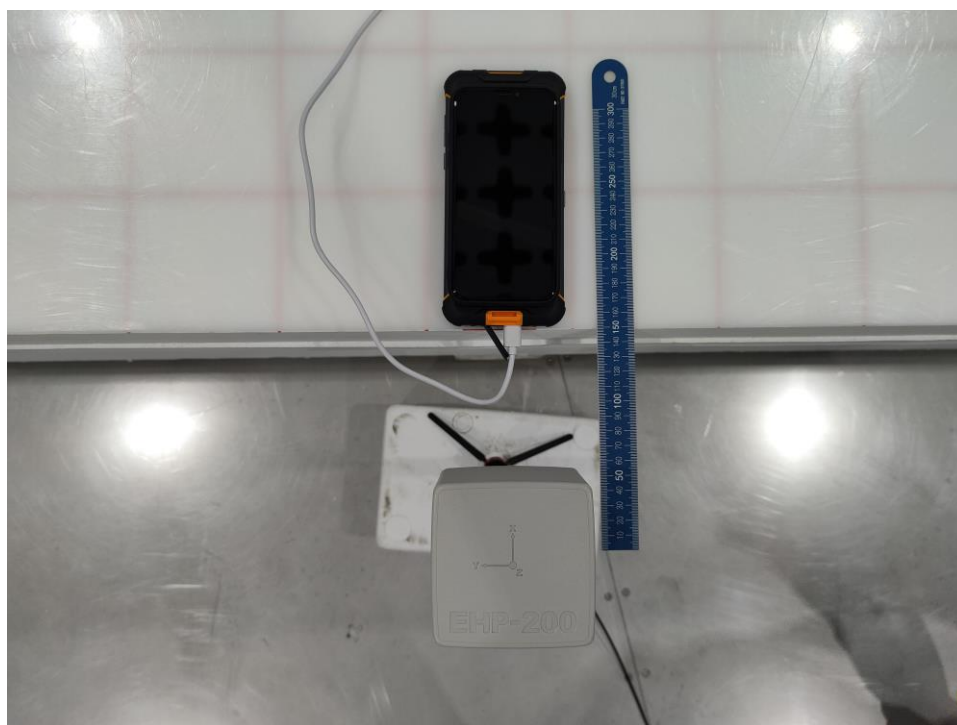
Test setup of D side
