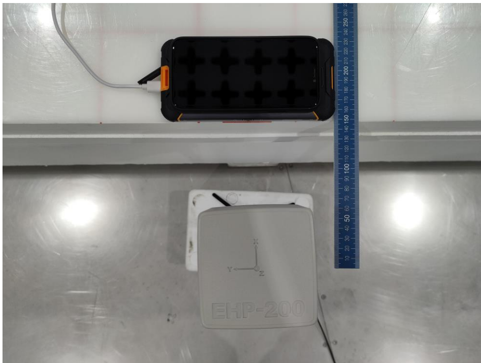
Test setup of B side
