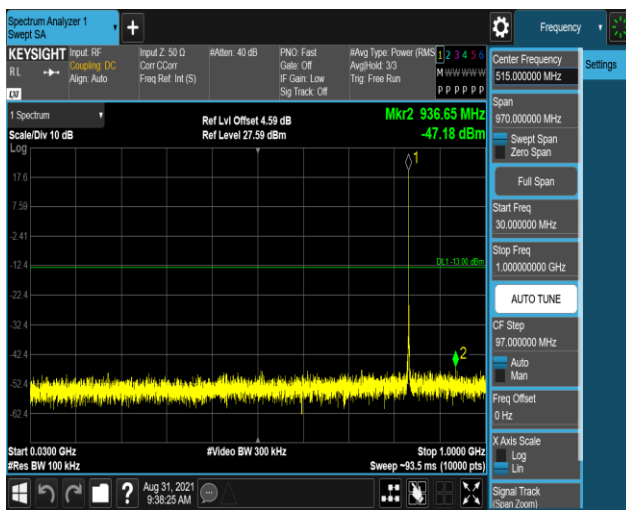
Band26-1.4MHz-QPSK-27033-1RB#0-Range1:30~1000MHz
