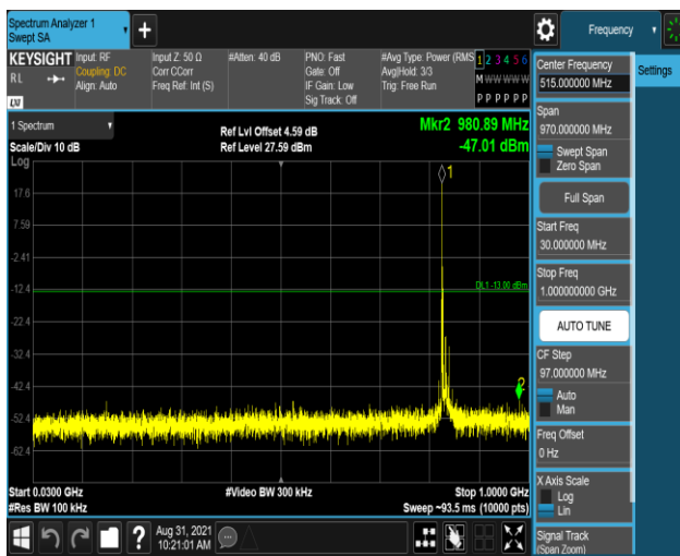
Band26-15MHz-QPSK-26965-1RB#0-Range1:30~1000MHz
