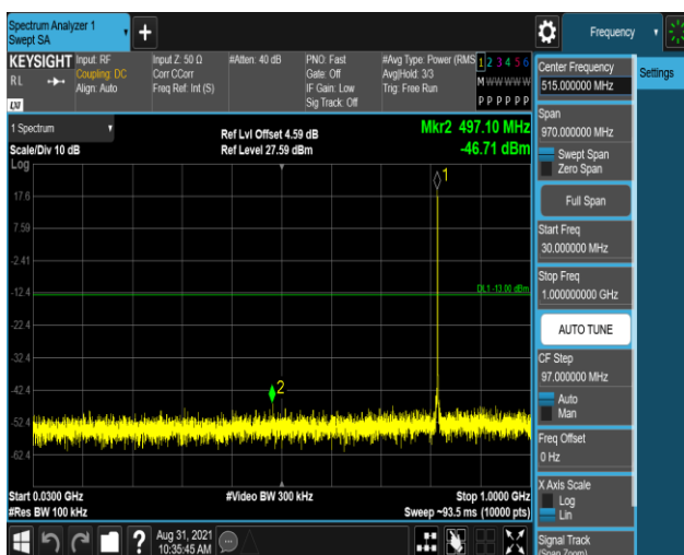
Band26-1.4MHz-QPSK-26740-1RB#0-Range1:30~1000MHz
