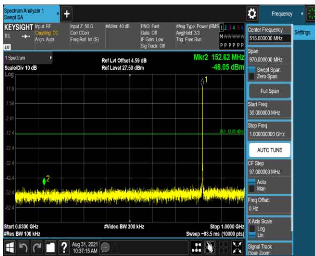
Band26-1.4MHz-16QAM-26797-1RB#0-Range1:30
