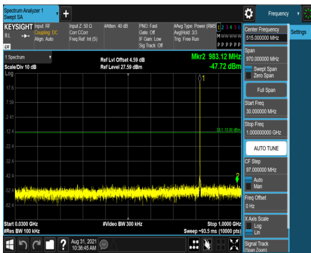
Band26-1.4MHz-QPSK-26797-1RB#0-Range1:30~1000MHz
