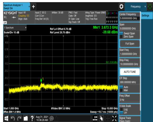
Band26-1.4MHz-16QAM-26740-1RB#0-Range2:1000
