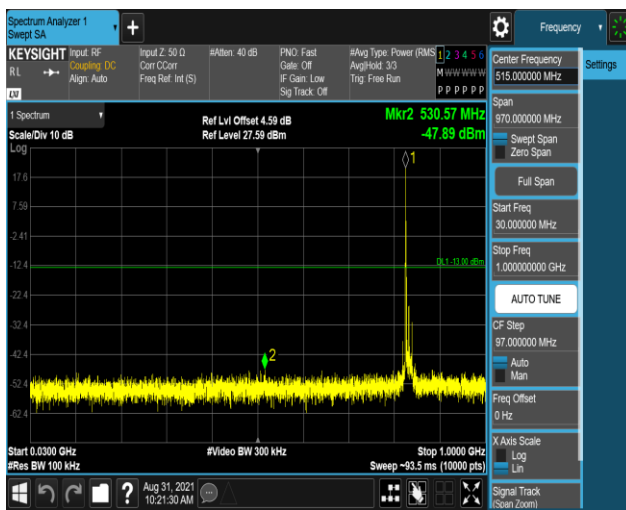
Band26-15MHz-16QAM-26965-1RB#0-Range1:30 ~1000MHz
