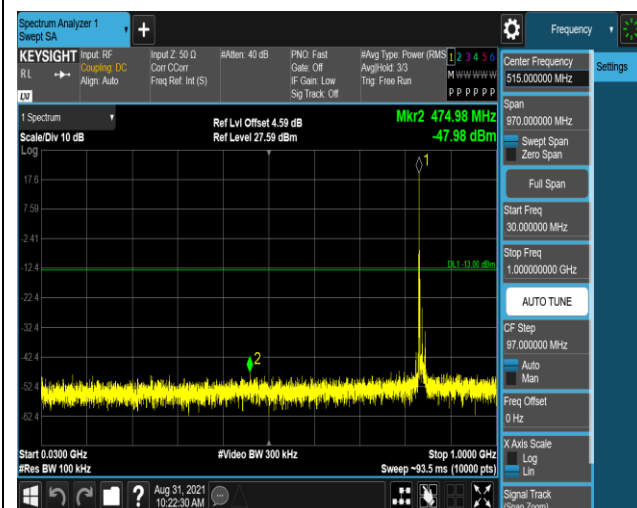
Band26-15MHz-16QAM-26965-1RB#0-Range1:30 ~1000MHz
