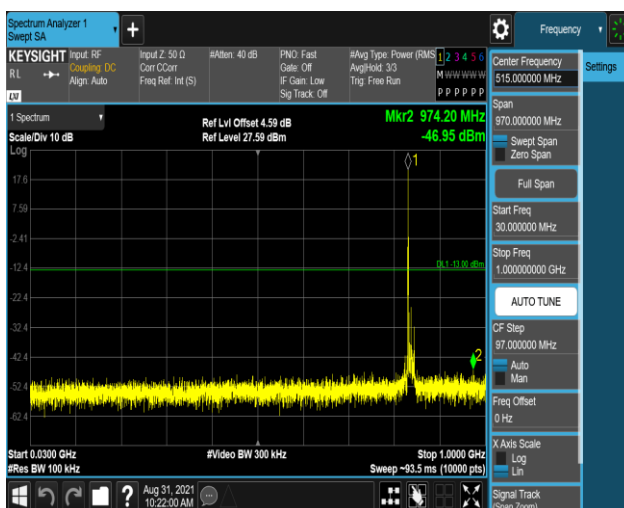
Band26-15MHz-QPSK-26965-1RB#0-Range1:30~1000MHz
