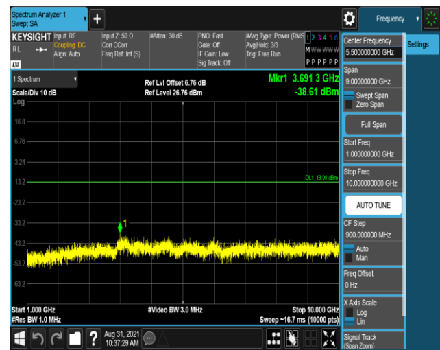
Band26-1.4MHz-16QAM-26797-1RB#0-Range2:1000
