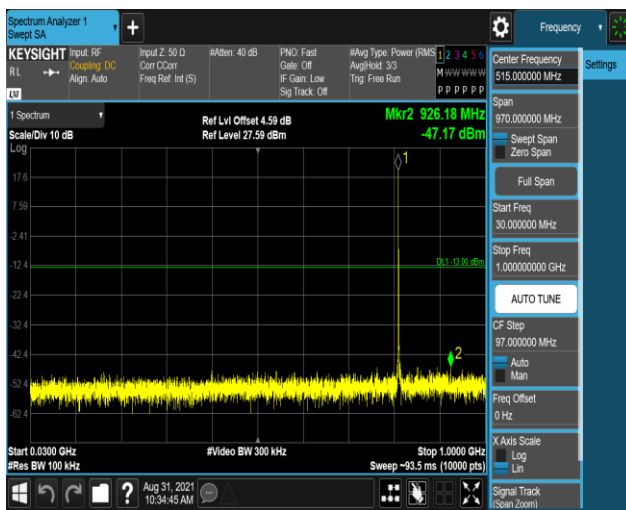
Band26-1.4MHz-QPSK-26740-1RB#0-Range1:30~1000MHz
