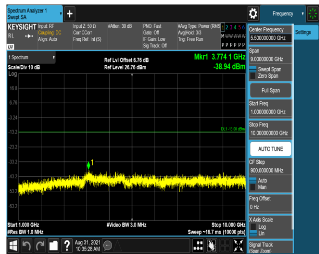
Band26-1.4MHz-16QAM-26740-1RB#0-Range2:1000
