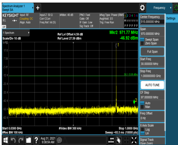
Band26-1.4MHz-16QAM-27033-1RB#0-Range1:30
