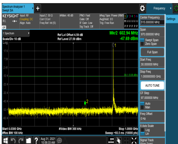
Band26-10MHz-16QAM-26740-1RB#0-Range1:30~1000MHz
