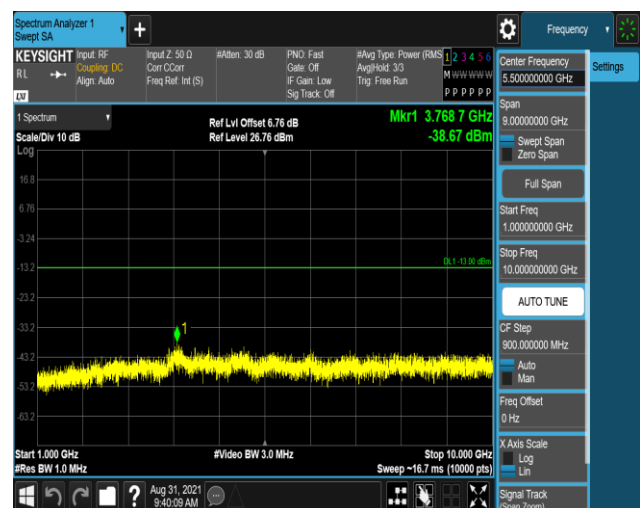
Band26-1.4MHz-16QAM-27033-1RB#0-Range2:1000
