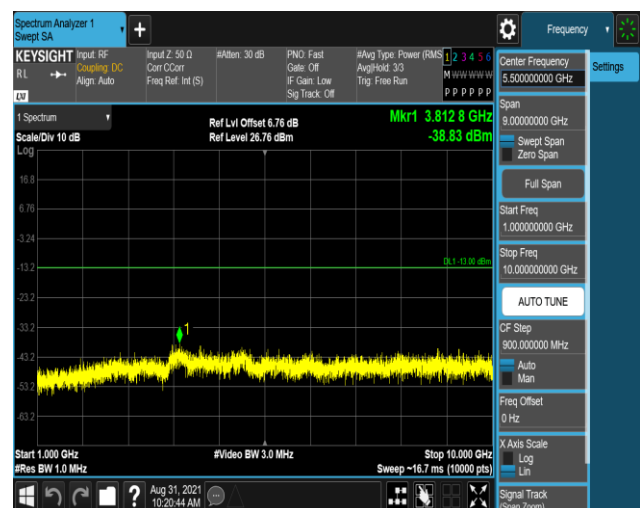
Band26-15MHz-16QAM-26865-1RB#0-Range2:1000~ 10000MHz
