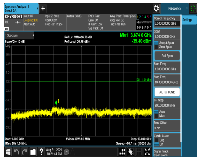
Band26-15MHz-16QAM-26965-1RB#0-Range2:1000~ 10000MHz
