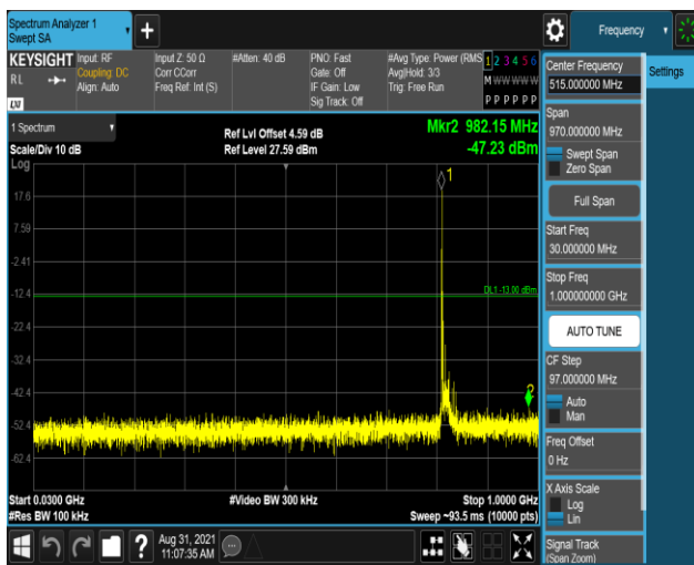
Band26-15MHz-16QAM-26865-1RB#0-Range1:30 ~1000MHz
