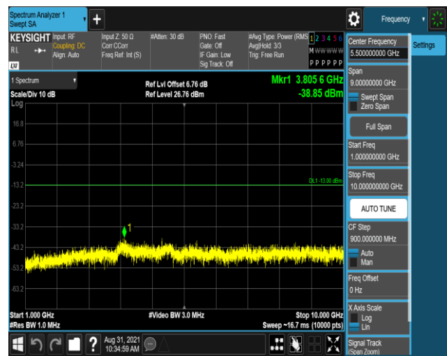
Band26-1.4MHz-QPSK-26740-1RB#0-Range2:1000~10000MHz
