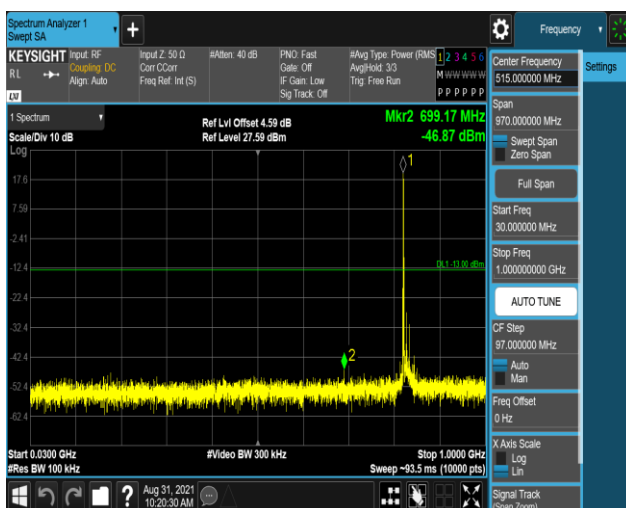
Band26-15MHz-16QAM-26865-1RB#0-Range1:30 ~1000MHz
