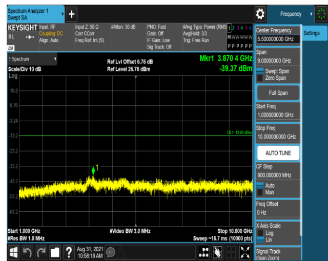
Band26-10MHz-16QAM-26740-1RB#0-Range2:1000~10000MHz
