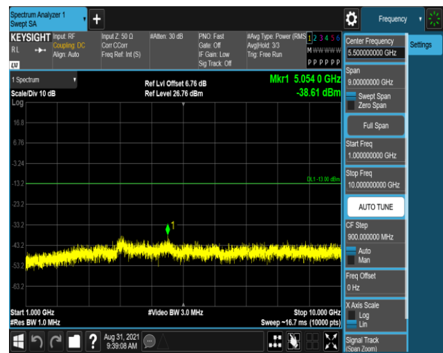
Band26-1.4MHz-16QAM-27033-1RB#0-Range2:1000
