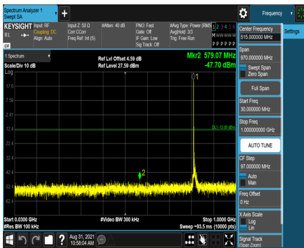
Band26-10MHz-16QAM-26740-1RB#0-Range1:30~1000MHz
