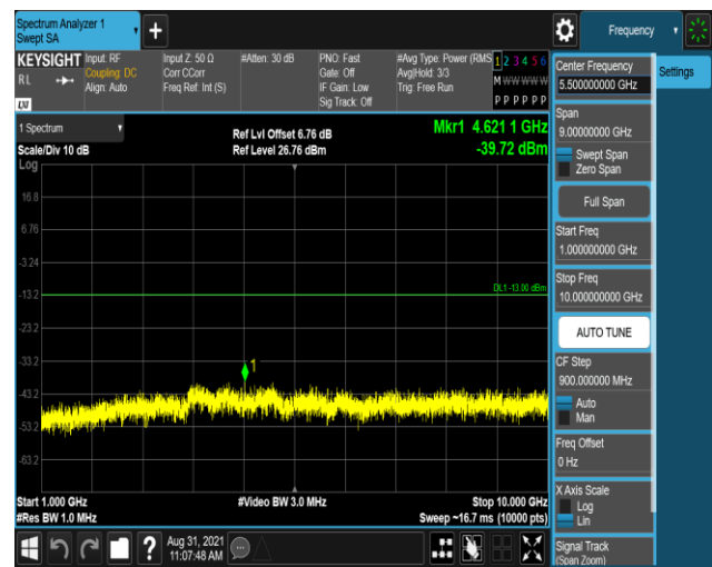
Band26-15MHz-16QAM-26865-1RB#0-Range2:1000~ 10000MHz
