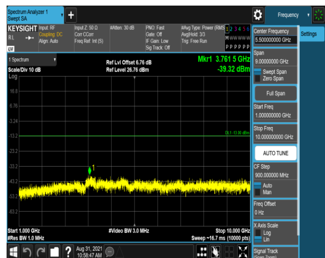
Band26-10MHz-16QAM-26740-1RB#0-Range2:1000~10000MHz
