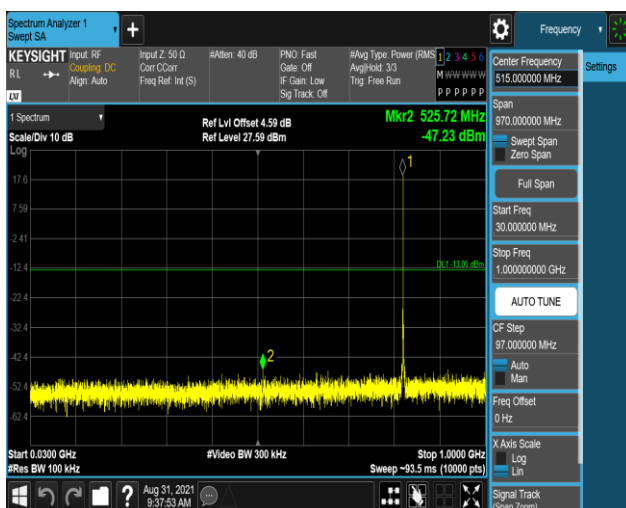
Band26-1.4MHz-16QAM-26797-1RB#0-Range1:30
