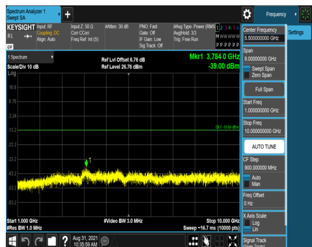
Band26-1.4MHz-QPSK-26740-1RB#0-Range2:1000~10000MHz
