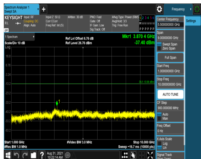
Band26-15MHz-QPSK-26965-1RB#0-Range2:1000~10000MHz
