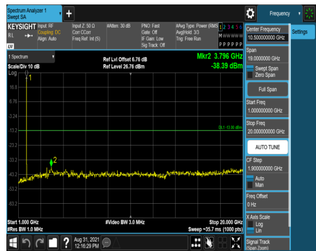
Band66-1.4MHz-QPSK-132322-1RB#0-Range2:1000 ~20000MHz
