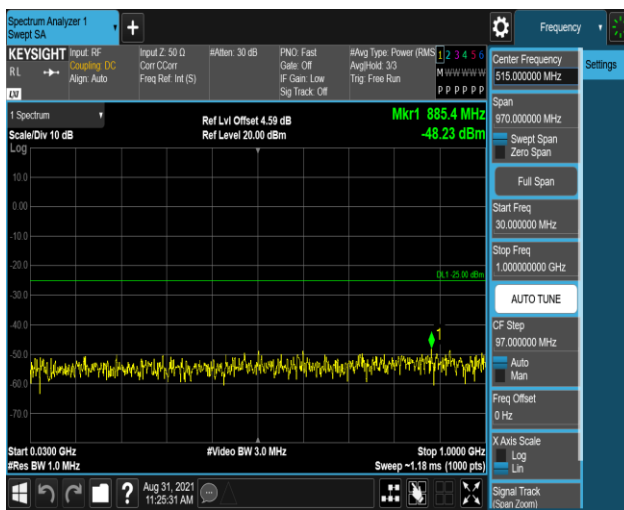
Band41-5MHz-16QAM-41215-1RB#0-Range1:30~1000MHz
