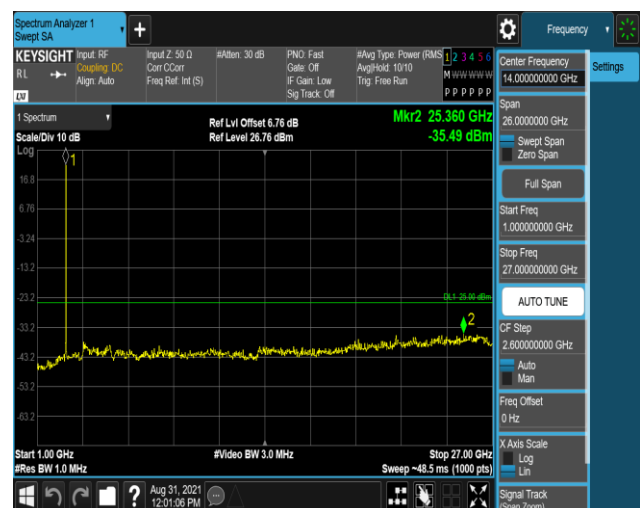
Band41-20MHz-16QAM-41140-1RB#0-Range2:1000~ 27000MHz
