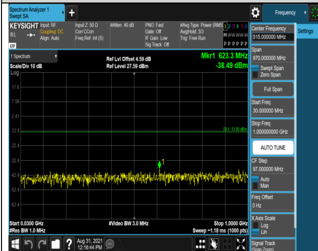
Band66-1.4MHz-16QAM-131979-1RB#0-Range1:3 0~1000MHz
