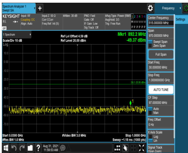
Band41-20MHz-16QAM-41140-1RB#0-Range1:30 ~1000MHz
