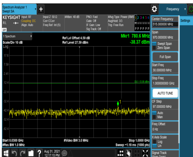
Band66-1.4MHz-QPSK-132322-1RB#0-Range1:30 ~1000MHz
