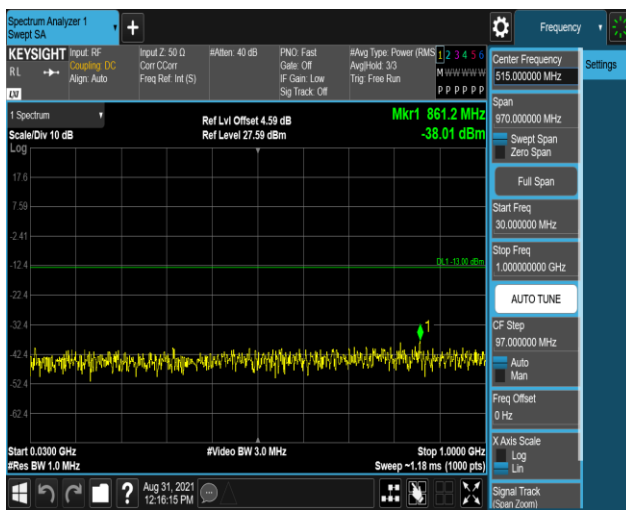
Band66-1.4MHz-QPSK-132322-1RB#0-Range1:30 ~1000MHz
