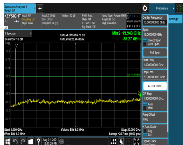
Band66-1.4MHz-QPSK-132322-1RB#0-Range2:1000 ~20000MHz
