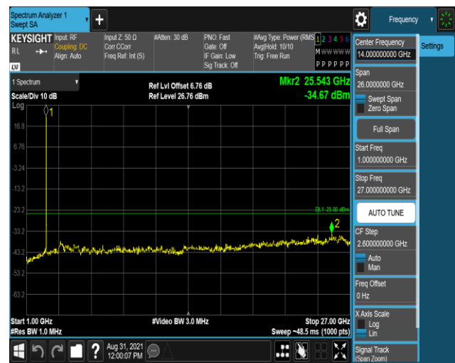
Band41-20MHz-16QAM-41140-1RB#0-Range2:1000~ 27000MHz
