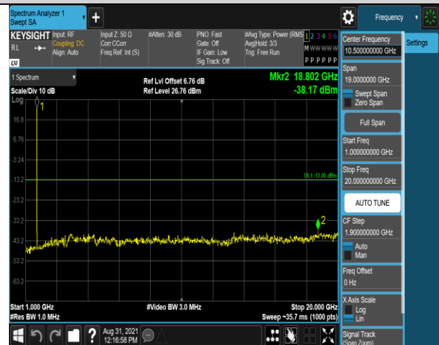
Band66-1.4MHz-16QAM-131979-1RB#0-Range2:100 0~20000MHz
