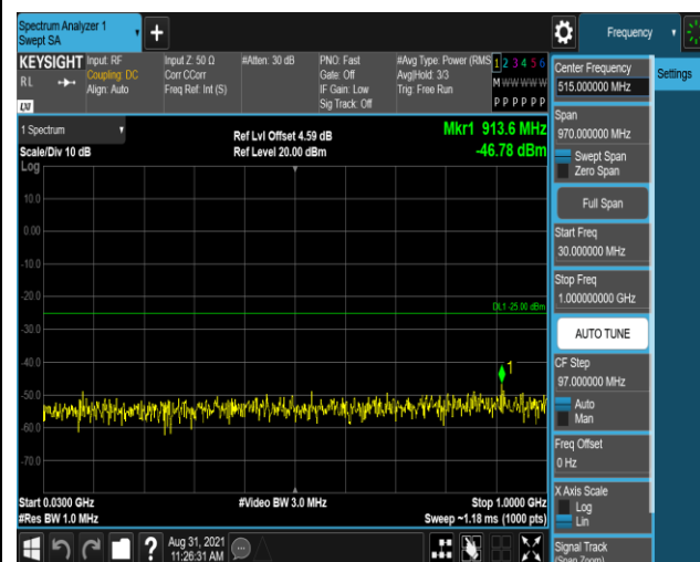
Band41-5MHz-16QAM-41215-1RB#0-Range1:30~1000MHz
