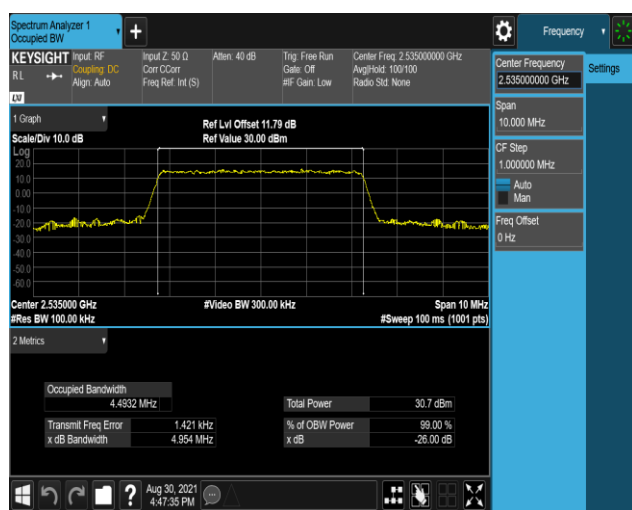
Band7-5MHz-16QAM-21100-25RB#0
