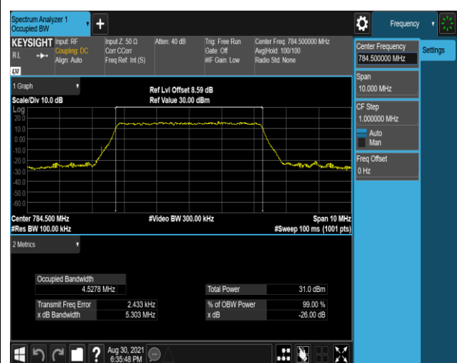
Band13-5MHz-16QAM-23255-25RB#0
