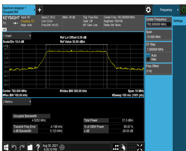
Band13-5MHz-16QAM-23230-25RB#0
