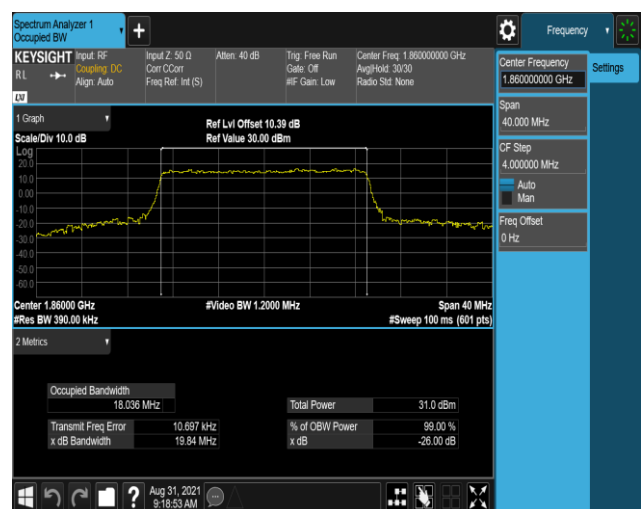
Band25-20MHz-16QAM-26140-100RB#0
