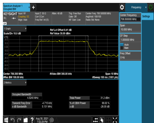
Band17-5MHz-16QAM-23755-25RB#0
