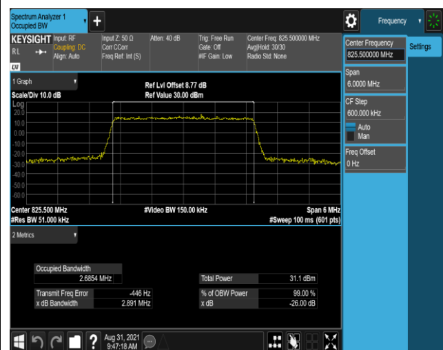
Band26-3MHz-QPSK-26805-15RB#0
