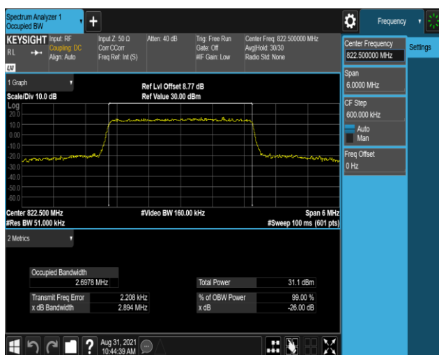
Band26-3MHz-QPSK-26775-15RB#0
