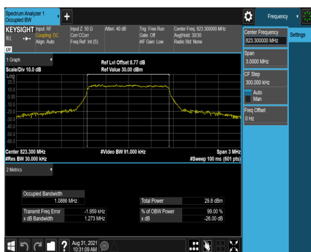
Band26-1.4MHz-16QAM-26783-6RB#0
