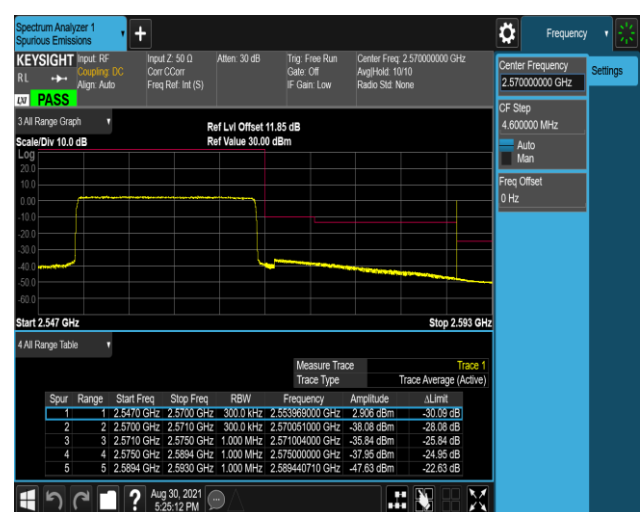
Band7-20MHz-16QAM-21350-100RB#0
