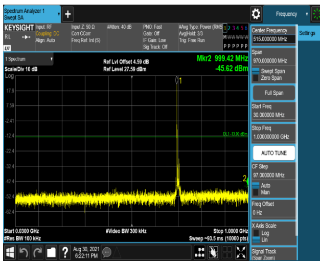
Band12-10MHz-16QAM-23130-1RB#0-Range1:30 ~1000MHz
