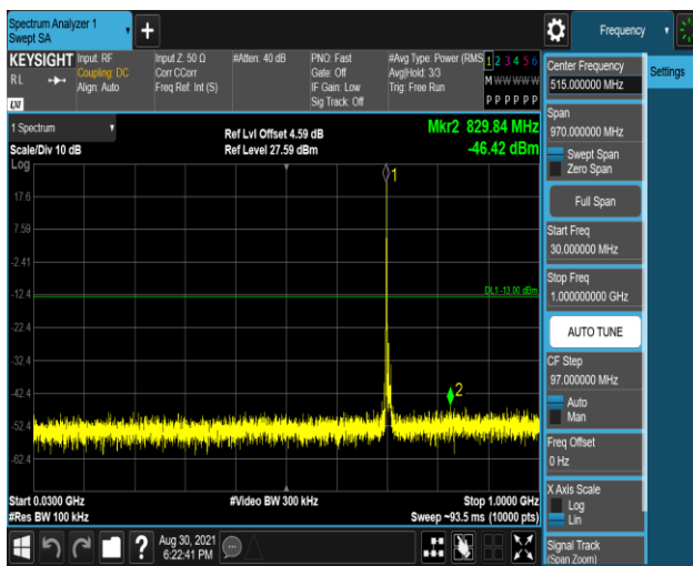
Band12-10MHz-16QAM-23060-1RB#0-Range1:30~1000MHz
