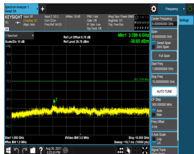
Band12-10MHz-16QAM-23130-1RB#0-Range2:1000~ 10000MHz
