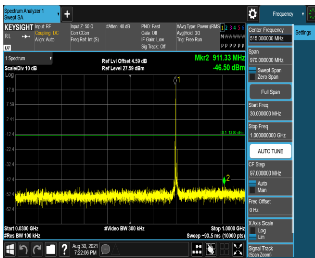
Band17-10MHz-QPSK-23790-1RB#0-Range1:30~1000MHz
