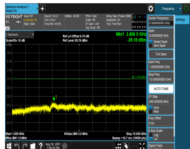
Band17-5MHz-QPSK-23790-1RB#0-Range2:1000~10 000MHz
