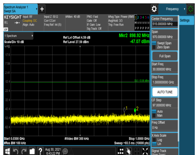
Band13-5MHz-16QAM-23255-1RB#0-Range1:30~1000MHz
