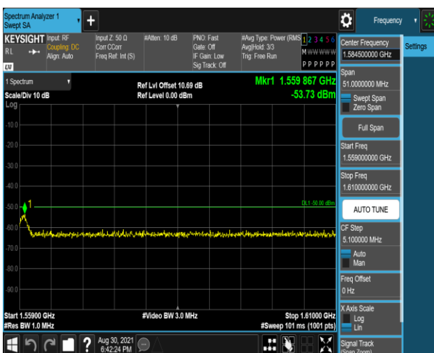
Band13-5MHz-16QAM-23230-1RB#0-Range3:1559~1610MHz
