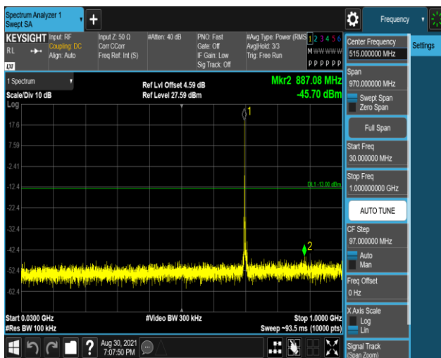
Band17-5MHz-16QAM-23755-1RB#0-Range1:30~ 1000MHz
