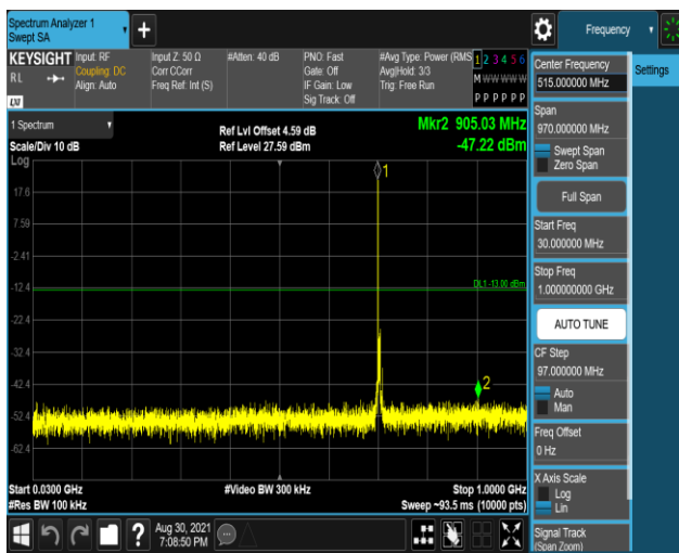
Band17-5MHz-16QAM-23825-1RB#0-Range1:30~1000MHz
