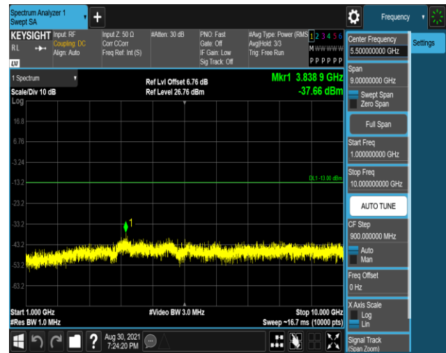
Band17-10MHz-16QAM-23780-1RB#0-Range2:1000~10000MHz
