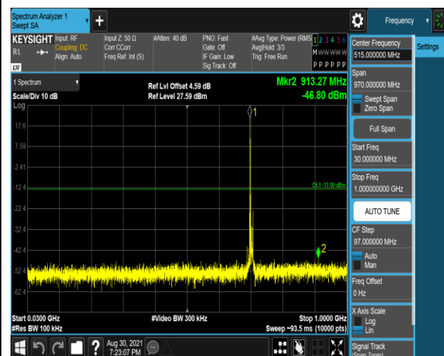
Band17-10MHz-QPSK-23790-1RB#0-Range1:30~1000MHz
