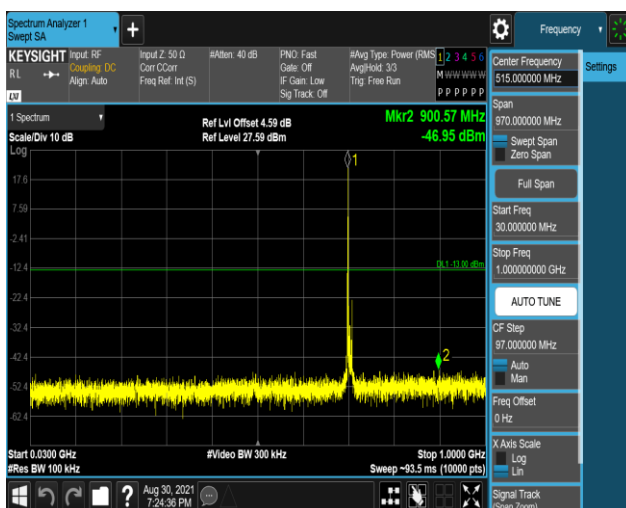
Band17-10MHz-16QAM-23800-1RB#0-Range1:30 ~1000MHz
