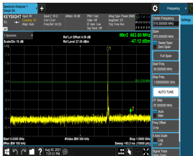
Band17-5MHz-QPSK-23790-1RB#0-Range1:30~1 000MHz
