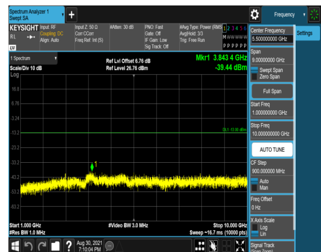
Band17-5MHz-16QAM-23825-1RB#0-Range2:1000~10000MHz
