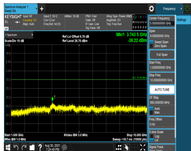
Band17-10MHz-16QAM-23800-1RB#0-Range2:1000~ 10000MHz
