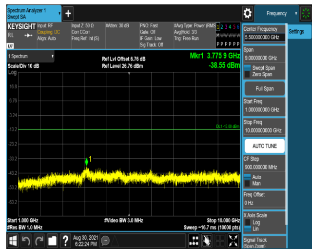
Band12-10MHz-16QAM-23130-1RB#0-Range2:1000~ 10000MHz
