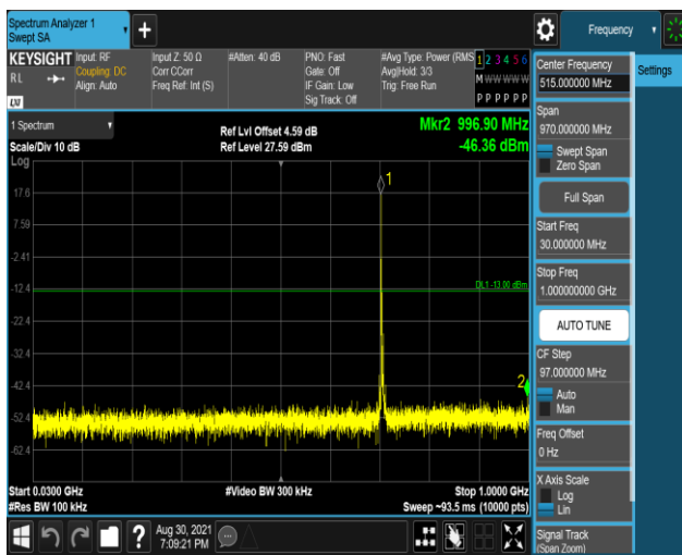
Band17-5MHz-16QAM-23755-1RB#0-Range1:30~ 1000MHz
