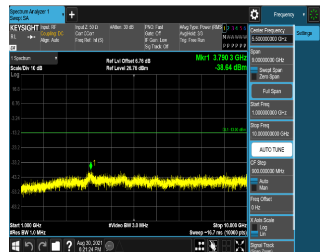
Band12-10MHz-16QAM-23060-1RB#0-Range2:1000~10000MHz
