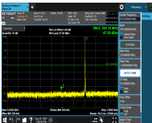
Band17-5MHz-16QAM-23825-1RB#0-Range1:30~1000MHz
