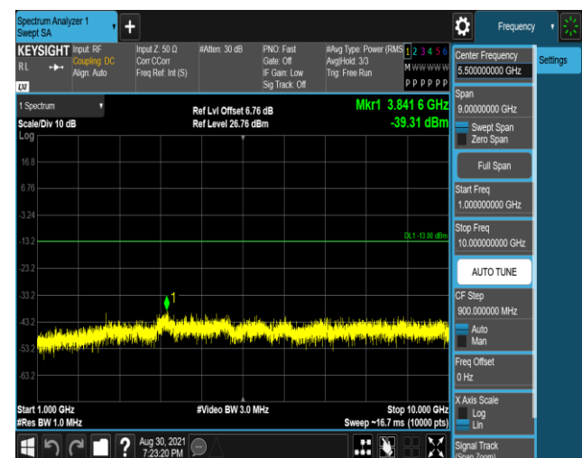
Band17-10MHz-QPSK-23790-1RB#0-Range2:1000~10000MHz
