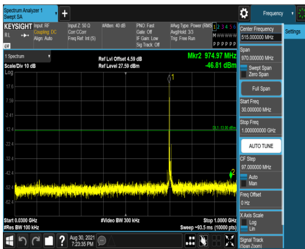
Band17-10MHz-16QAM-23800-1RB#0-Range1:30 ~1000MHz
