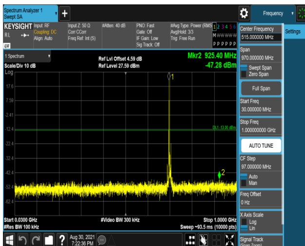
Band17-10MHz-16QAM-23780-1RB#0-Range1:30~1000MHz
