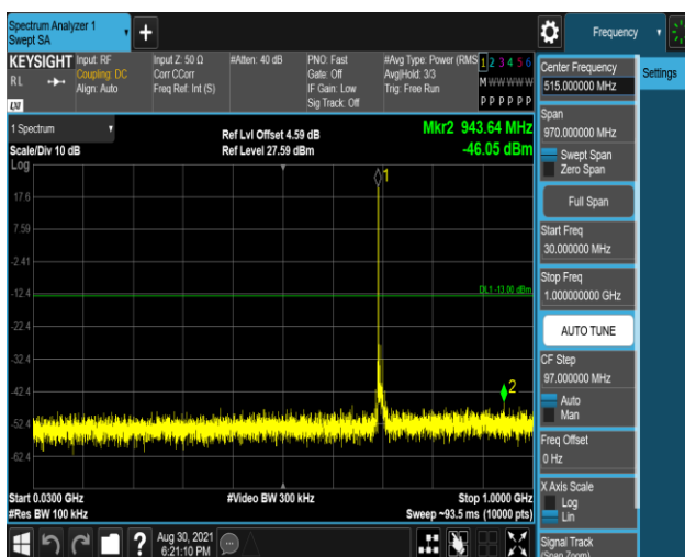
Band12-10MHz-16QAM-23060-1RB#0-Range1:30~1000MHz
