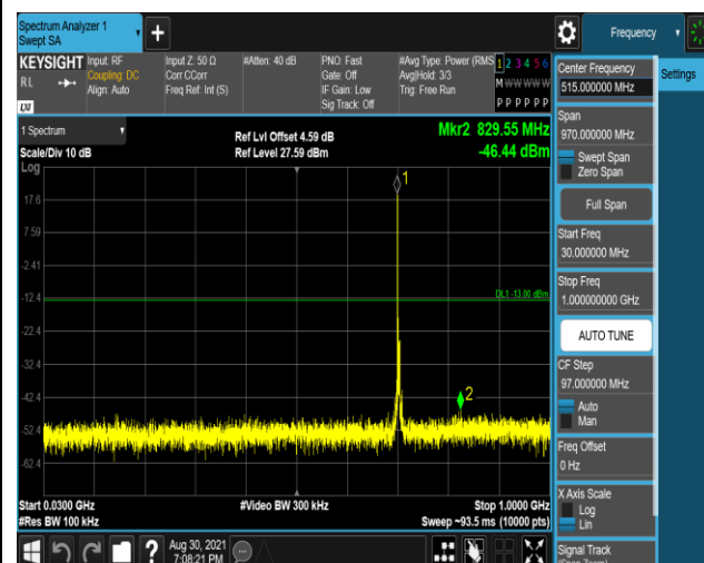
Band17-5MHz-QPSK-23790-1RB#0-Range1:30~1 000MHz
