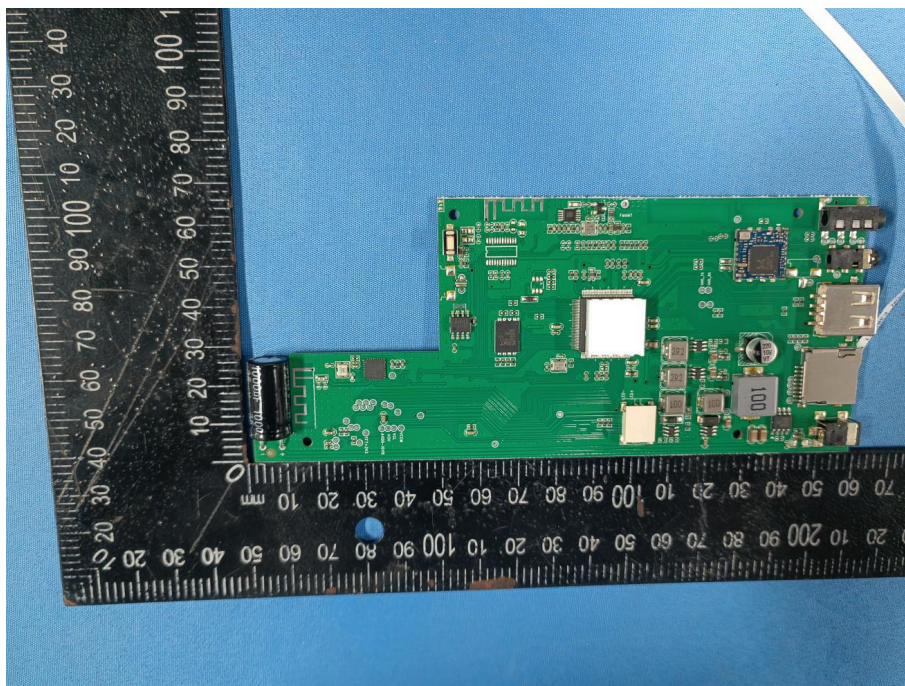
PCB antenna(WIFI)
