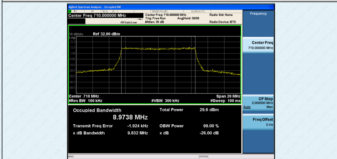
Band17-10MHz-16QAM-23790-50RB#0-8.9738
