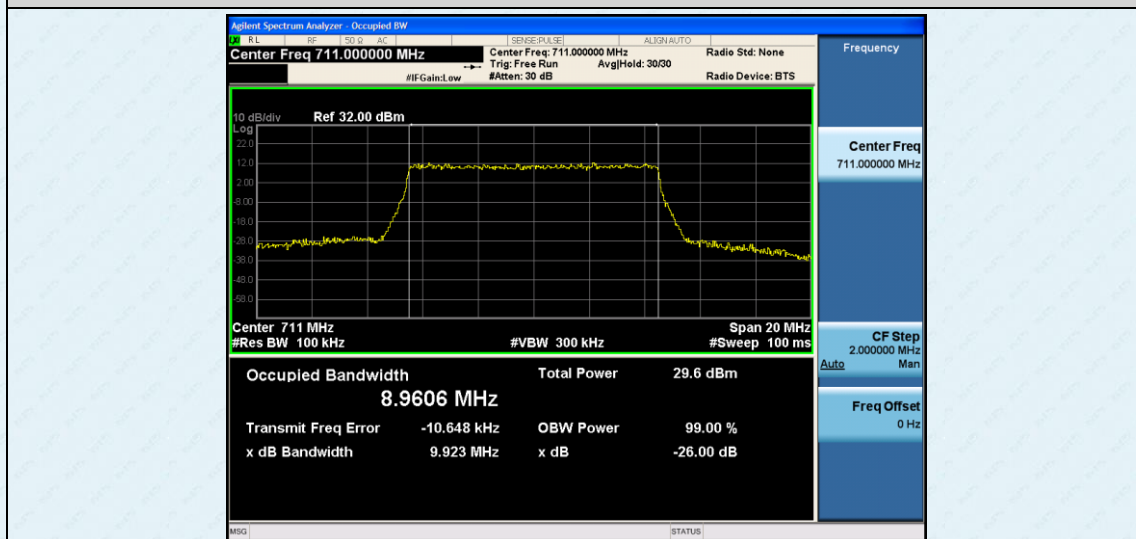
Band17-10MHz-16QAM-23800-50RB#0-8.9606
