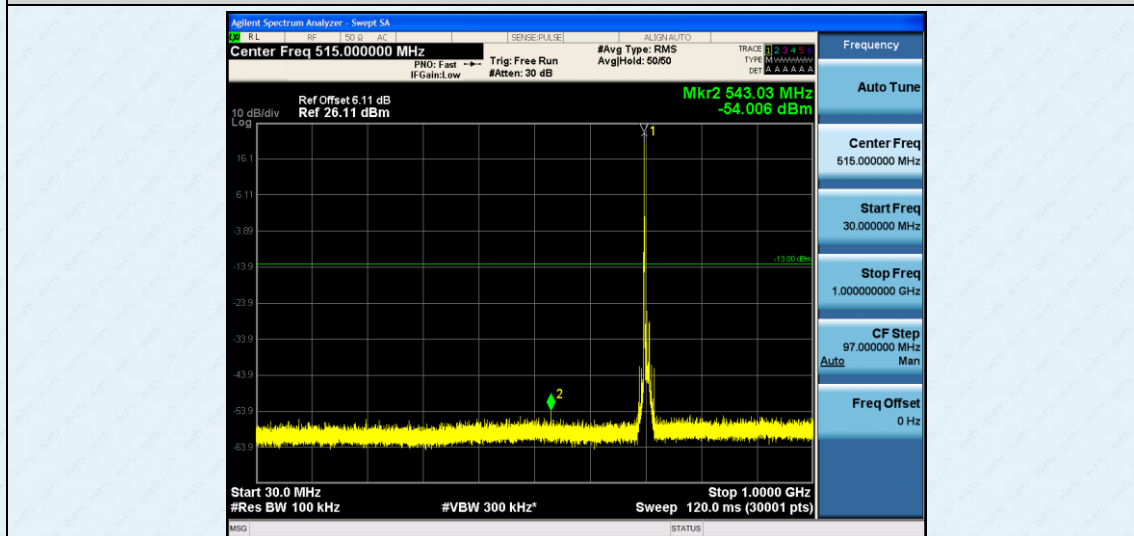
Band17-10MHz-16QAM-23790-1RB#0-30~1000MHz
