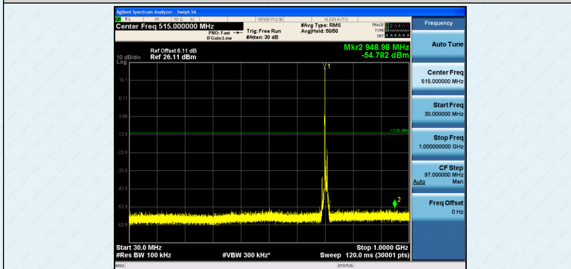
Band17-10MHz-QPSK-23800-1RB#0-30~1000MHz
